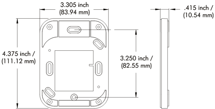
FIGURE 1. Model SWH-3100 Reader Backplate (includes tamper switch magnet)
