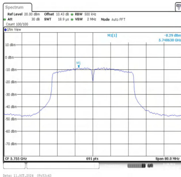
11AC40MIMO-Ant2-5755-PASS
