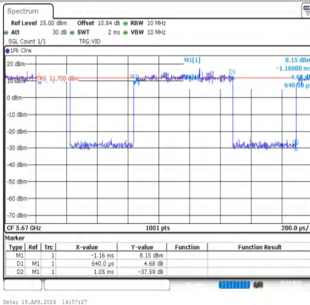
NTNV-11AX40MIMO-Ant1-5670
