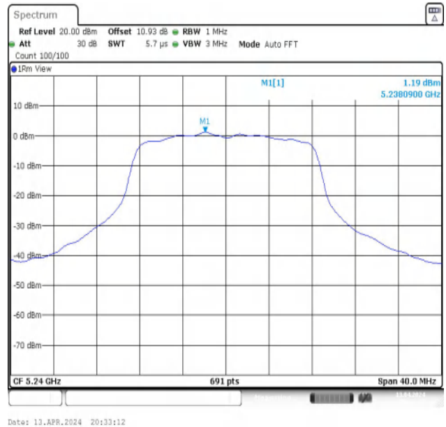
11A-Ant2-5240-PASS
