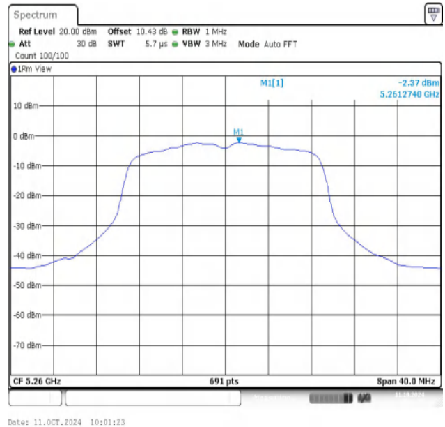
11AC20MIMO-Ant2-5260-PASS
