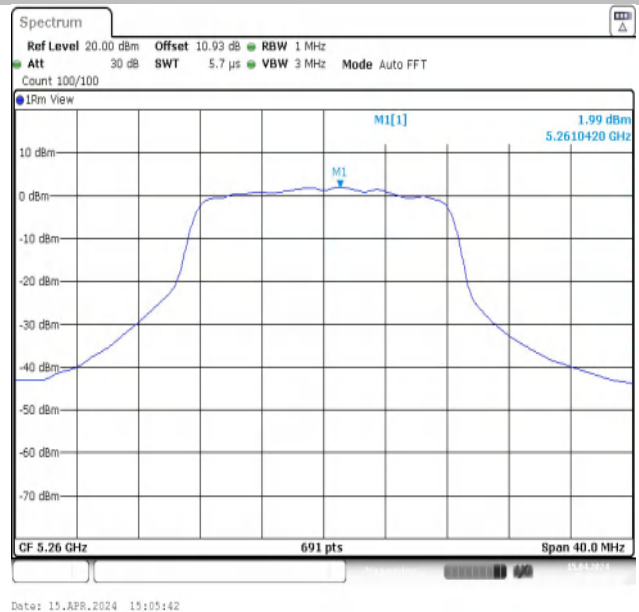
11A-Ant2-5260-PASS
