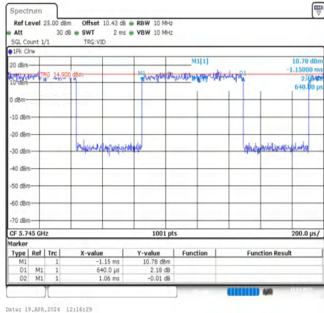
NTNV-11AX20MIMO-Ant2-5745
