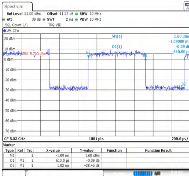
NTNV-11AX80MIMO-Ant1-5530
