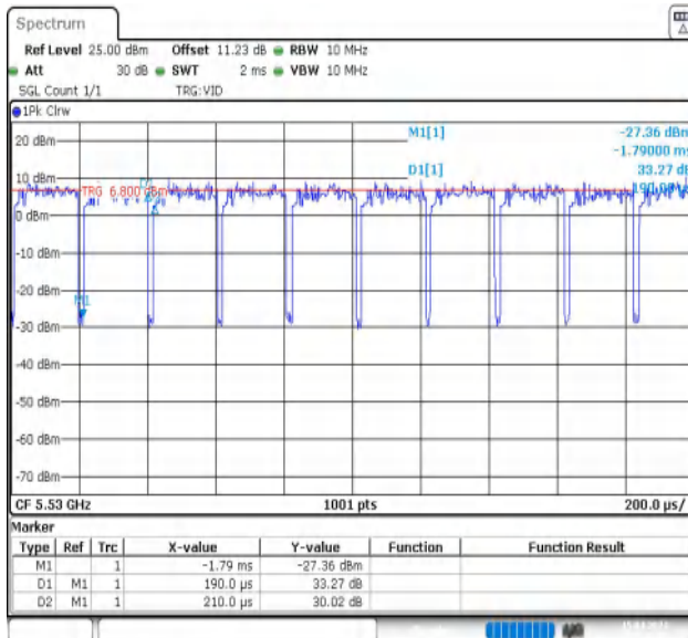
NTNV-11AC80MIMO-Ant1-5530
