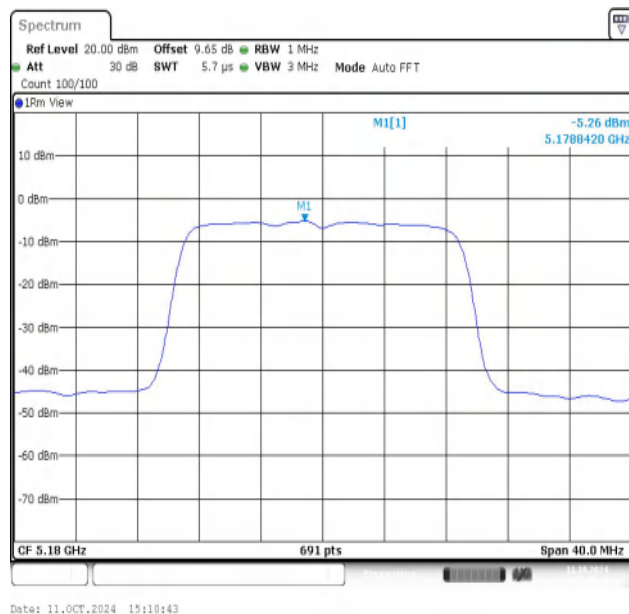
11N20MIMO-Ant2-5180-PASS
