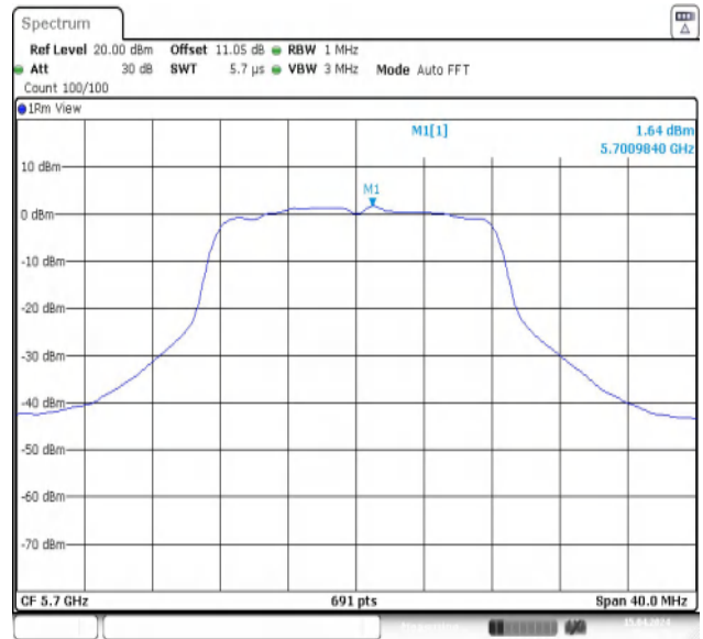
11A-Ant2-5700-PASS
