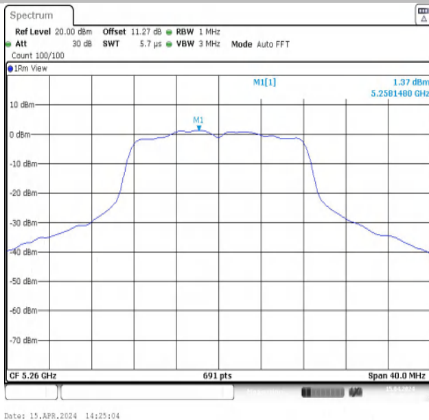
11A-Ant1-5260-PASS
