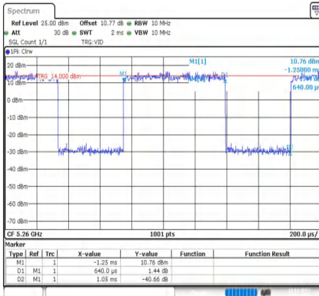
NTVN-11AX20MIMO-Ant1-5260
