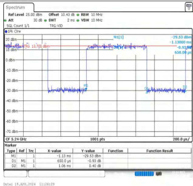
NTNV-11AX20MIMO-Ant2-5240
