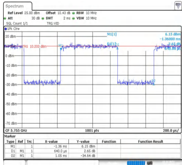
NTVN-11AX40MIMO-Ant2-5755
