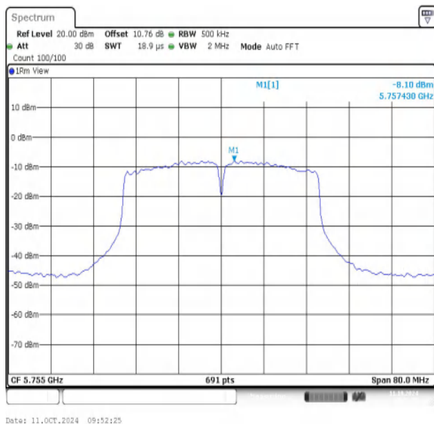
11AC40MIMO-Ant1-5755-PASS
