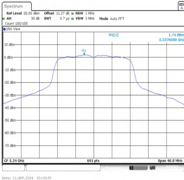
11A-Ant1-5240-PASS
