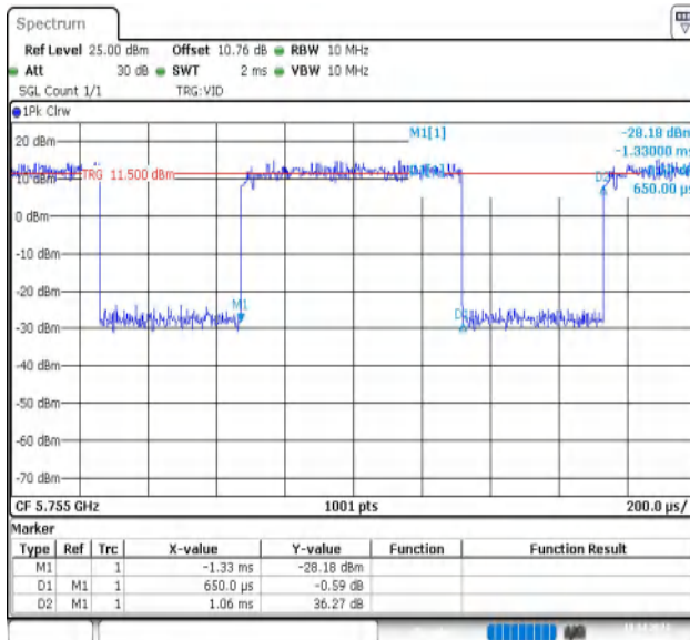
NTVN-11AX40MIMO-Ant1-5755
