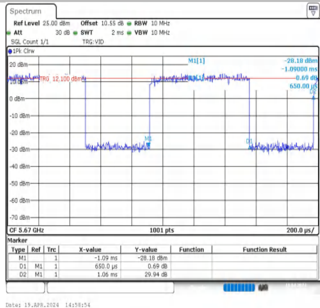
NTNV-11AX40MIMO-Ant2-5670
