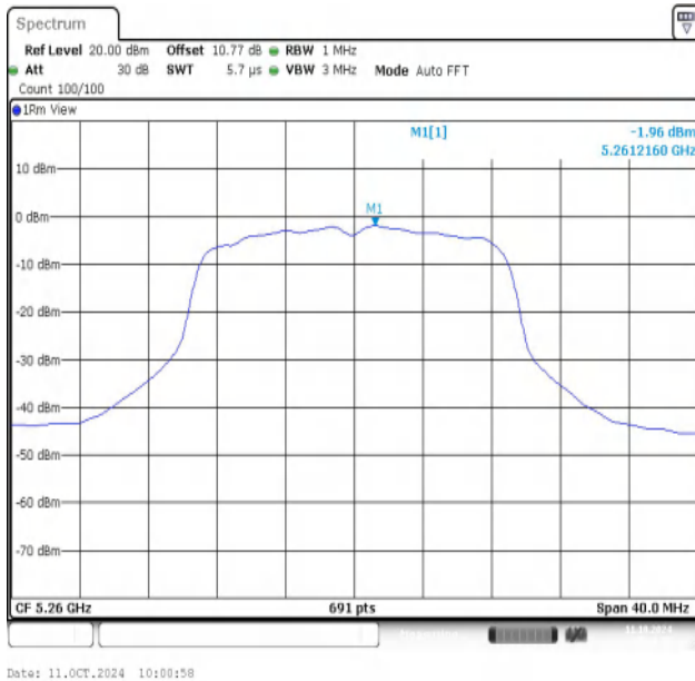
11AC20MIMO-Ant1-5260-PASS
