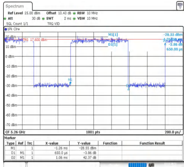
NTVN-11AX20MIMO-Ant2-5260
