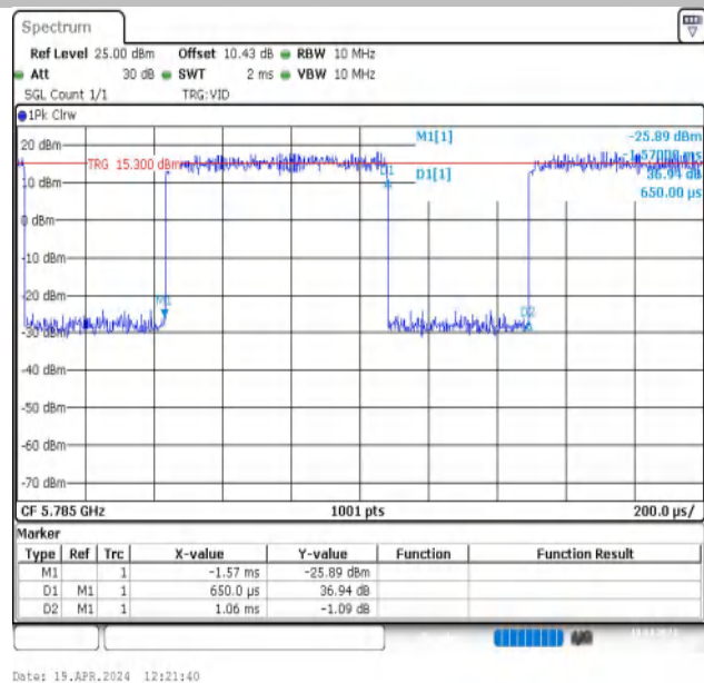
NTNV-11AX20MIMO-Ant2-5785
