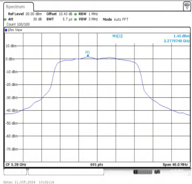
11AC20MIMO-Ant2-5280-PASS
