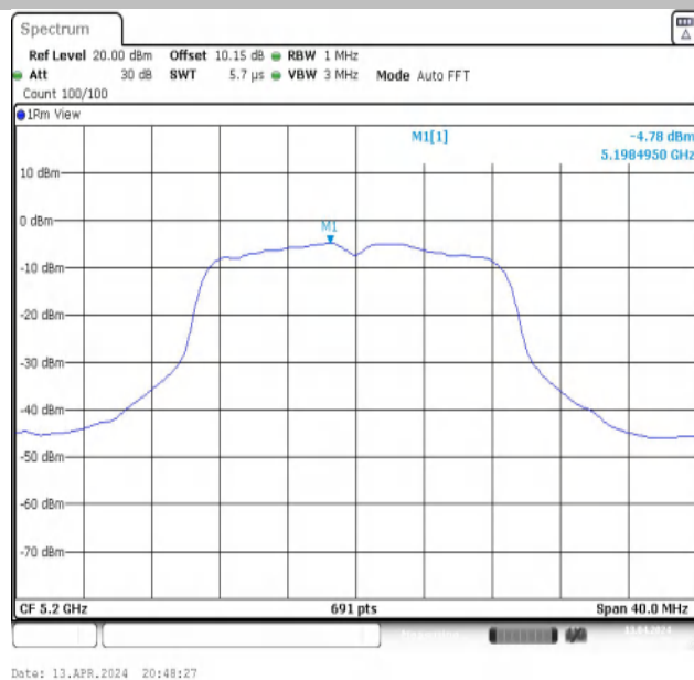
11N20MIMO-Ant2-5200-PASS
