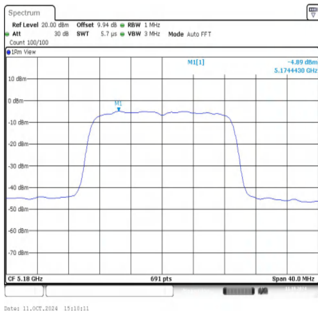
11N20MIMO-Ant1-5180-PASS
