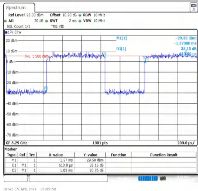
NTNV-11AX80MIMO-Ant2-5290
