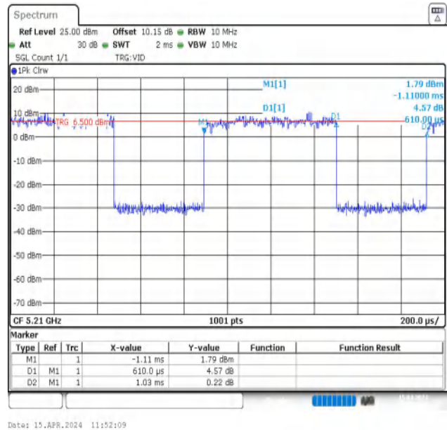
NTNV-11AX80MIMO-Ant2-5210
