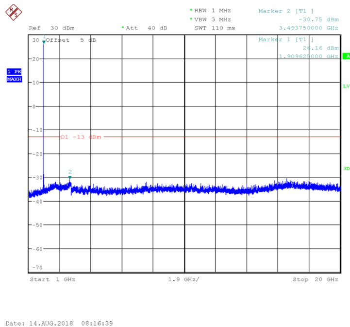
Channel 810: 1GHz~20GHz
