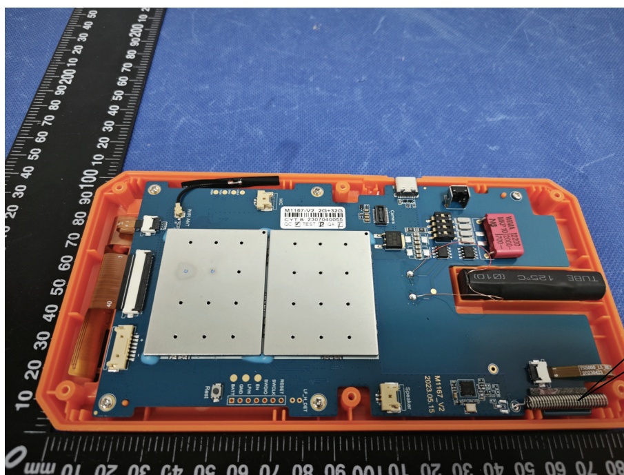
315MHz/433MHz ANT
