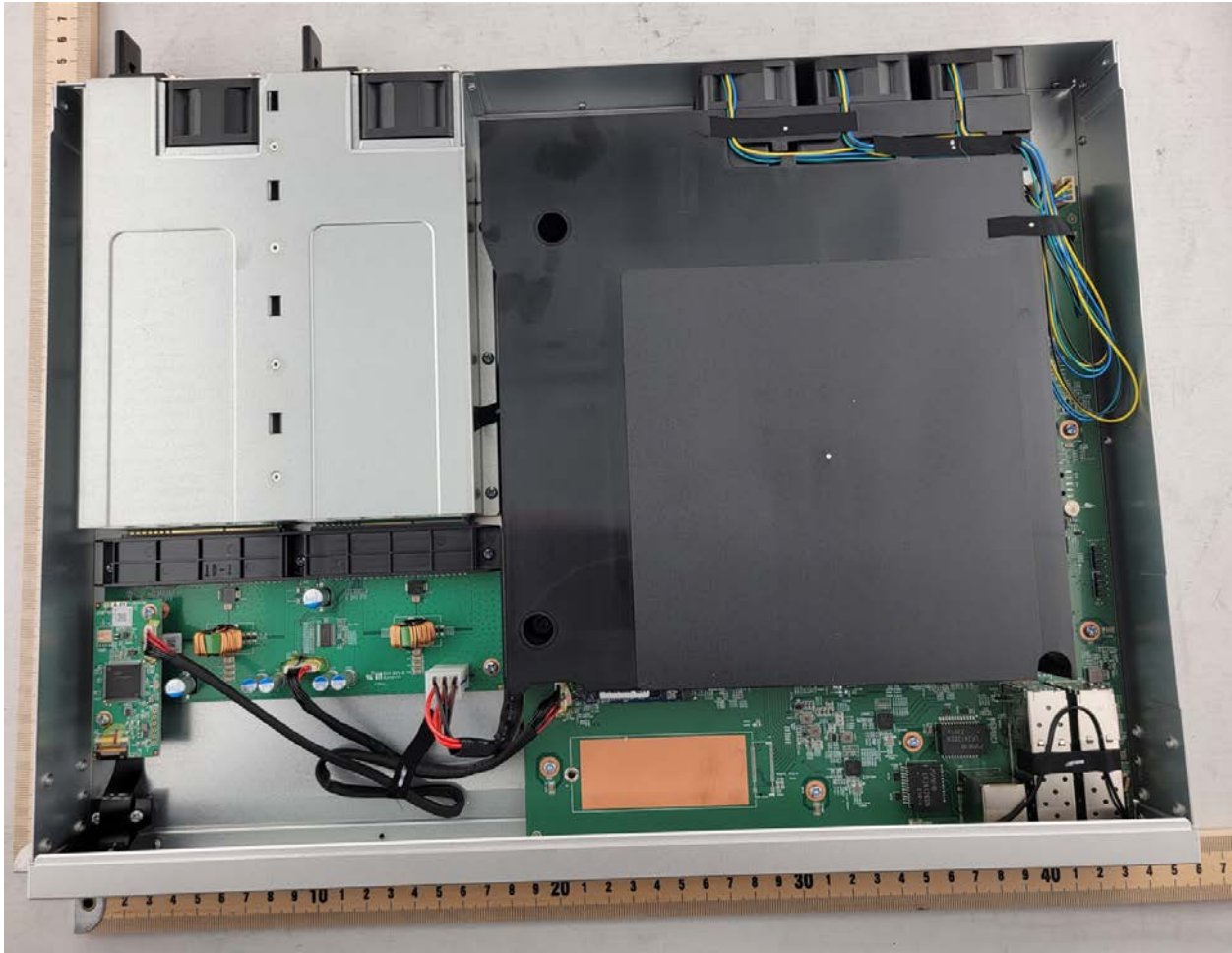
Photograph 1: Internal View of DUT with Top Off
