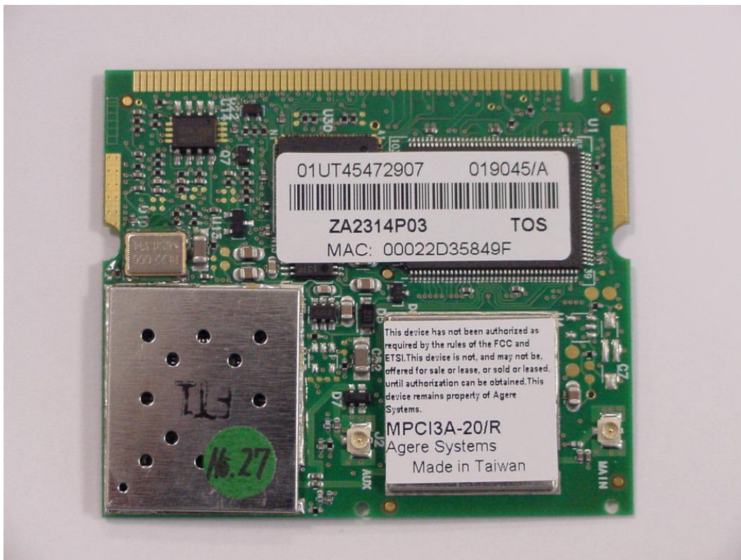
Front Side – with RF shielding
