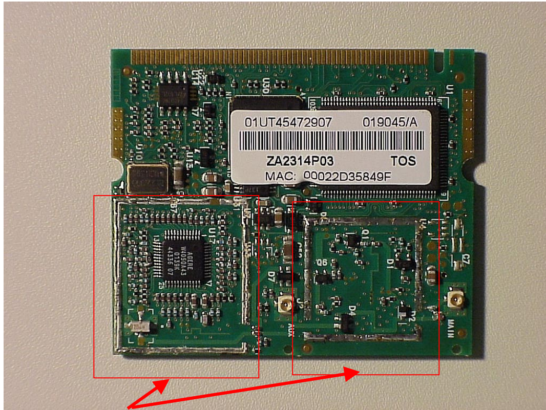
Front Side – without RF shielding
