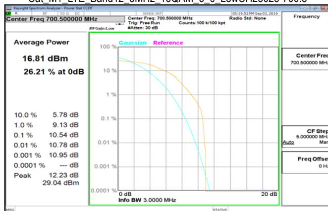
Cat M1 LTE_Band12_3MHz_16QAM_6_0_LowCH23025-700.5
