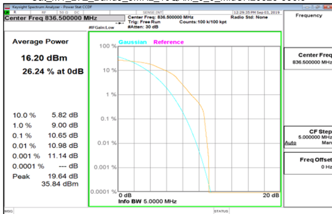
Cat_M1_LTE_Band5_5MHz_16QAM_6_0_MidCH20525-836.5
