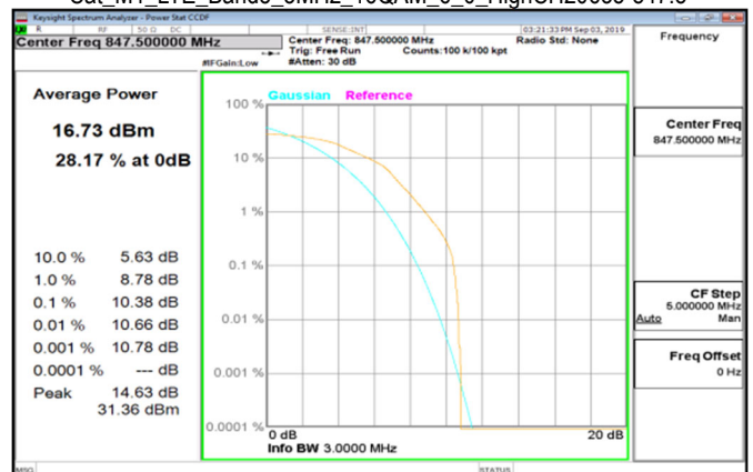
Cat M1 LTE Band5_3MHz_16QAM_6_0_HighCH20635-847.5
