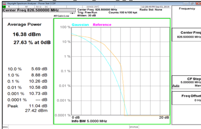
Cat_M1_LTE_Band5_5MHz_16QAM_6_0_LowCH20425-826.5
