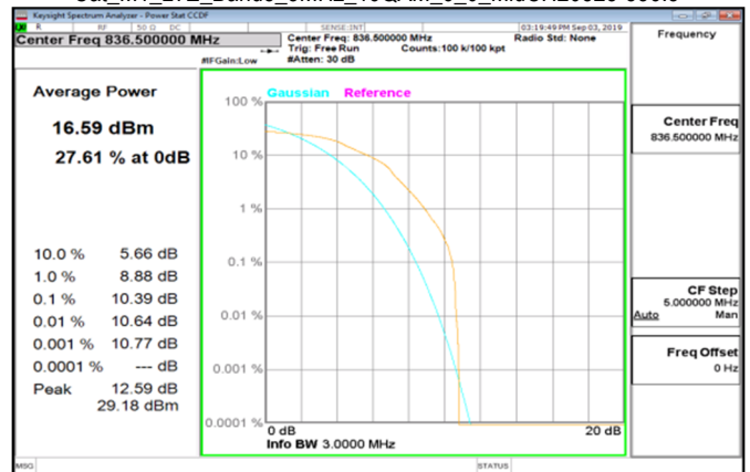
Cat M1 LTE Band5_3MHz_16QAM_6_0_MidCH20525-836.5
