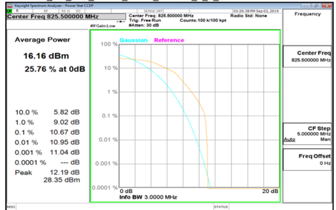
Cat M1 LTE Band5_3MHz_16QAM_6_0_LowCH20415-825.5
