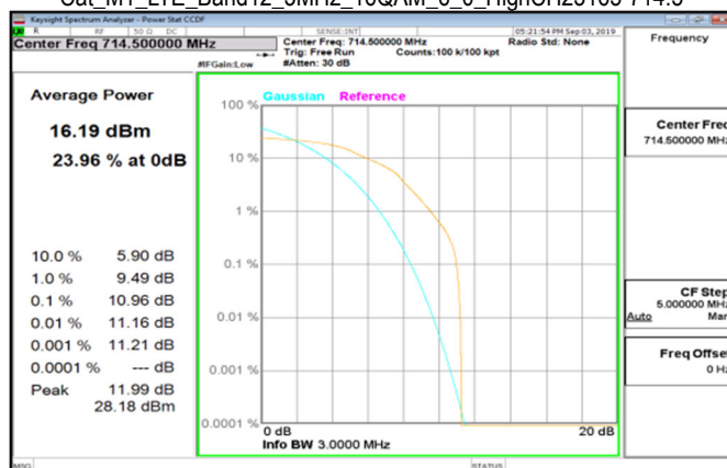
Cat M1 LTE_Band12_3MHz_16QAM_6_0_HighCH23165-714.5
