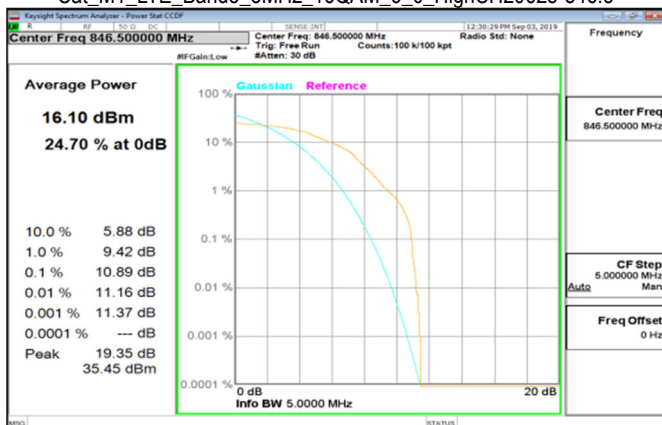
Cat_M1_LTE_Band5_5MHz_16QAM_6_0_HighCH20625-846.5
