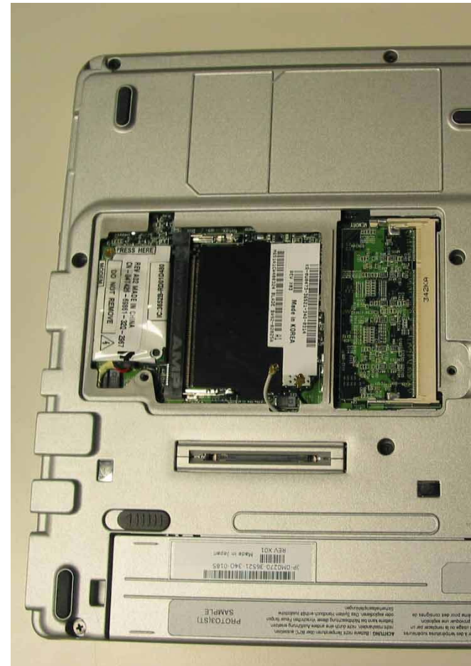
Bottom View showing the MINI PCI expansion slot with (left) and without (right) Wireless LAN Card installed
