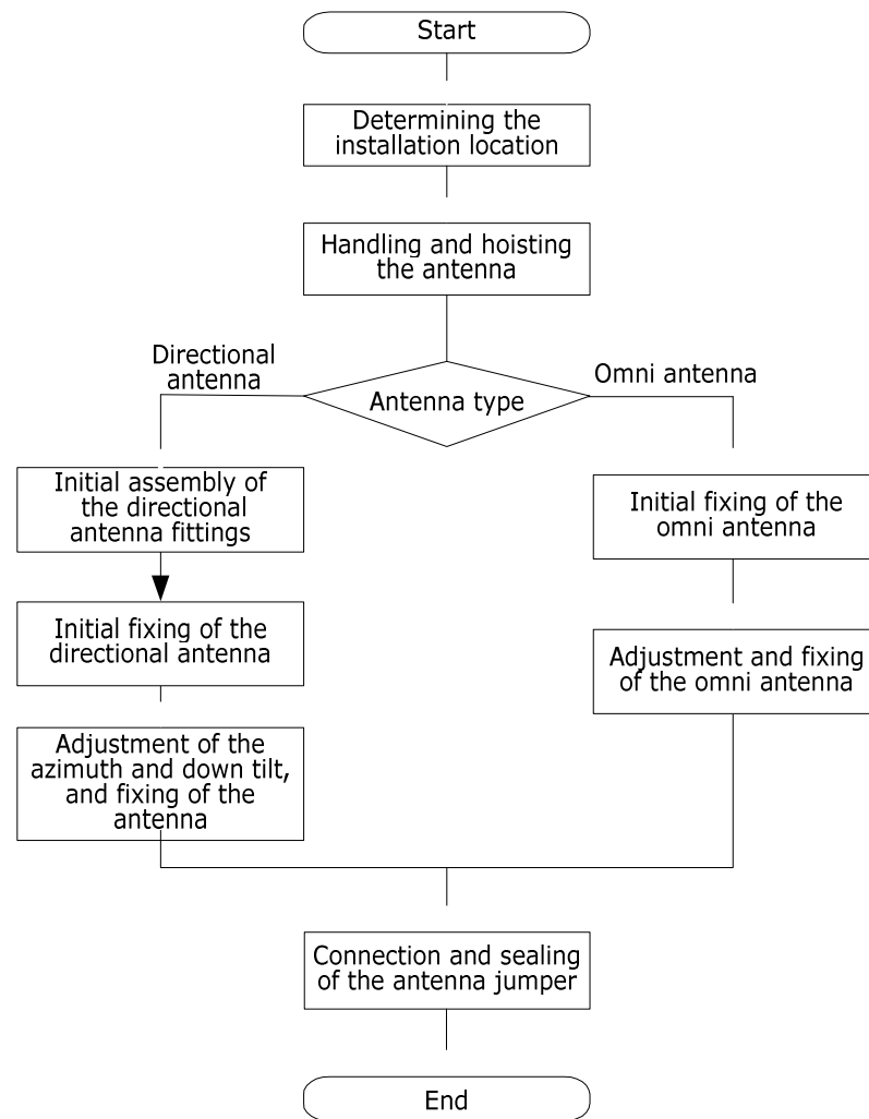
FIGURE 31 ANTENNA INSTALLATION FLOW
