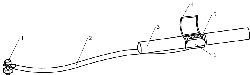
FIGURE 46 THE GROUNDING CLIP STRUCTURE
