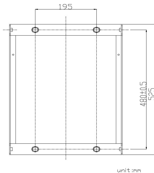
FIGURE 13 SUPPORT HOLES LAYOUT
