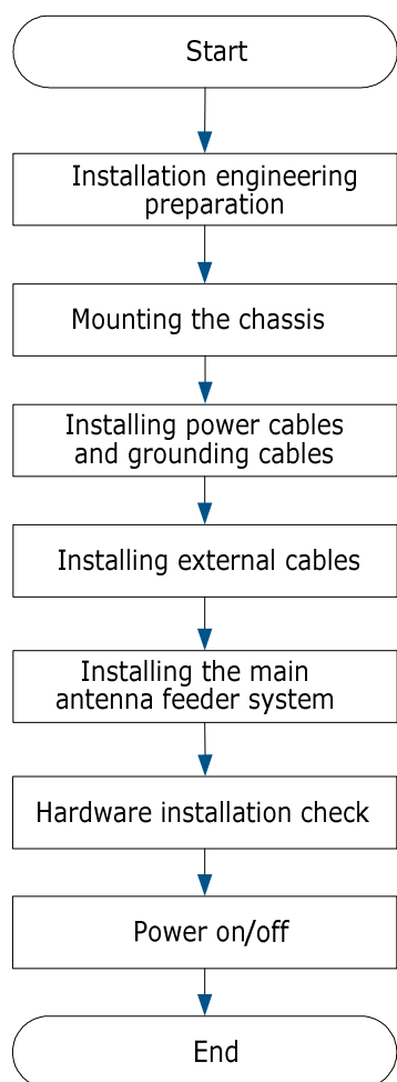
FIGURE 3 RA25 INSTALLATION FLOW
