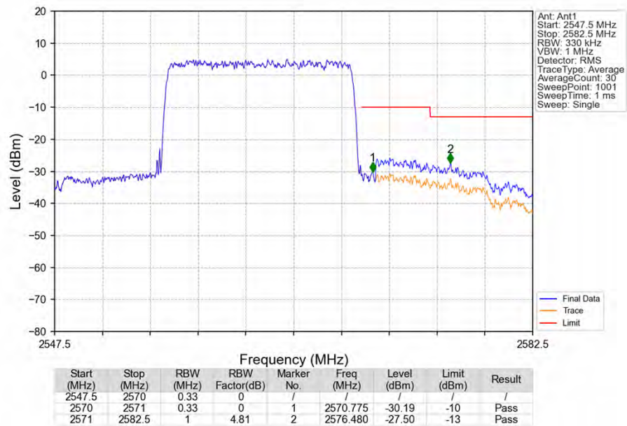
Band7_15MHz_16QAM_HCH_2562.5MHz_RB_75_0_NTNV
