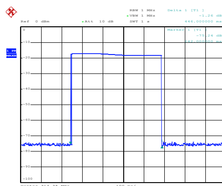
T period
