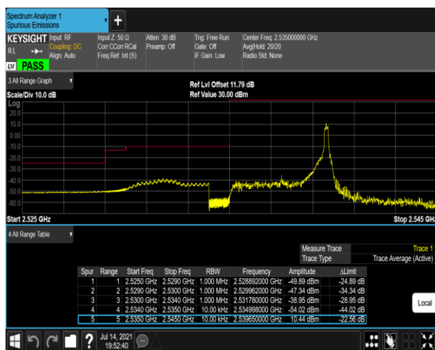
Band41-5MHz-16QAM-40065-1RB#24
