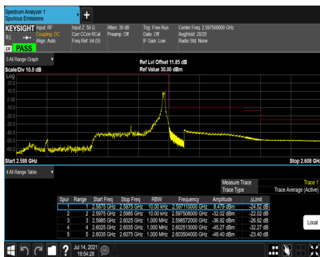
Band41-5MHz-QPSK-40640-1RB#24
