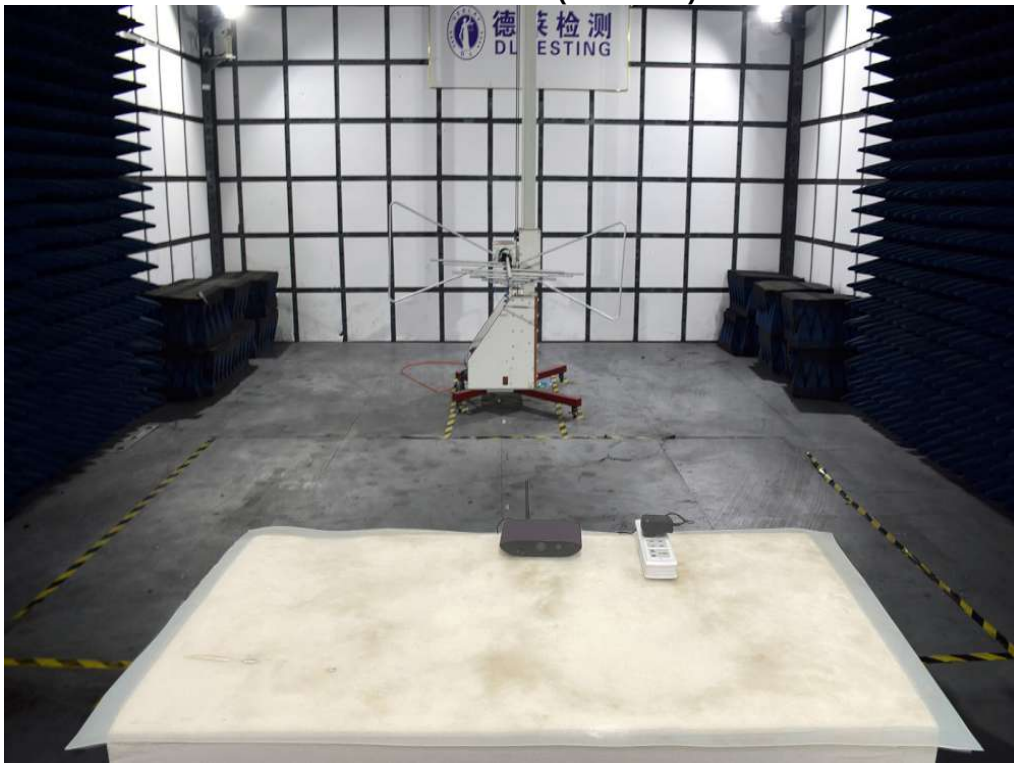
RadiatedEmission(Below 1G)
