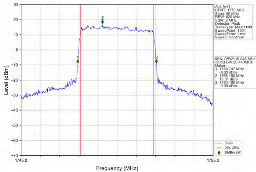
n66_15kHz_SISO_NTNV_20MHz_CP-OFDM_64_QAM_1770MHz_Outer_Full
