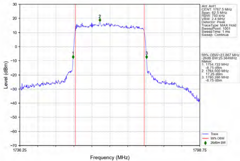
n66_15kHz_SISO_NTNV_25MHz_CP-OFDM_QPSK_1767.5MHz_Outer_Full
