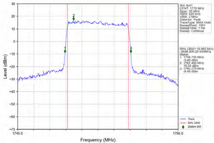
n66_15kHz_SISO_NTNV_20MHz_CP-OFDM_QPSK_1770MHz_Outer_Full
