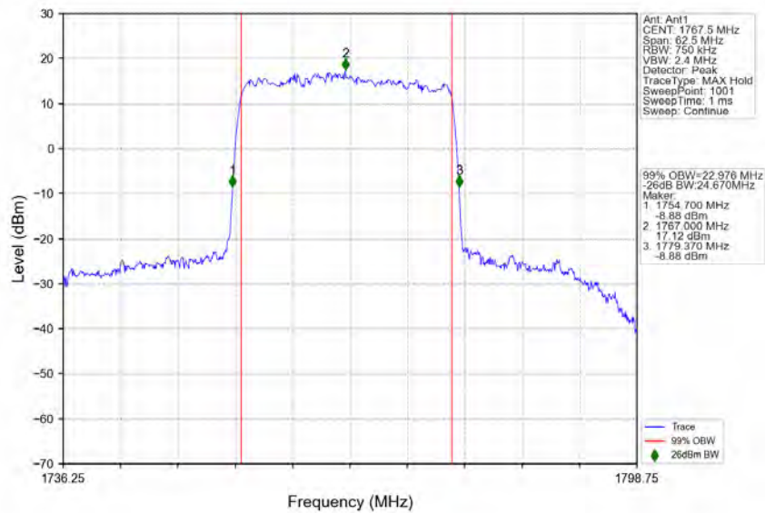
n66_15kHz_SISO_NTNV_25MHz_DFT-s-OFDM_64_QAM_1767.5MHz_Outer_Full
