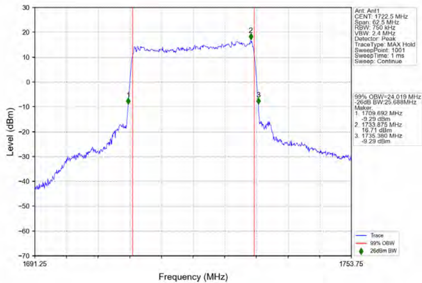
n66_15kHz_SISO_NTNV_25MHz_CP-OFDM_64_QAM_1722.5MHz_Outer_Full
