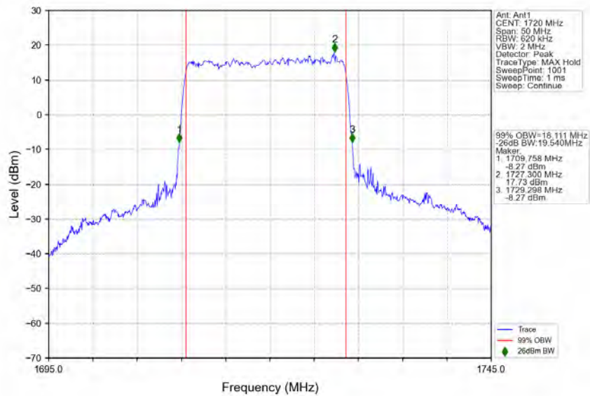
n66_15kHz_SISO_NTNV_20MHz_DFT-s-OFDM_64QAM_1720MHz_Outer_Full
