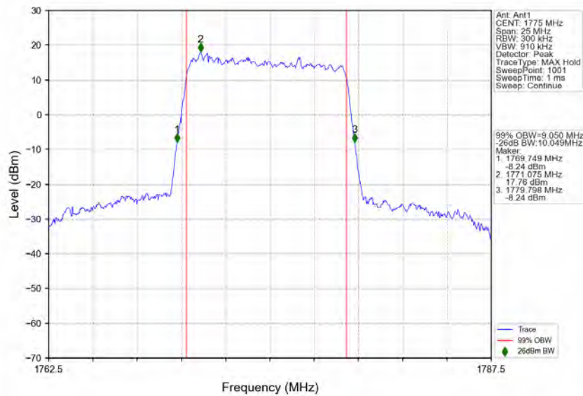
n66_15kHz_SISO_NTNV_10MHz_DFT-s-OFDM_64_QAM_1775MHz_Outer_Full
