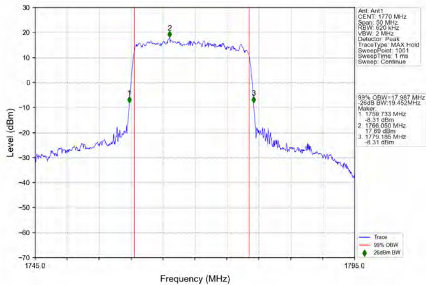
n66_15kHz_SISO_NTNV_20MHz_DFT-s-OFDM_64_QAM_1770MHz_Outer_Full
