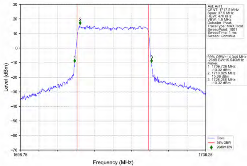
n66_15kHz_SISO_NTNV_15MHz_CP-OFDM 64 QAM 1717.5MHz_Outer_Full
