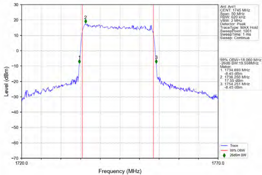
n66_15kHz_SISO_NTNV_20MHz_DFT-s-OFDM_16_QAM_1745MHz_Outer_Full
