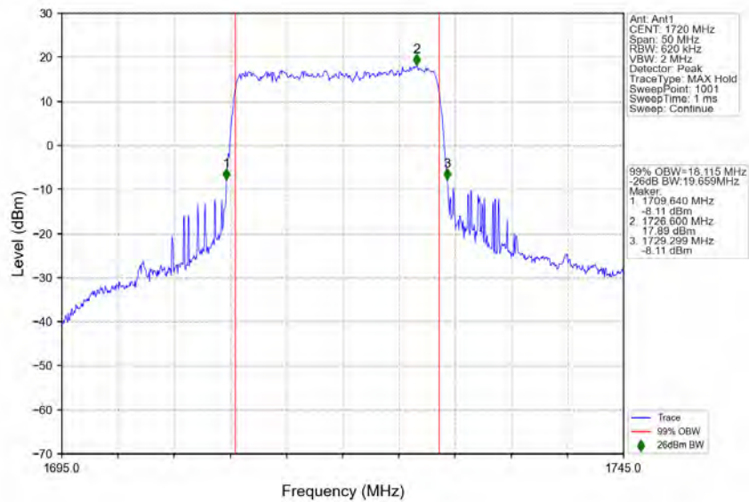
n66_15kHz_SISO_NTNV_20MHz_DFT-s-OFDM QPSK_1720MHz_Outer_Full
