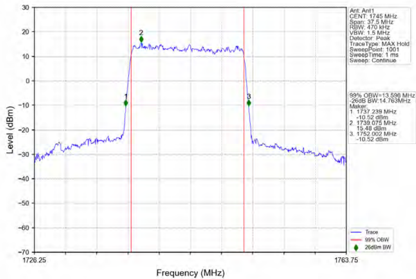
n66_15kHz_SISO_NTNV_15MHz_DFT-s-OFDM_256_QAM_1745MHz_Outer_Full
