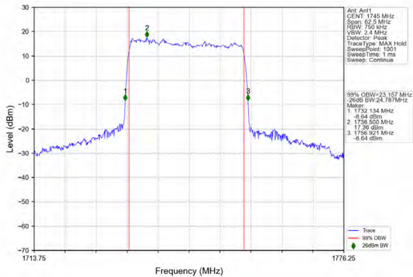
n66_15kHz_SISO_NTNV_25MHz_DFT-s-OFDM_16_QAM_1745MHz_Outer_Full
