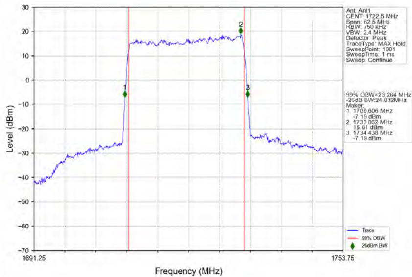
n66_15kHz_SISO_NTNV_25MHz_DFT-s-OFDM QPSK_1722.5MHz_Outer_Full
