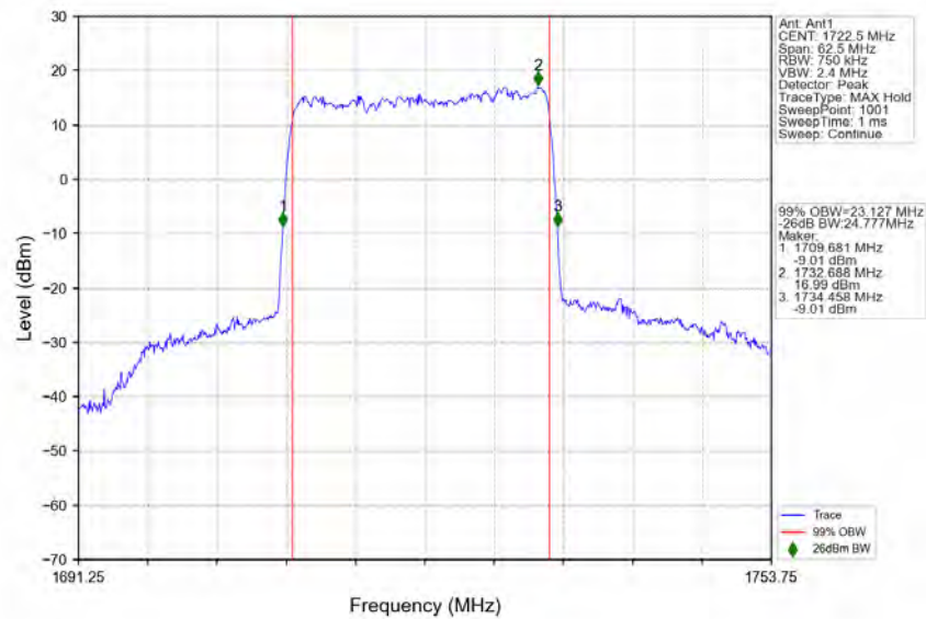
n66_15kHz_SISO_NTNV_25MHz_DFT-s-OFDM_64 QAM_1722.5MHz_Outer_Full
