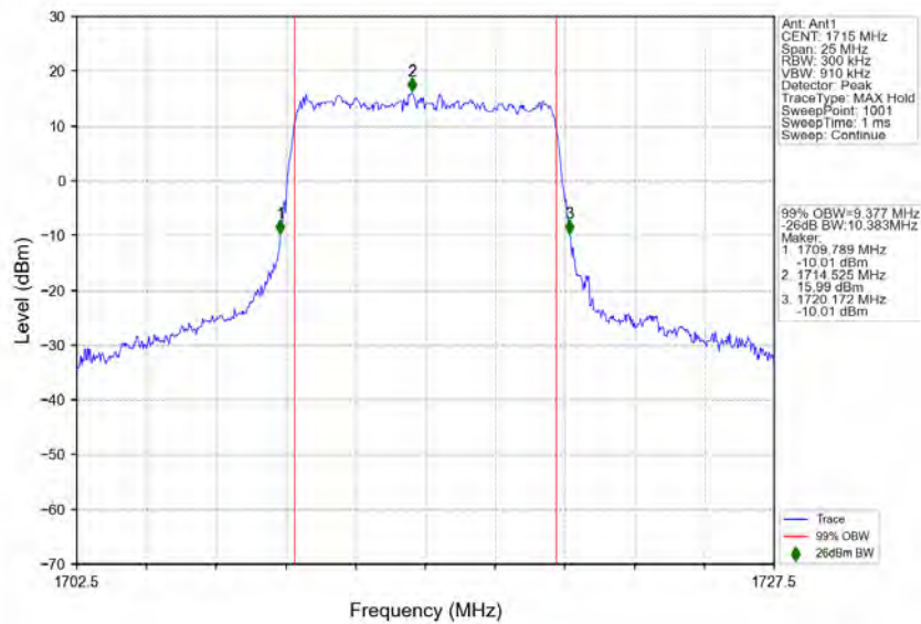
n66_15kHz_SISO_NTNV_10MHz_CP-OFDM_64 QAM_1715MHz_Outer_Full
