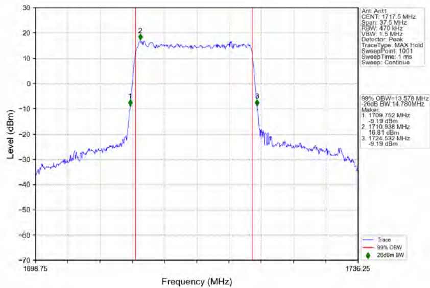
n66_15kHz_SISO_NTNV_15MHz_DFT-s-OFDM_64 QAM_1717.5MHz_Outer_Full
