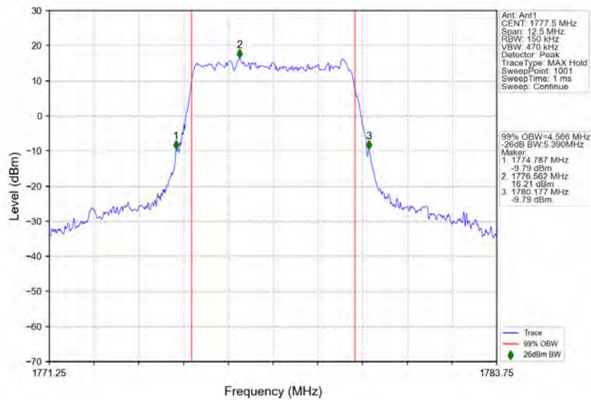
n66_15kHz_SISO_NTNV_5MHz_CP-OFDM_QPSK_1777.5MHz_Outer_Full
