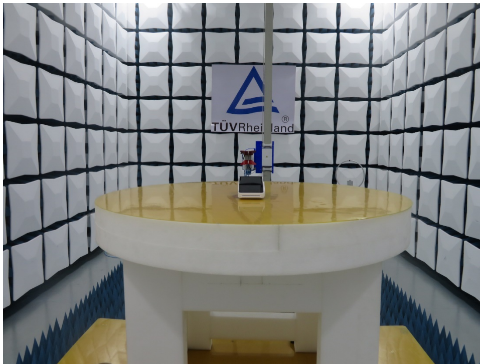
Photograph 3: Set-up for Radiated Spurious Emissions, Above 1GHz
