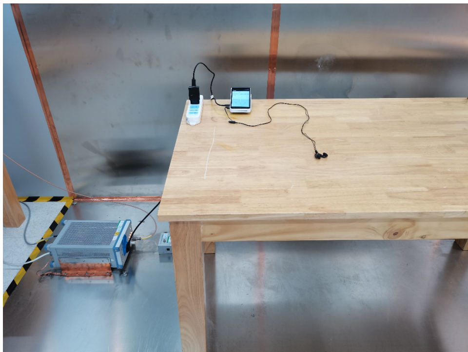
Photograph 4: Set-up for Conducted Emissions on AC Mains
