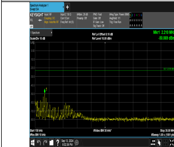
Band26_10MHz_16QAM_26990_1RB#49_0.15~30_0.15~30
