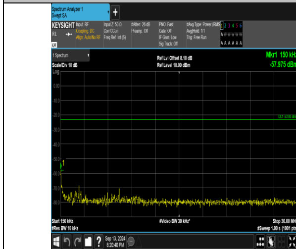
Band26_15MHz_16QAM_26865_1RB#74_0.15~30_0.15~30
