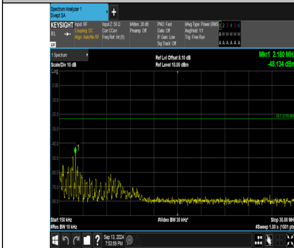
Band26_10MHz_16QAM_26840_50RB#0_0.15~30_0.15~30
