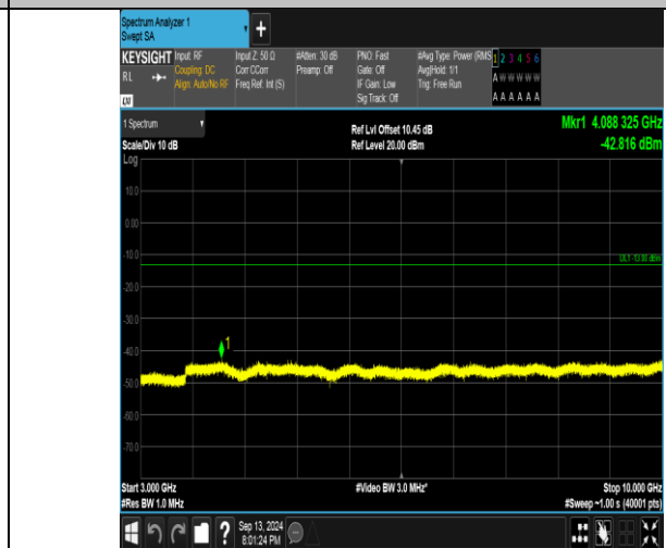
Band26_10MHz_16QAM_26990_1RB#0_3000~10000_3000~10000
