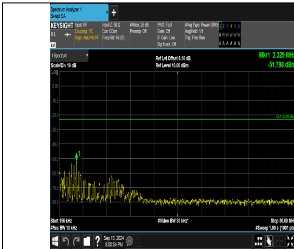
Band26_10MHz_16QAM_26990_1RB#0_0.15~30_0.15~30
