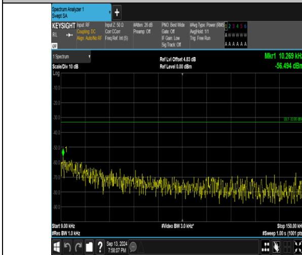
Band26_10MHz_QPSK_26915_50RB#0_0.009~0.15_0.009~0.15
