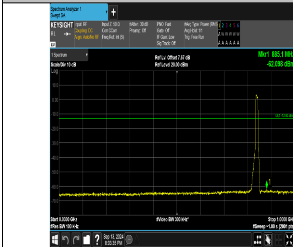
Band26_10MHz_QPSK_26990_50RB#0_30~1000_30~1000
