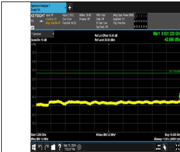
Band26_10MHz_QPSK_26840_50RB#0_3000~10000_3000~10000
