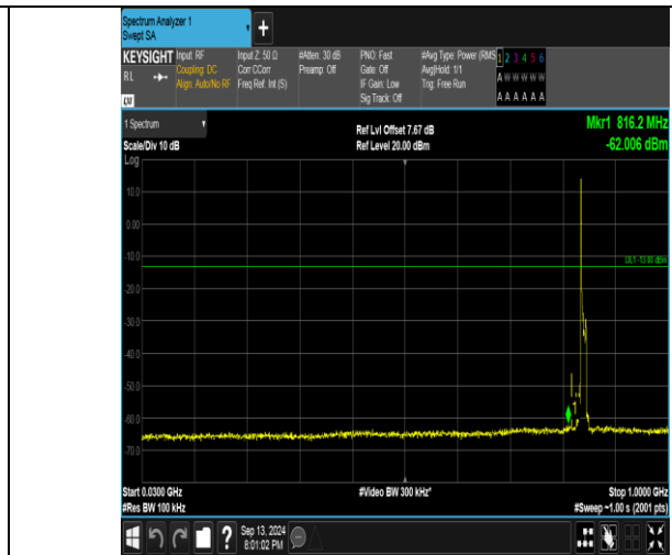
Band26_10MHz_16QAM_26990_1RB#0_30~1000_30~1000
