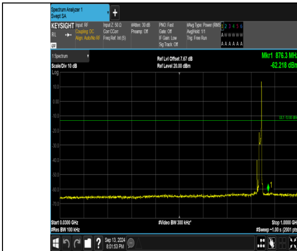
Band26_10MHz_QPSK_26990_1RB#49_30~1000_30~1000
