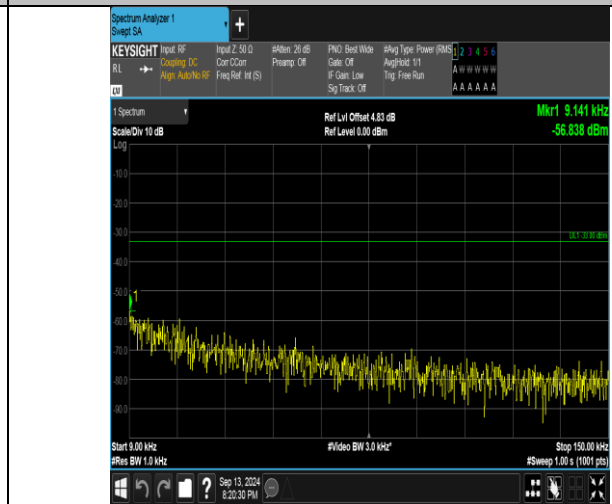
Band26_15MHz_16QAM_26865_1RB#74_0.009~0.15_0.009~0.15
