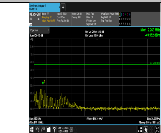
Band26_10MHz_QPSK_26990_1RB#49_0.15~30_0.15~30
