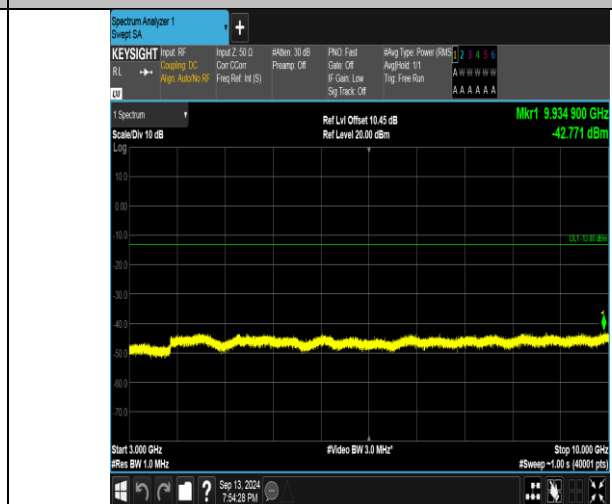
Band26_10MHz_16QAM_26840_50RB#0_3000~10000_3000~10000
