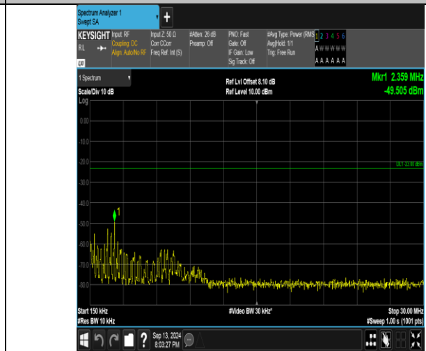
Band26_10MHz_QPSK_26990_50RB#0_0.15~30_0.15~30
