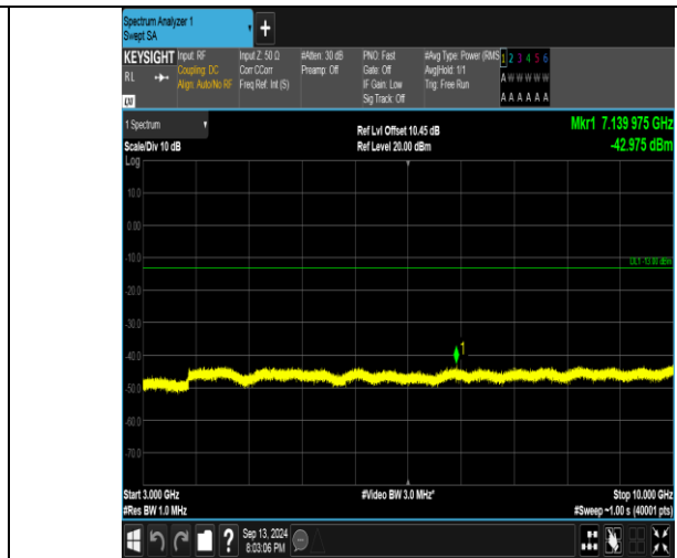
Band26_10MHz_16QAM_26990_1RB#49_3000~10000_3000~10000
