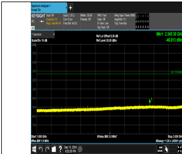
Band26_10MHz_16QAM_26990_1RB#49_1000~3000_1000~3000
