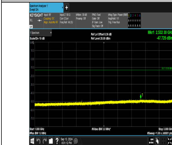
Band26_10MHz_16QAM_26990_1RB#0_1000~3000_1000~3000
