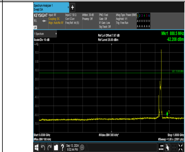
Band26_10MHz_16QAM_26990_1RB#49_30~1000_30~1000
