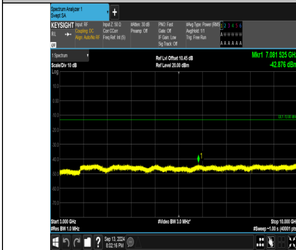
Band26_10MHz_QPSK_26990_1RB#49_3000~10000_3000~10000
