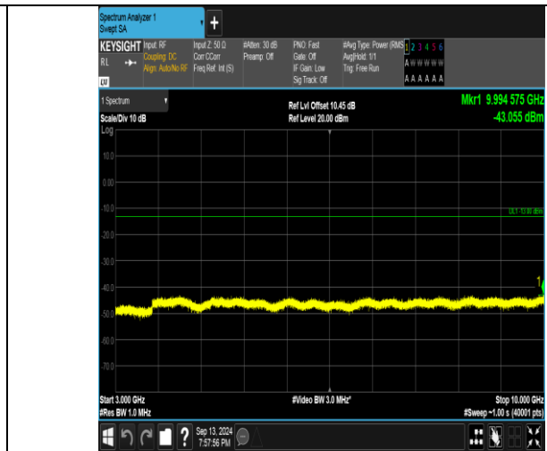
Band26_10MHz_16QAM_26915_1RB#49_3000~10000_3000~10000
