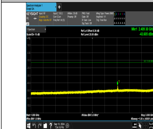
Band26_10MHz_16QAM_26840_50RB#0_1000~3000_1000~3000
