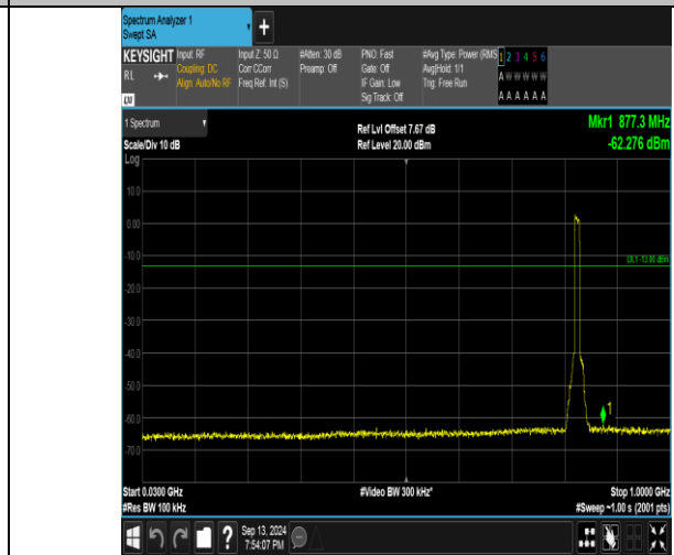
Band26_10MHz_16QAM_26840_50RB#0_30~1000_30~1000
