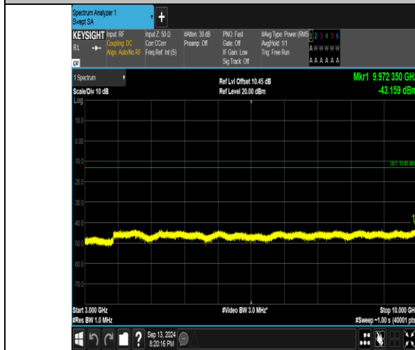
Band26_15MHz_QPSK_26865_1RB#74_3000~10000_3000~10000
