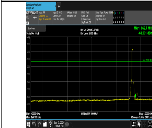
Band26_10MHz_QPSK_26915_50RB#0_30~1000_30~1000
