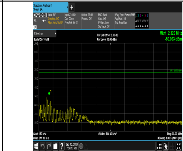
Band26_10MHz_QPSK_26915_50RB#0_0.15~30_0.15~30
