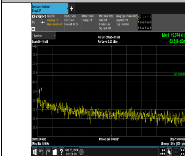
Band26_10MHz_QPSK_26990_1RB#49_0.009~0.15_0.009~0.15
