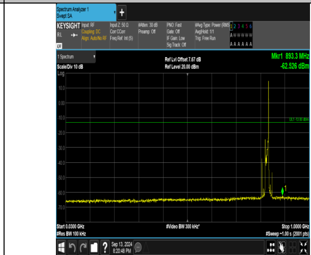
Band26_15MHz_16QAM_26865_1RB#74_30~1000_30~1000
