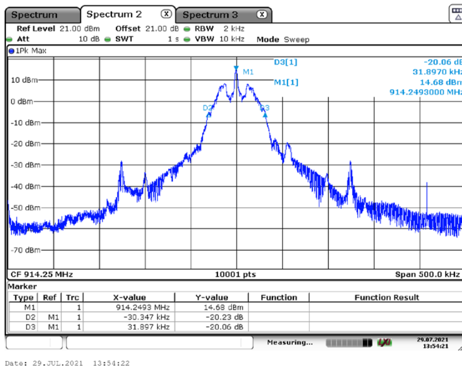
Plot 3: mid channel, 20 dB BW
