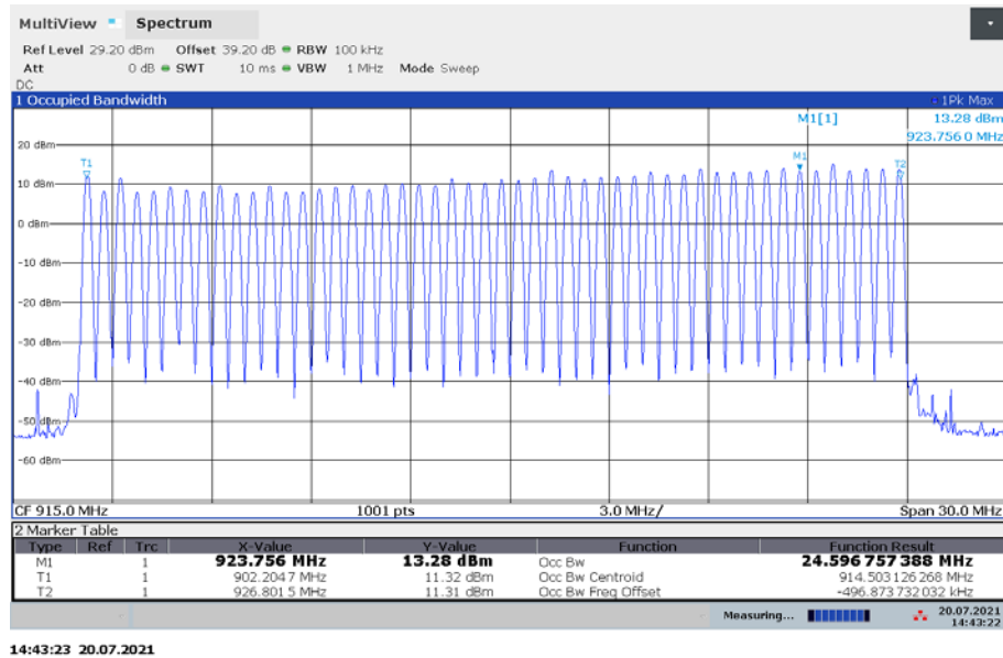
Plot 1: Number of hopping channels
