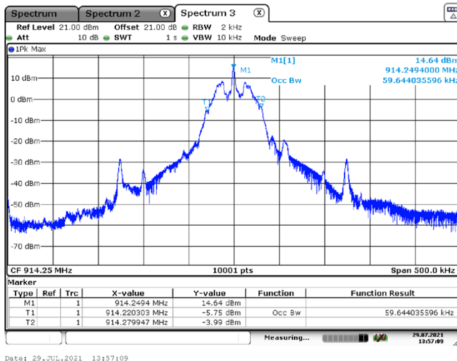
Plot 4: mid channel, 99% OBW
