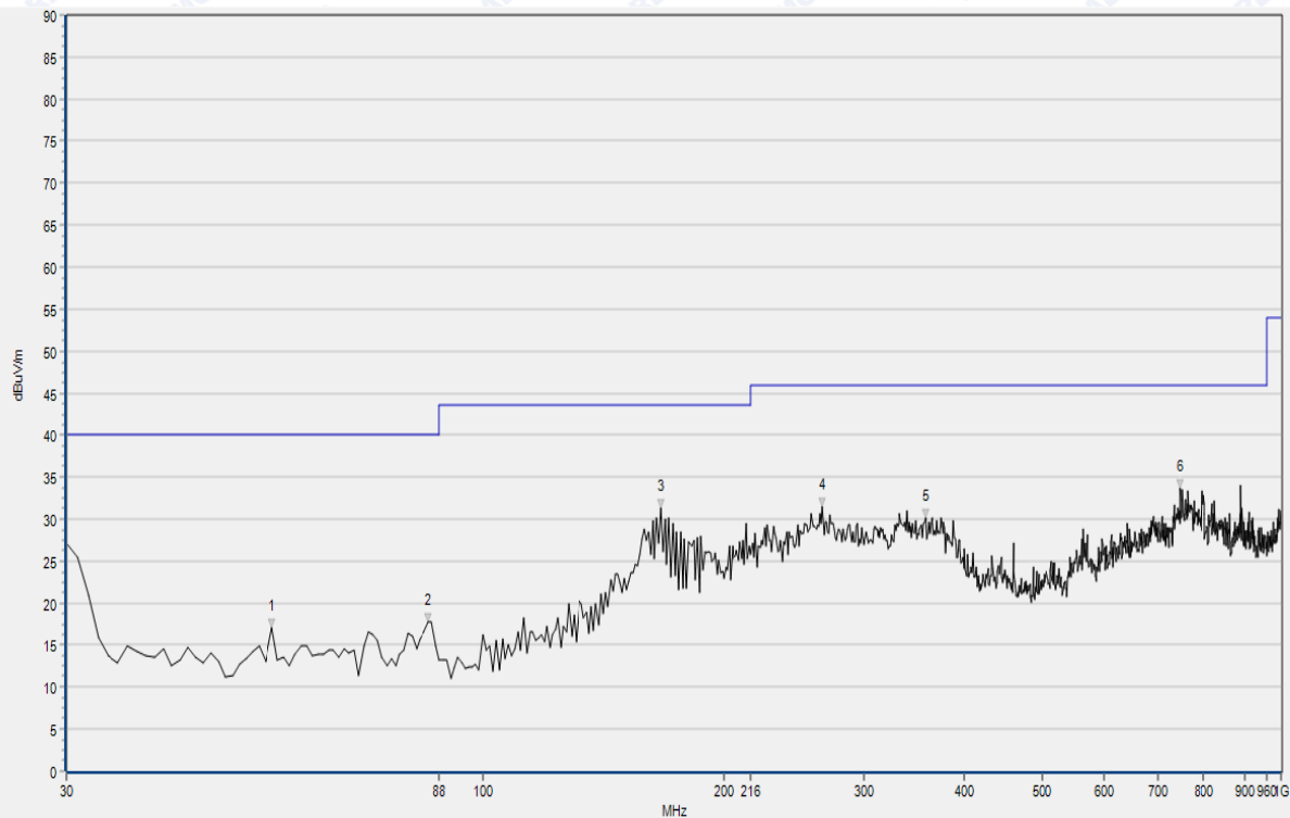
(Plot C: 30MHz – 1GHz, Test Antenna Horizontal)
