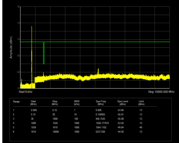
Band13 QAM16 BW=5MHz Channel=23205 RB Size=25 Position=#0
