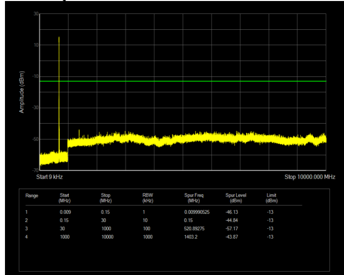
Band12 QAM16 BW=3MHz Channel=23095 RB Size=15 Position=#0
