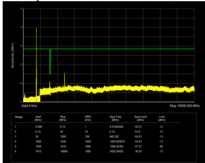
Band13 QAM16 BW=5MHz Channel=23230 RB Size=25 Position=#0
