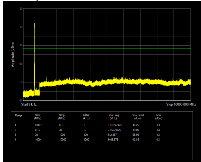
Band12 QAM16 BW=5MHz Channel=23095 RB Size=25 Position=#0
