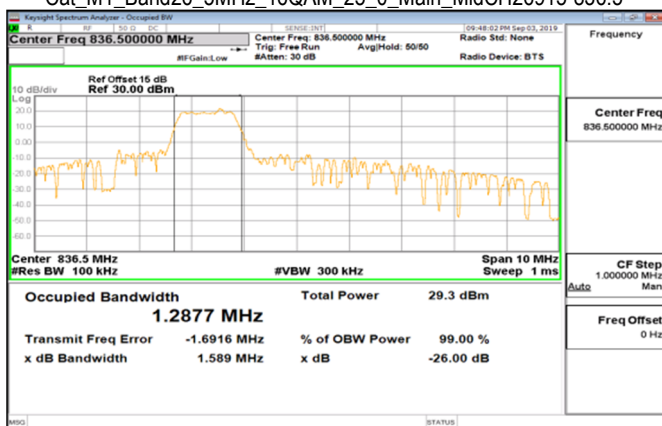
Cat_M1_Band26_5MHz_16QAM_25_0_Main_MidCH26915-836.5
