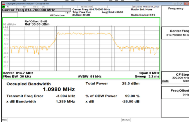
Cat_M1_Band26_Part90s_1_4MHz_16QAM_6_0_Main_LowCH26697-814.7
