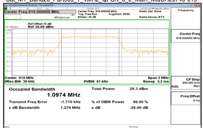
Cat_M1_Band26_Part90s_1_4MHz_QPSK_6_0_Main_MidCH26740-819
