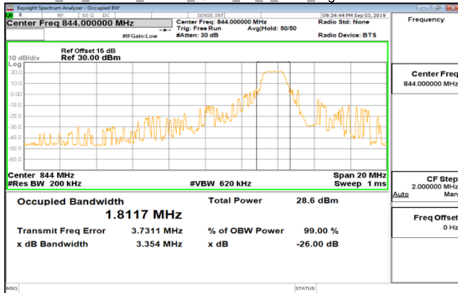
Cat_M1_Band26_10MHz_QPSK_50_0_Main_HighCH26990-844
