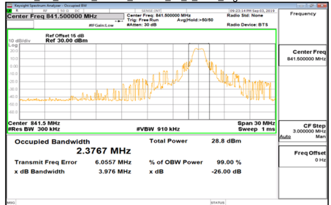
Cat_M1_Band26_15MHz_16QAM_75_0_Main_HighCH26965-841.5
