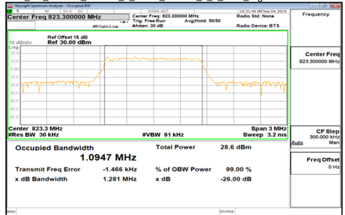
Cat_M1_Band26_Part90s_1_4MHz_16QAM_6_0_Main_HighCH26783-823.3
