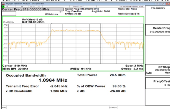
Cat_M1_Band26_Part90s_1_4MHz_16QAM_6_0_Main_MidCH26740-819
