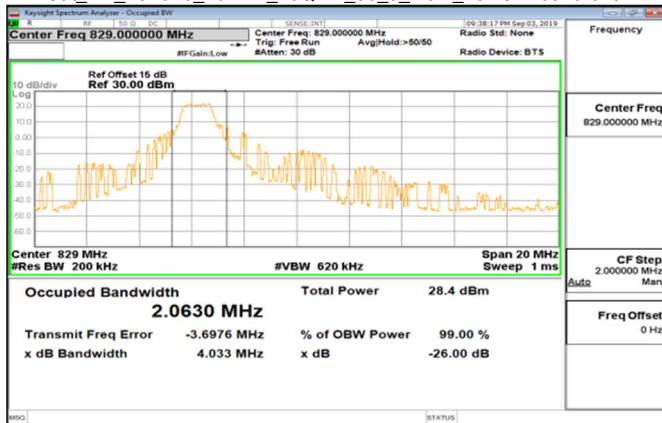
Cat_M1_Band26_10MHz_16QAM_50_0_Main_LowCH26840-829
