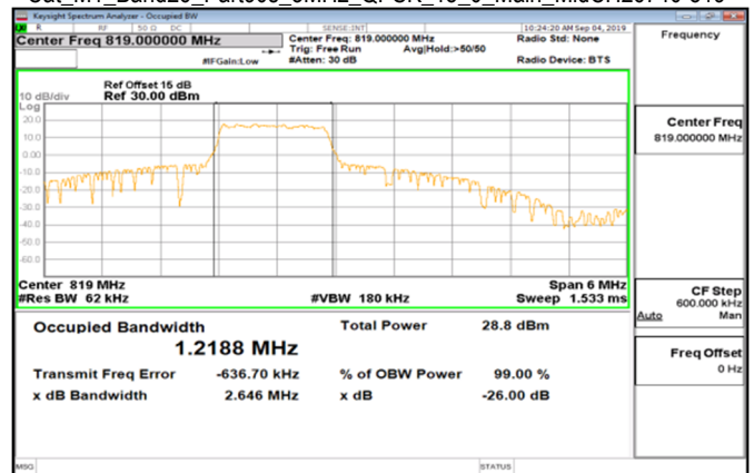
Cat_M1_Band26_Part90s_3MHz_QPSK_15_0_Main_MidCH26740-819
