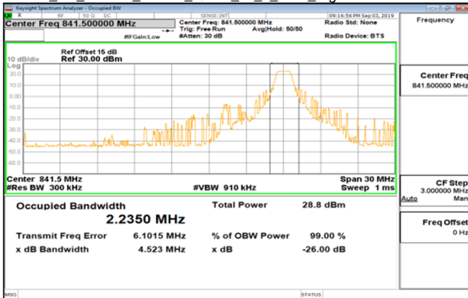
Cat_M1_Band26_15MHz_QPSK_75_0_Main_HighCH26965-841.5
