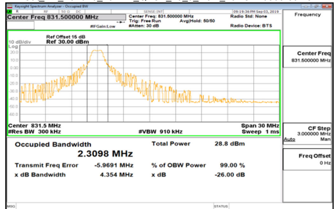
Cat_M1_Band26_15MHz_QPSK_75_0_Main_LowCH26865-831.5
