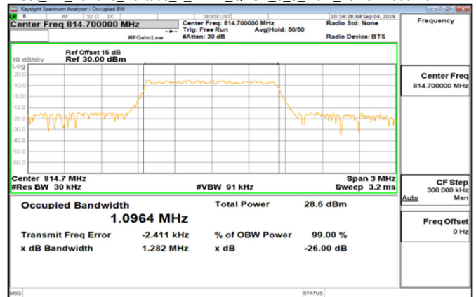
Cat_M1_Band26_Part90s_1_4MHz_QPSK_6_0_Main_LowCH26697-814.7
