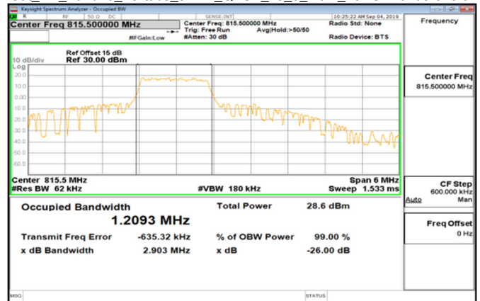
Cat_M1_Band26_Part90s_3MHz_QPSK_15_0_Main_LowCH26705-815.5
