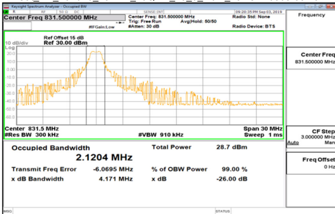
Cat_M1_Band26_15MHz_16QAM_75_0_Main_LowCH26865-831.5
