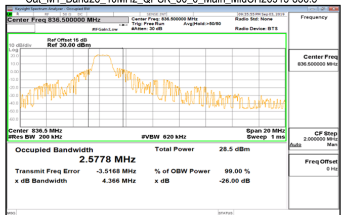
Cat_M1_Band26_10MHz_QPSK_50_0_Main_MidCH26915-836.5
