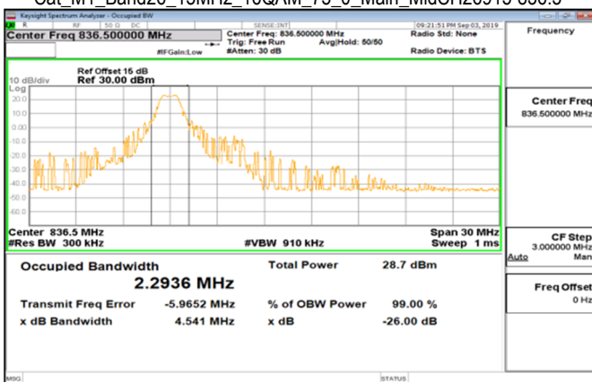
Cat_M1_Band26_15MHz_16QAM_75_0_Main_MidCH26915-836.5
