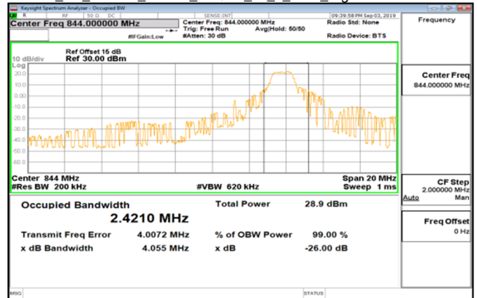
Cat_M1_Band26_10MHz_16QAM_50_0_Main_HighCH26990-844
