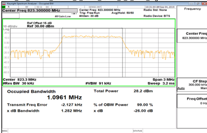
Cat_M1_Band26_Part90s_1_4MHz_QPSK_6_0_Main_HighCH26783-823.3
