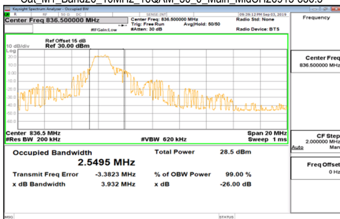
Cat_M1_Band26_10MHz_16QAM_50_0_Main_MidCH26915-836.5
