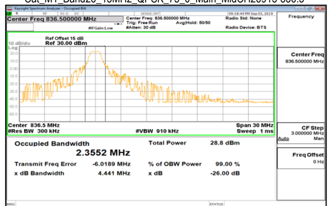
Cat_M1_Band26_15MHz_QPSK_75_0_Main_MidCH26915-836.5
