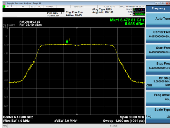
Plot 7-117. Power Spectral Density Plot Antenna 3b (20MHz 802.11a (UNII Band 6) – Ch. 105)
