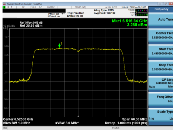
Plot 7-118. Power Spectral Density Plot Antenna 3b (40MHz 802.11ax (UNII Band 6) – Ch. 115)
