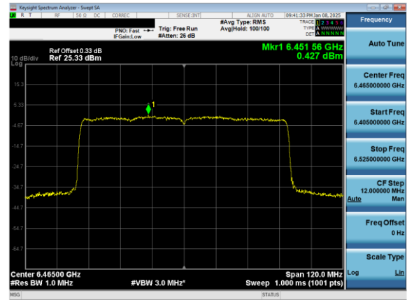
Plot 7-119. Power Spectral Density Plot Antenna 3b (80MHz 802.11ax (UNII Band 6) – Ch. 103)
