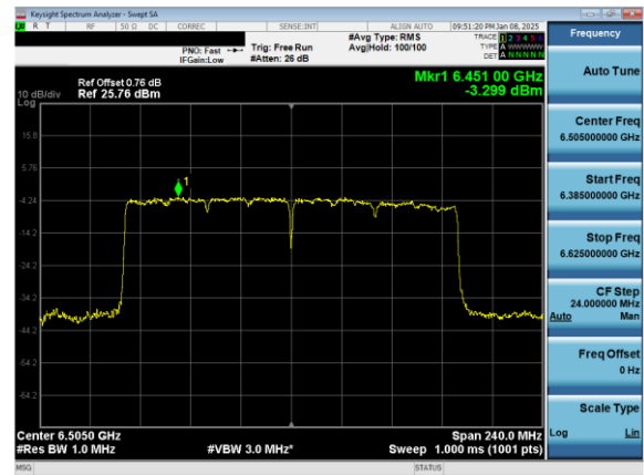
Plot 7-120. Power Spectral Density Plot Antenna 3b (160MHz 802.11ax (UNII Band 6) – Ch. 111)
