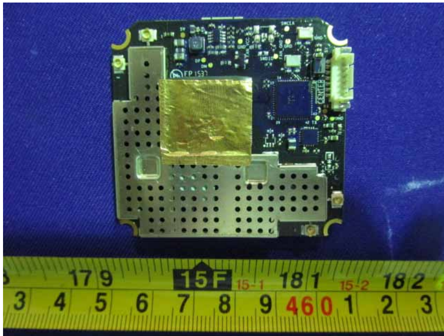
EUT –RF Module Top View (S/N: 151013002-1)
