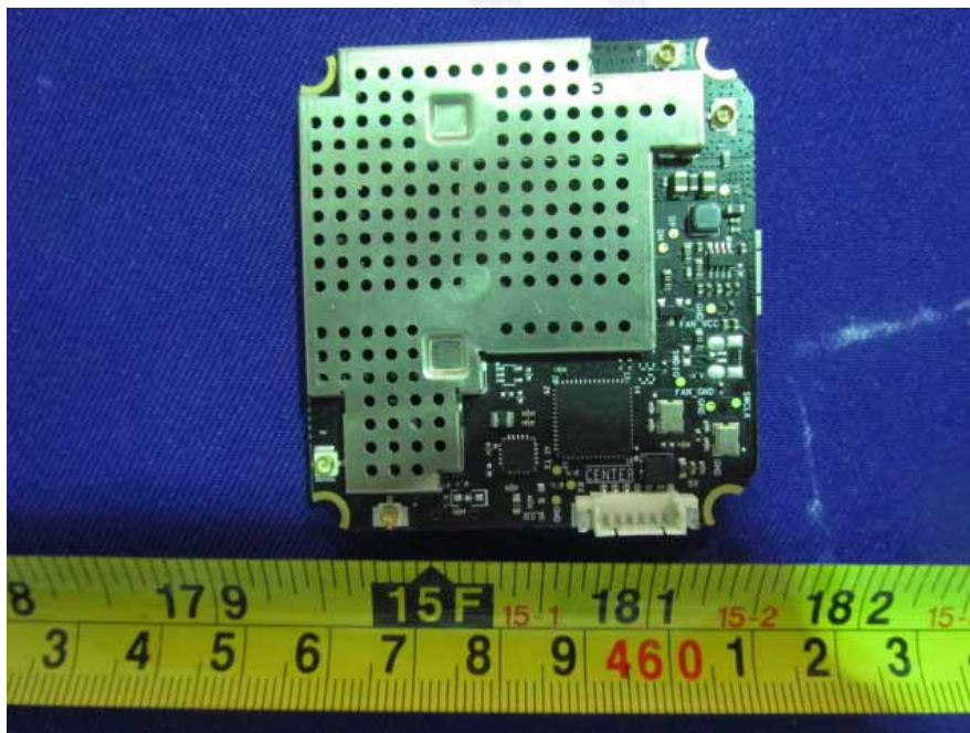
EUT –RF Module Top View (S/N: 151013002-2)
