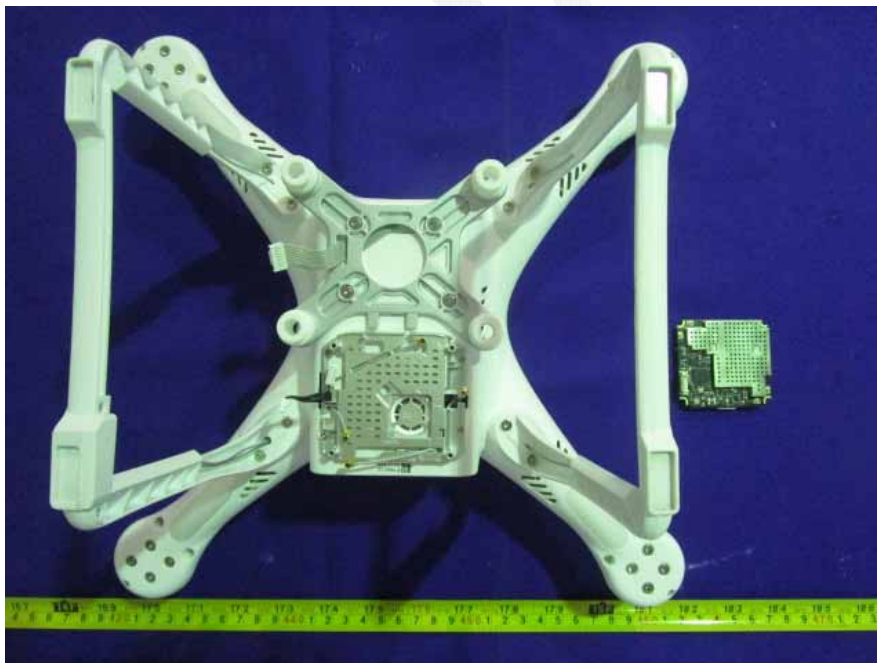
EUT –Uncover View (S/N: 151013002-2)
