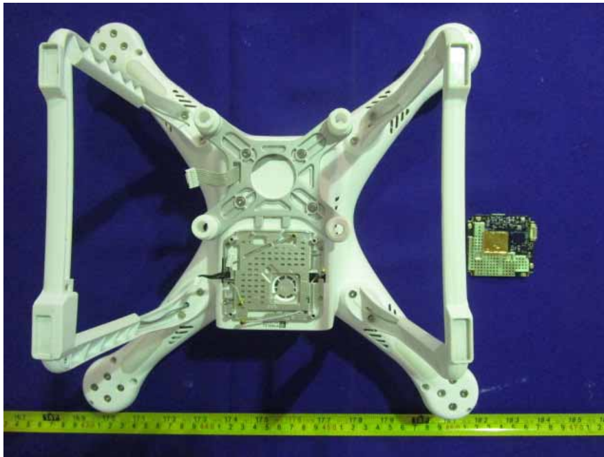
EUT –Uncover View (S/N: 151013002-1)
