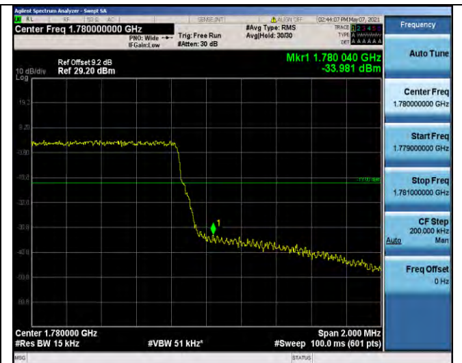
Band66-1.4MHz-16QAM-132665-6RB#0
