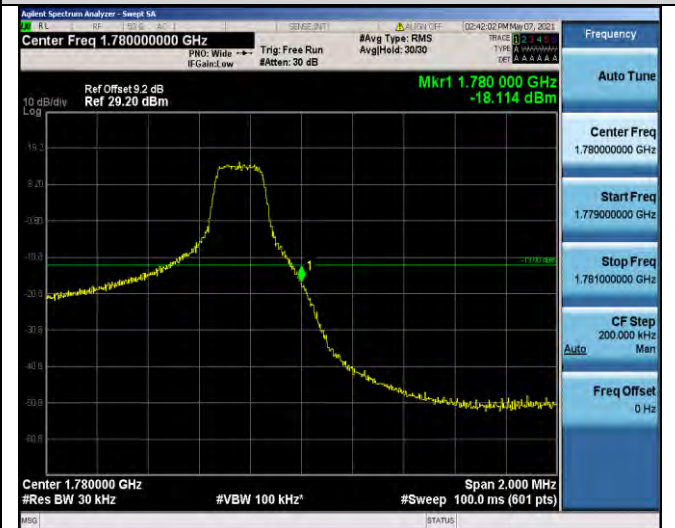
Band66-3MHz-16QAM-132657-1RB#14
