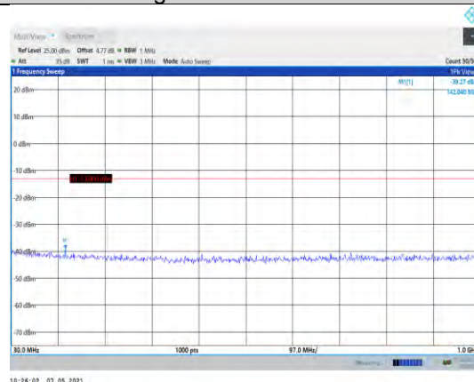
Band2-20MHz-16QAM-19100-1RB#0- Range1:30~1000MHz
