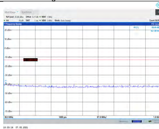
Band2-3MHz-QPSK-19185-1RB#0- Range1:30~1000MHz
