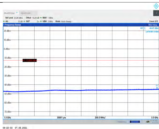
Band5-4132-1000~3000MHz
