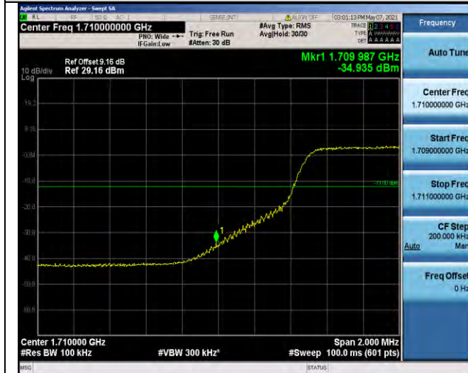
Band66-10MHz-16QAM-132022-50RB#0
