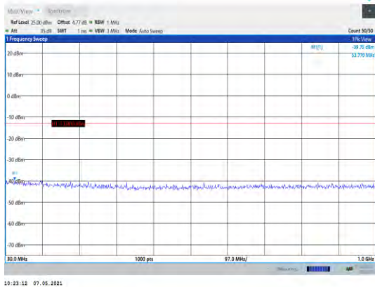
Band2-1.4MHz-QPSK-19193-1RB#0- Range1:30~1000MHz
