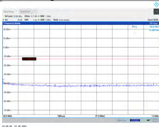
Band2-20MHz-16QAM-18900-1RB#0- Range1:30~1000MHz
