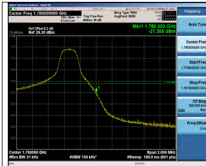
Band66-5MHz-16QAM-132647-1RB#24
