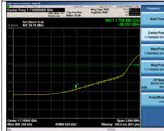
Band66-20MHz-QPSK-132072-100RB#0
