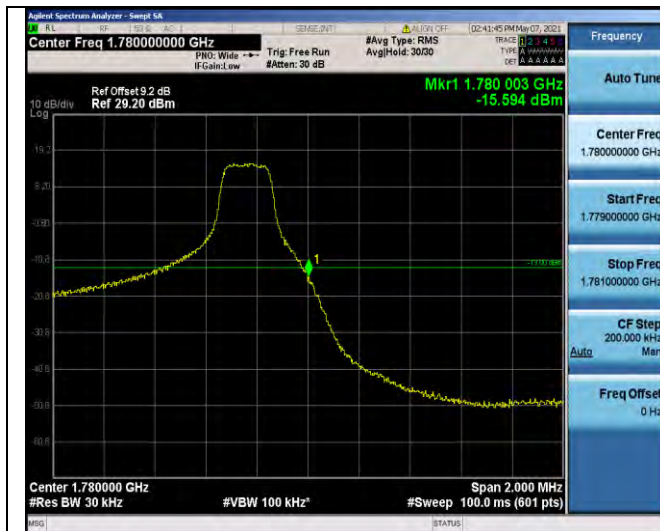
Band66-3MHz-QPSK-132657-1RB#14
