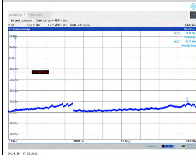
Band4-1513-1000~20000MHz
