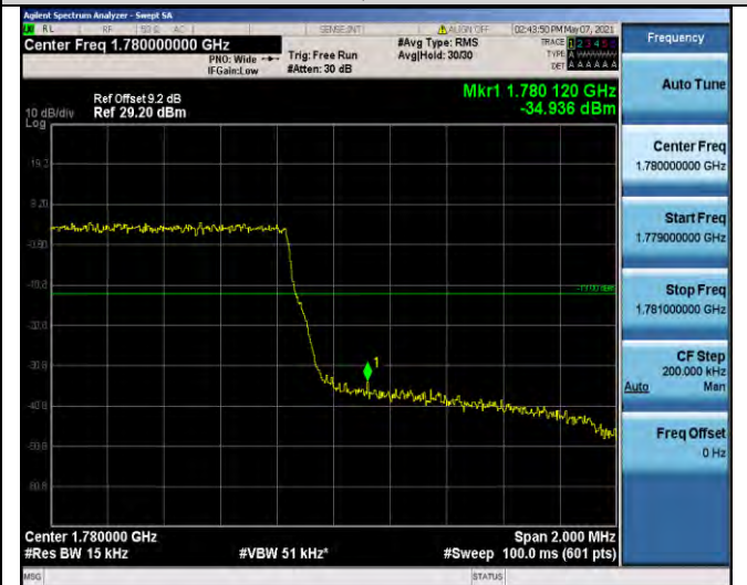
Band66-1.4MHz-QPSK-132665-6RB#0
