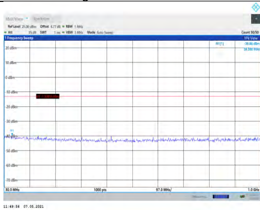
Band4-1.4MHz-QPSK-20175-1RB#0- Range1:30~1000MHz
