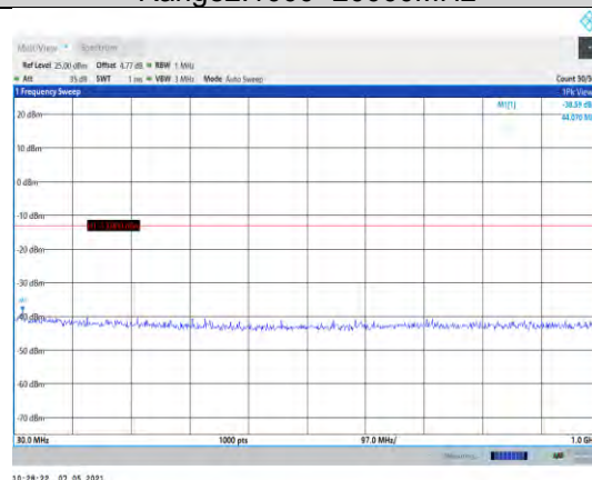
Band2-15MHz-QPSK-19125-1RB#0- Range1:30~1000MHz
