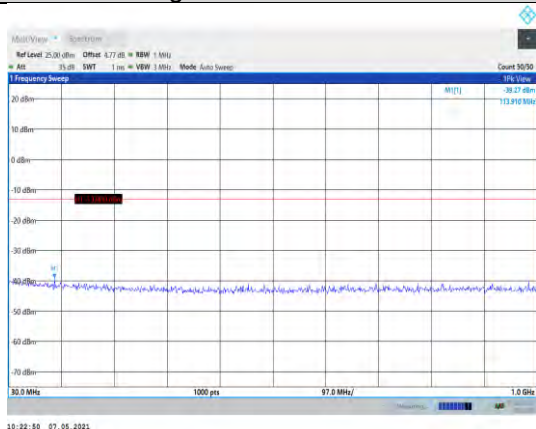
Band2-1.4MHz-16QAM-18900-1RB#0- Range1:30~1000MHz
