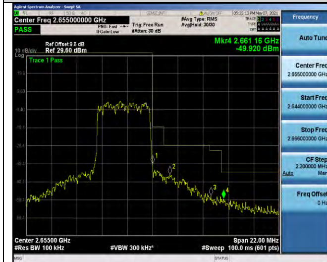
Band41-5MHz-16QAM-41215-25RB#0
