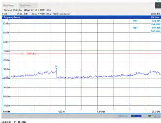
Band2-1.4MHz-QPSK-18607-1RB#0- Range2:1000~20000MHz
