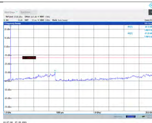
Band2-15MHz-QPSK-18900-1RB#0- Range2:1000~20000MHz
