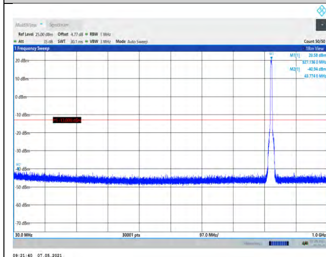
Band5-4132-30~1000MHz
