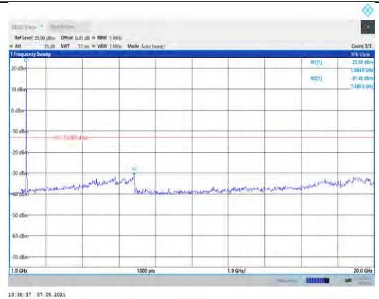
Band2-10MHz-16QAM-18900-1RB#0- Range2:1000~20000MHz
