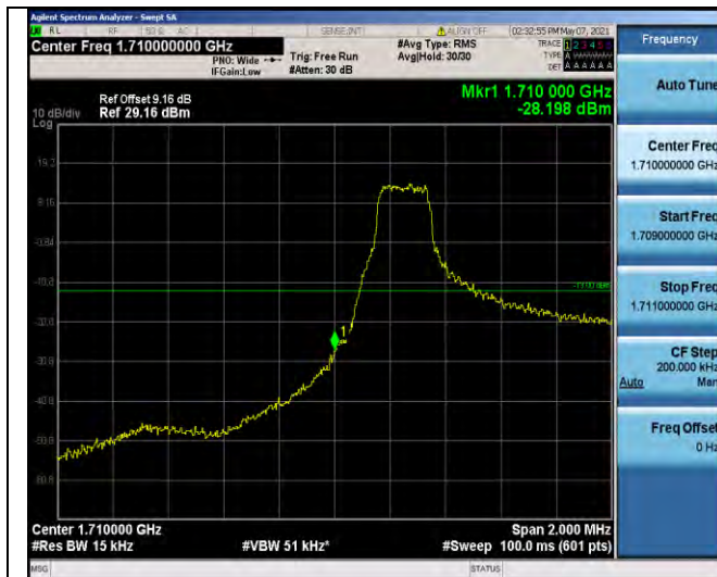
Band66-1.4MHz-16QAM-131979-1RB#0
