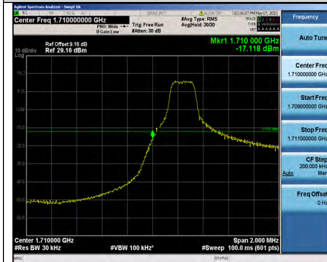
Band66-3MHz-16QAM-131987-1RB#0
