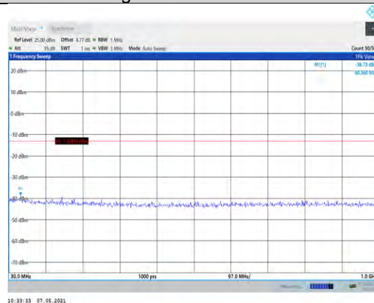
Band2-3MHz-16QAM-19185-1RB#0- Range1:30~1000MHz
