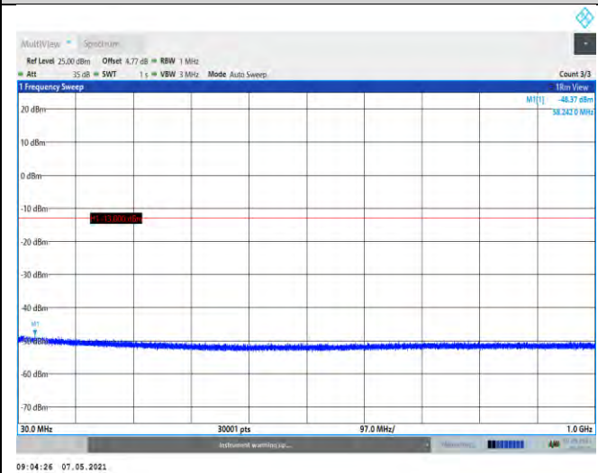
Band2-9400-30~1000MHz
