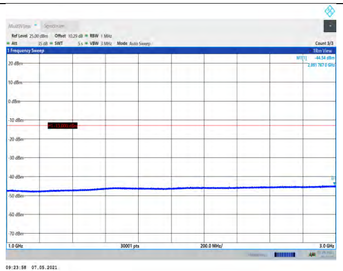
Band5-4233-1000~3000MHz
