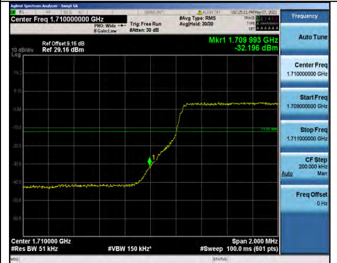
Band66-5MHz-16QAM-131997-25RB#0
