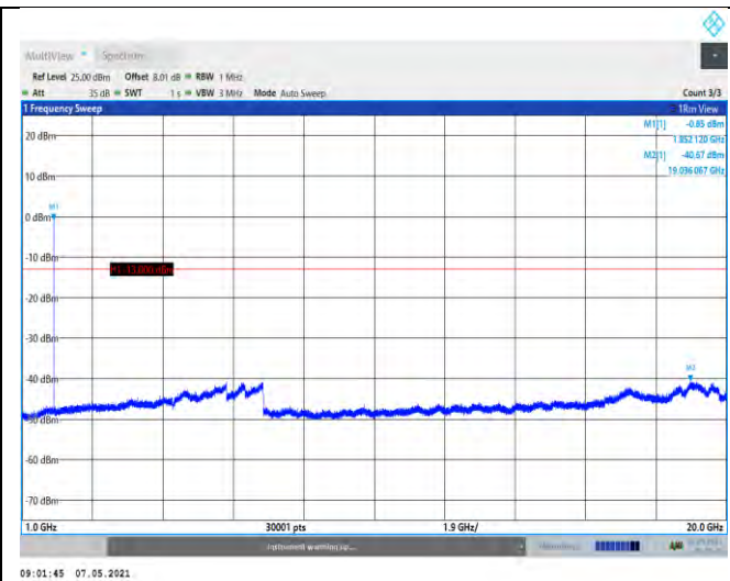
Band2-9262-1000~20000MHz
