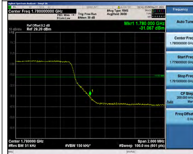
Band66-5MHz-16QAM-132647-25RB#0
