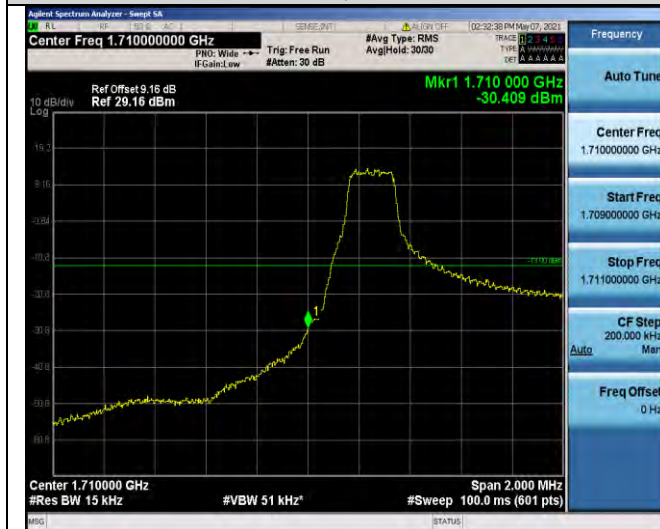
Band66-1.4MHz-QPSK-131979-1RB#0
