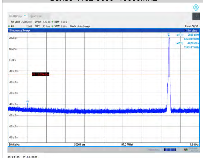
Band5-4233-30~1000MHz
