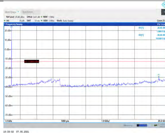
Band2-3MHz-16QAM-18900-1RB#0- Range2:1000~20000MHz
