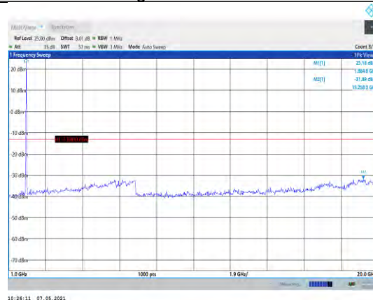
Band2-20MHz-16QAM-19100-1RB#0- Range2:1000~20000MHz
