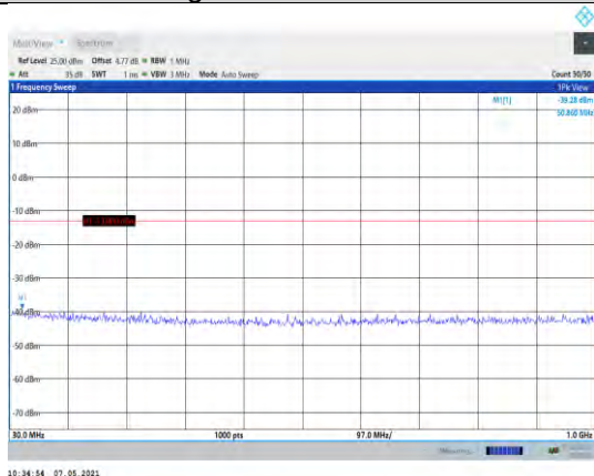
Band2-5MHz-16QAM-18900-1RB#0- Range1:30~1000MHz
