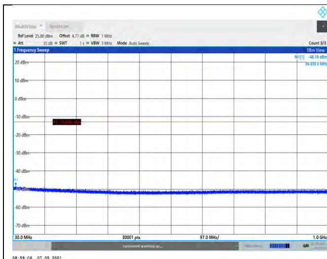
Band2-9262-30~1000MHz
