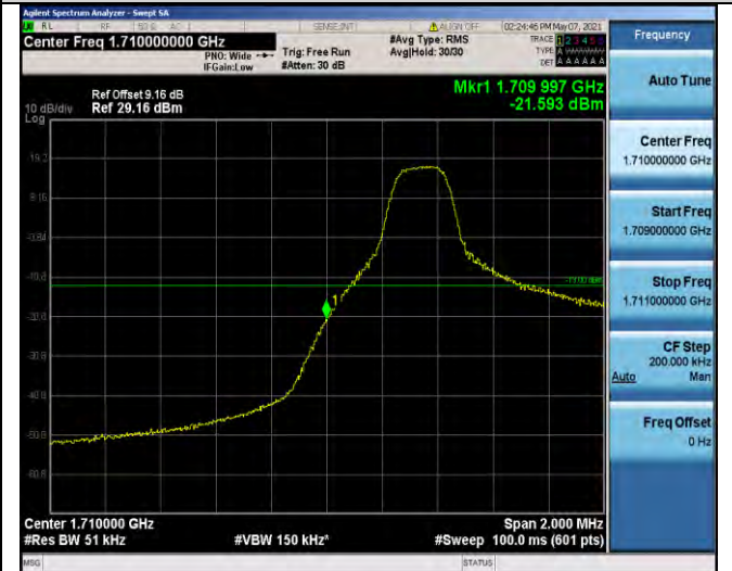
Band66-5MHz-16QAM-131997-1RB#0
