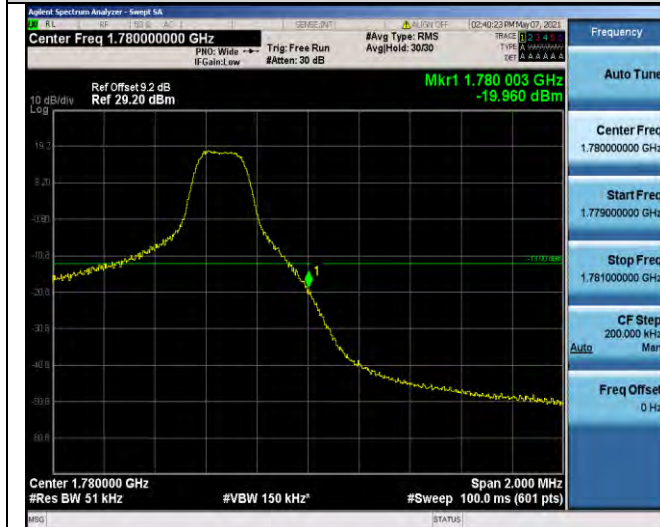
Band66-5MHz-QPSK-132647-1RB#24
