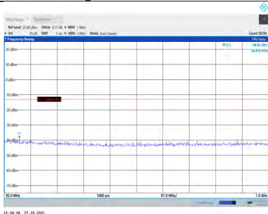
Band2-5MHz-QPSK-18900-1RB#0- Range1:30~1000MHz
