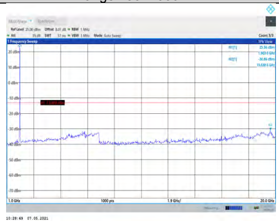
Band2-15MHz-16QAM-19125-1RB#0- Range2:1000~20000MHz
