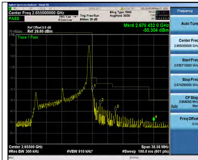
Band41-15MHz-QPSK-41165-1RB#74
