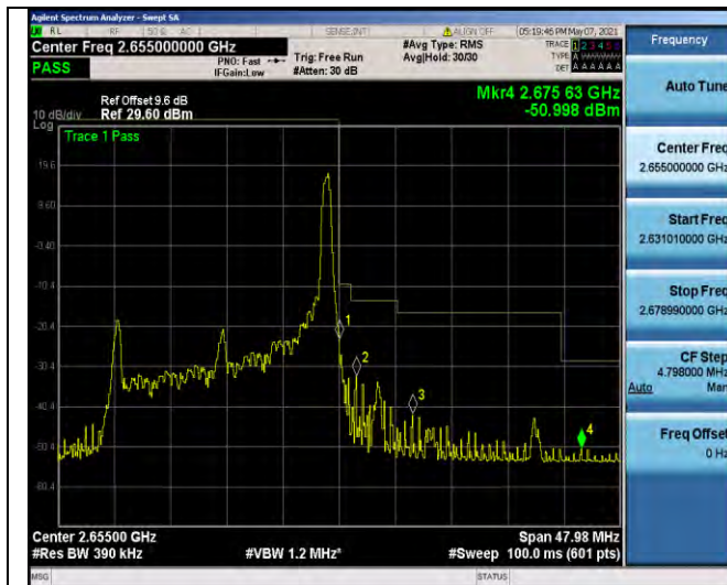
Band41-20MHz-16QAM-41140-1RB#99
