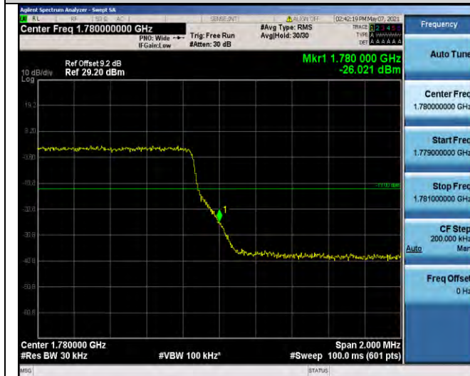
Band66-3MHz-QPSK-132657-15RB#0
