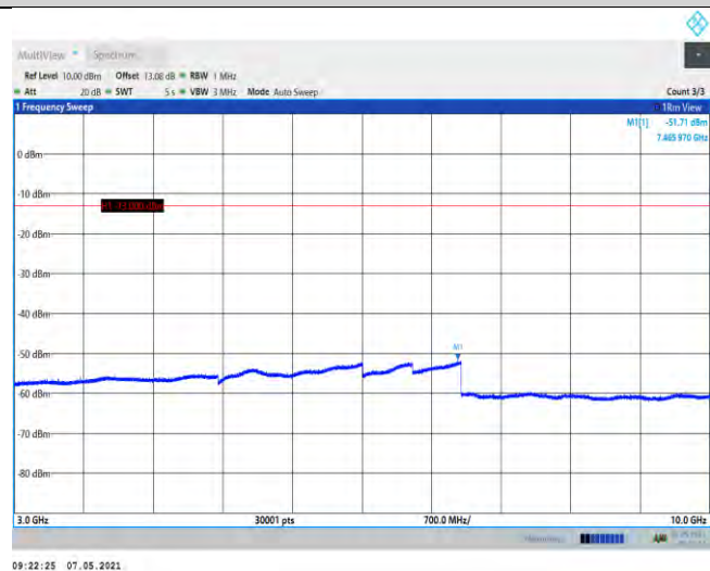
Band5-4132-3000~10000MHz
