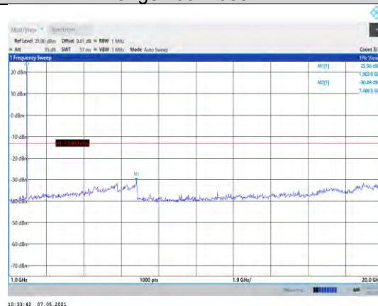
Band2-3MHz-16QAM-19185-1RB#0- Range2:1000~20000MHz
