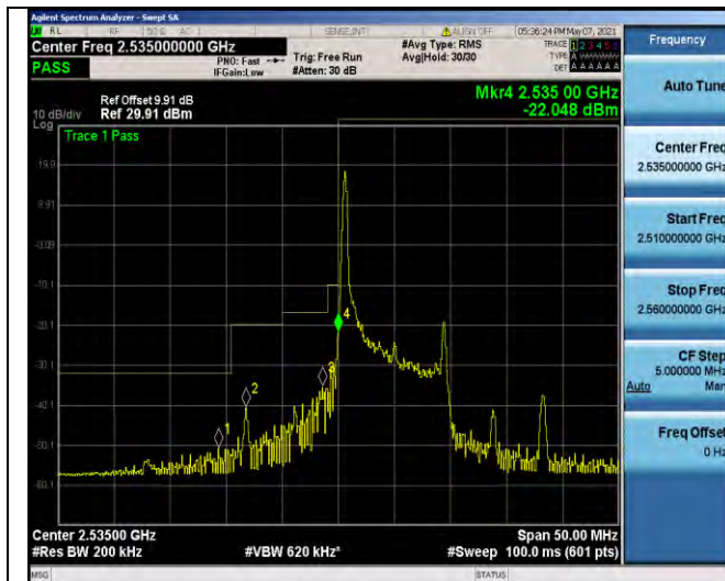
Band41-10MHz-16QAM-40090-1RB#0
