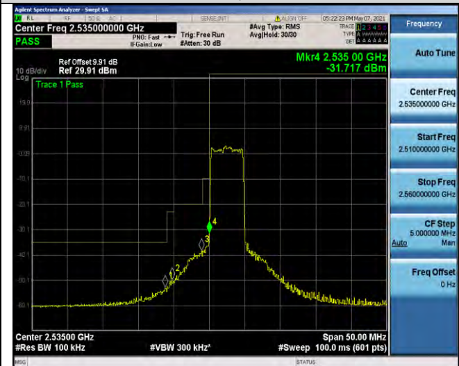
Band41-5MHz-16QAM-40065-25RB#0
