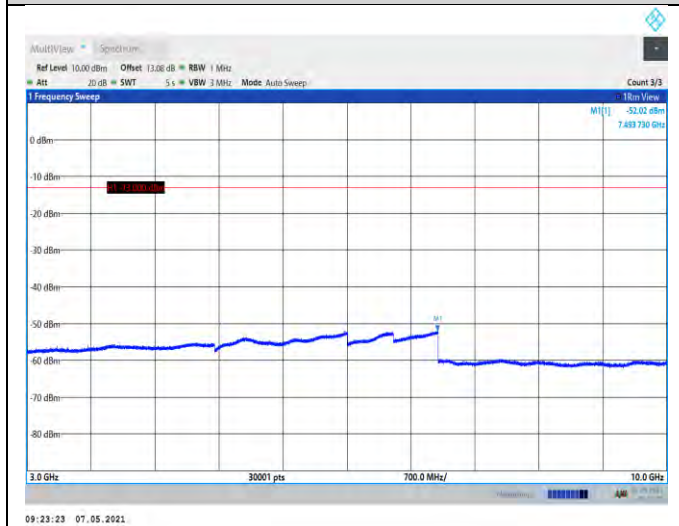
Band5-4182-3000~10000MHz
