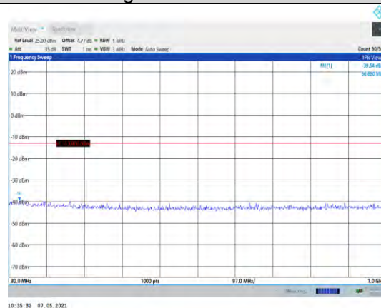
Band2-5MHz-16QAM-19175-1RB#0- Range1:30~1000MHz
