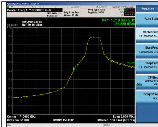
Band66-5MHz-QPSK-131997-1RB#0
