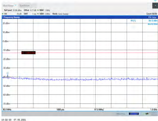
Band2-1.4MHz-QPSK-18900-1RB#0- Range1:30~1000MHz
