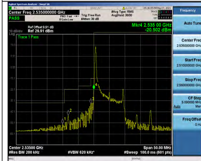
Band41-10MHz-QPSK-40090-1RB#0
