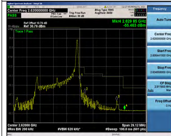
Band38-10MHz-QPSK-38200-1RB#49
