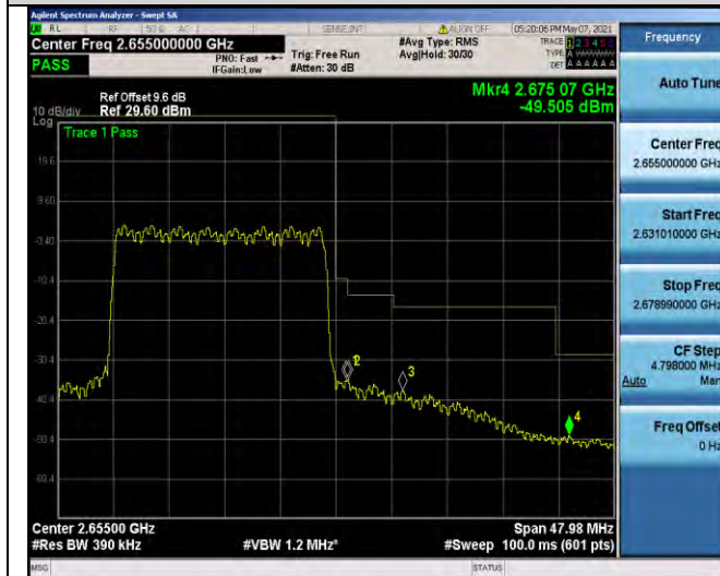
Band41-20MHz-16QAM-41140-100RB#0
