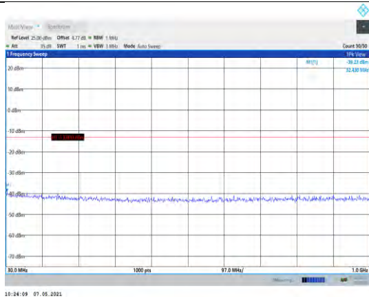
Band2-20MHz-16QAM-18700-1RB#0- Range1:30~1000MHz
