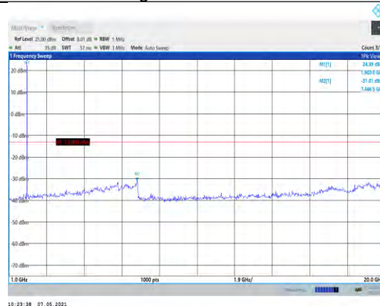
Band2-1.4MHz-16QAM-19193-1RB#0- Range2:1000~20000MHz
