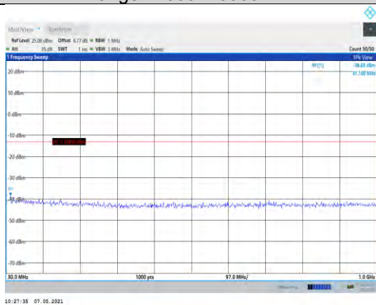
Band2-15MHz-16QAM-18900-1RB#0- Range1:30~1000MHz
