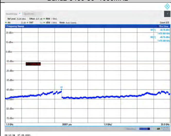
Band2-9400-1000~20000MHz
