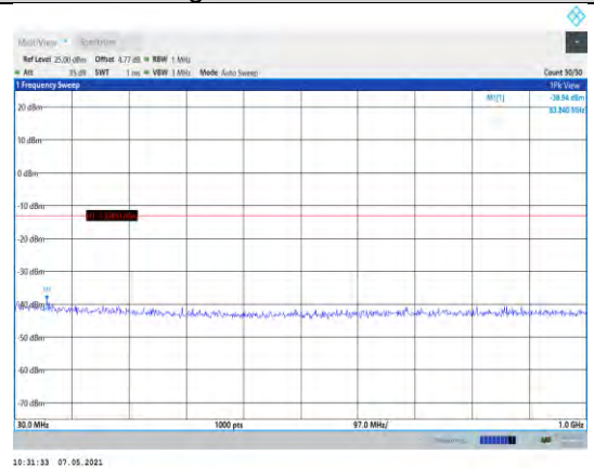
Band2-10MHz-16QAM-19150-1RB#0- Range1:30~1000MHz
