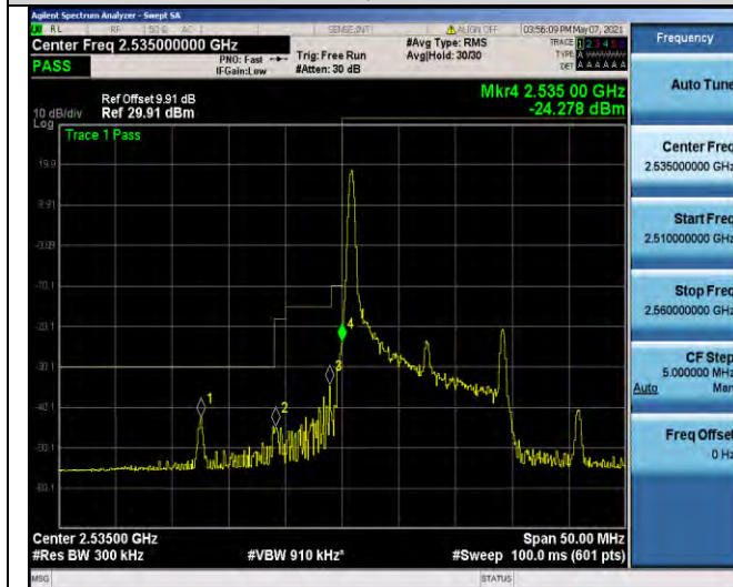
Band41-15MHz-16QAM-40115-1RB#0
