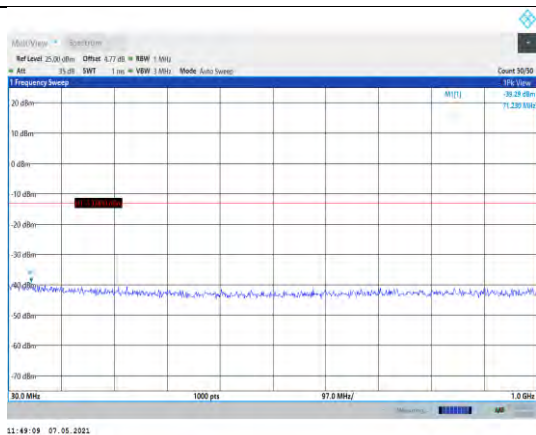
Band4-1.4MHz-QPSK-19957-1RB#0- Range1:30~1000MHz
