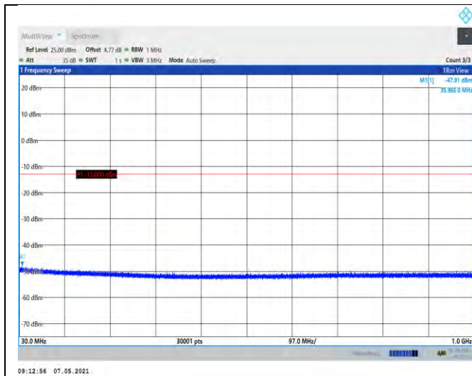
Band2-9538-30~1000MHz
