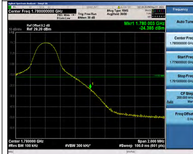
Band66-10MHz-16QAM-132622-1RB#49
