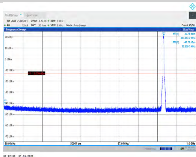
Band5-4182-30~1000MHz
