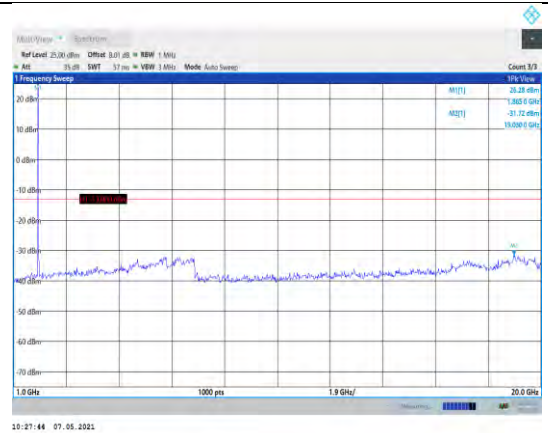
Band2-15MHz-16QAM-18900-1RB#0- Range2:1000~20000MHz
