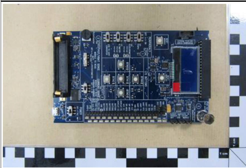
Evaluation Board Top
