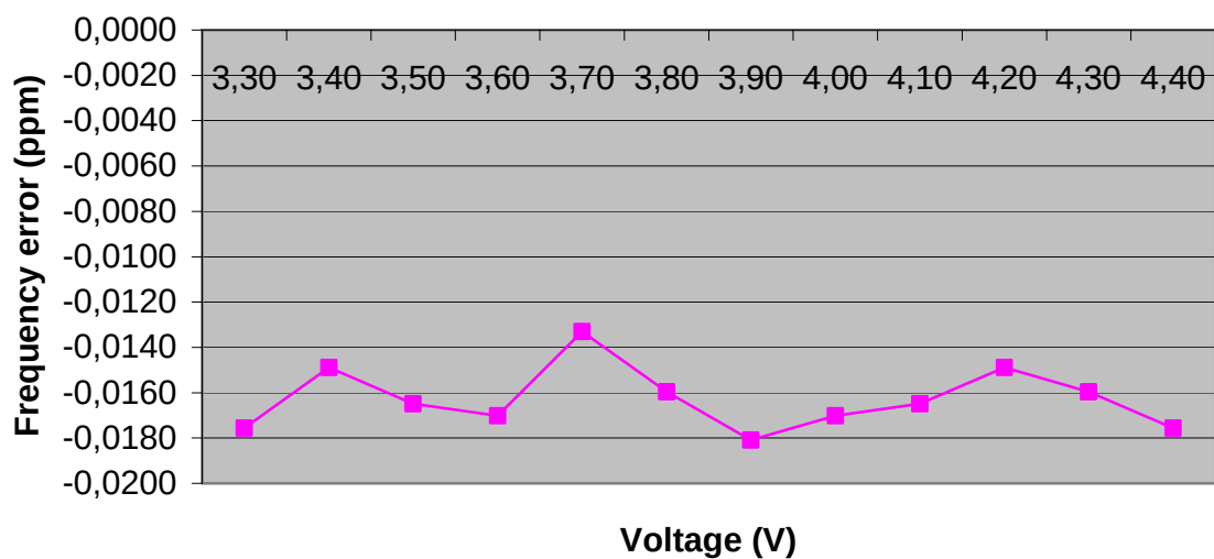
Frequency Error vs. Voltage
