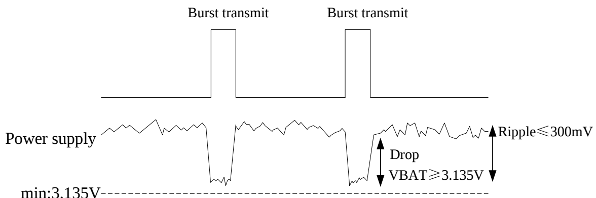
Figure 3-3 Power Supply Requirement
