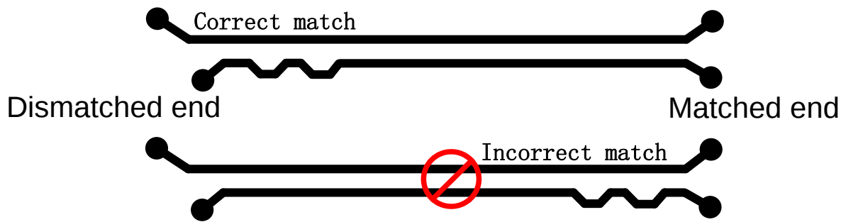
Figure 3-13 Length Match Design of PCIe Difference Pair
