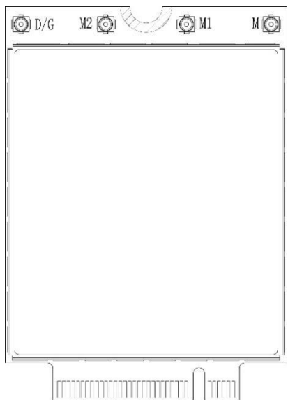
Figure 4-1 RF connectors
