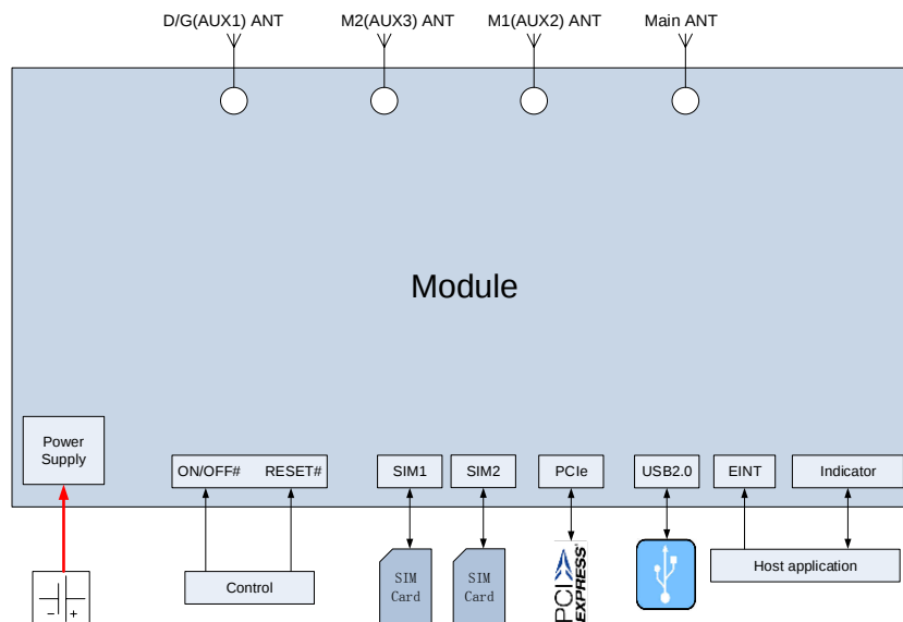
Figure2-1 Application Framework
