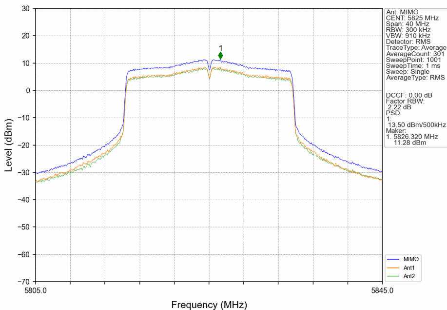
802.11ax(HEW20)_HCH_5825MHz_RU242_Left_MIMO_NTNV
