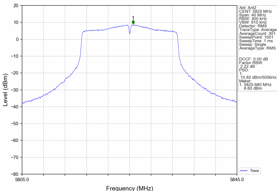
802.11ac(VHT20)_HCH_5825MHz_MIMO_NTNV
