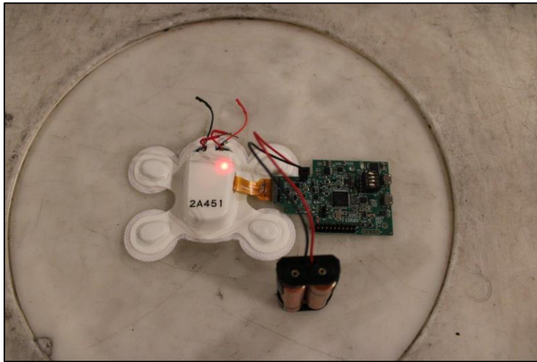
Closeup View of EUT
