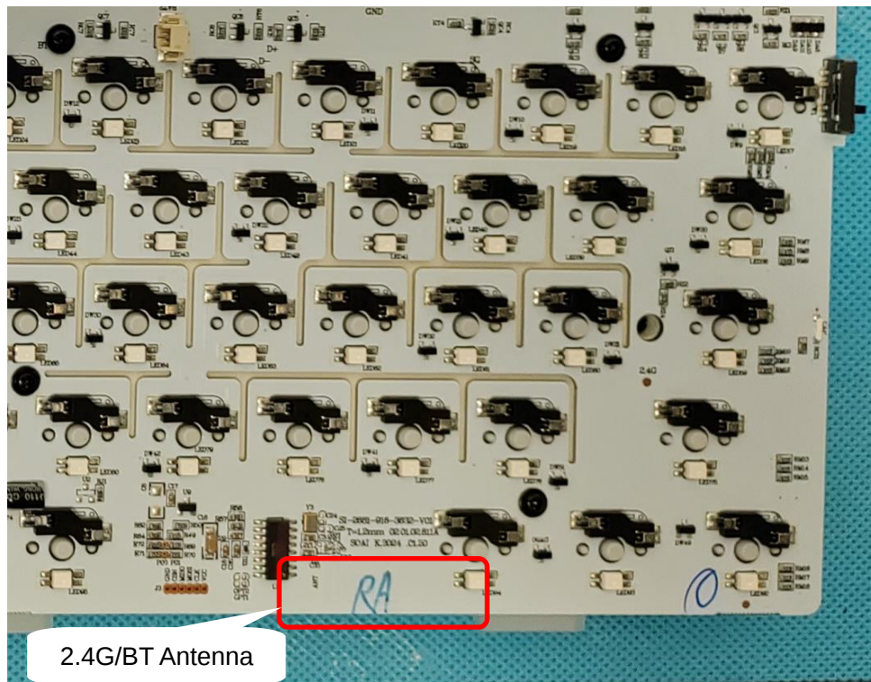
INTERNAL VIEW OF EUT (FIGURE 7)
