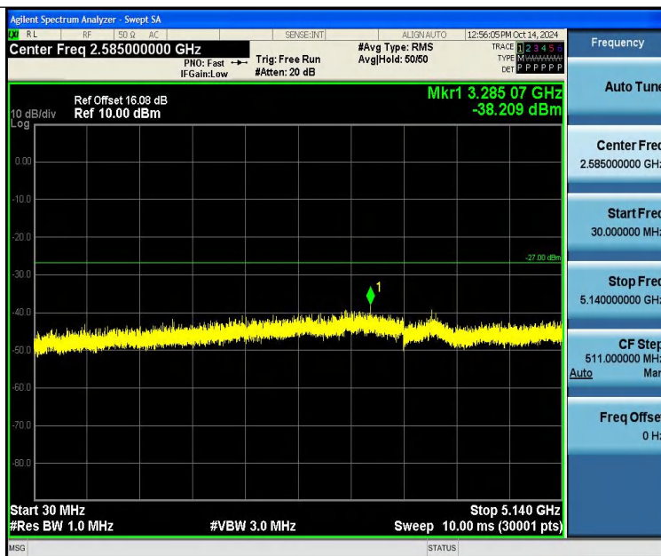
11N20SISO-Ant1-5240-30~5140-PASS
