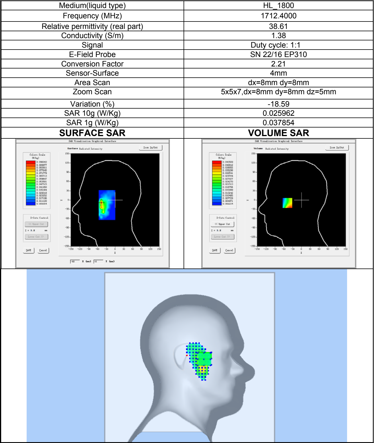
Plot 7: WCDMA BAND IV, Low channel (Left Head Cheek) Product Description: Smart Phone Test Date: 2023-04-18
