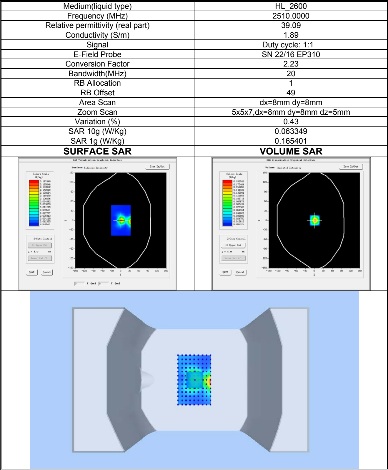
Plot 18: LTE BAND 7, Low channel (Body-worn/ Hotspot, Bottom Edge) Product Description: Smart Phone Test Date: 2023-04-10
