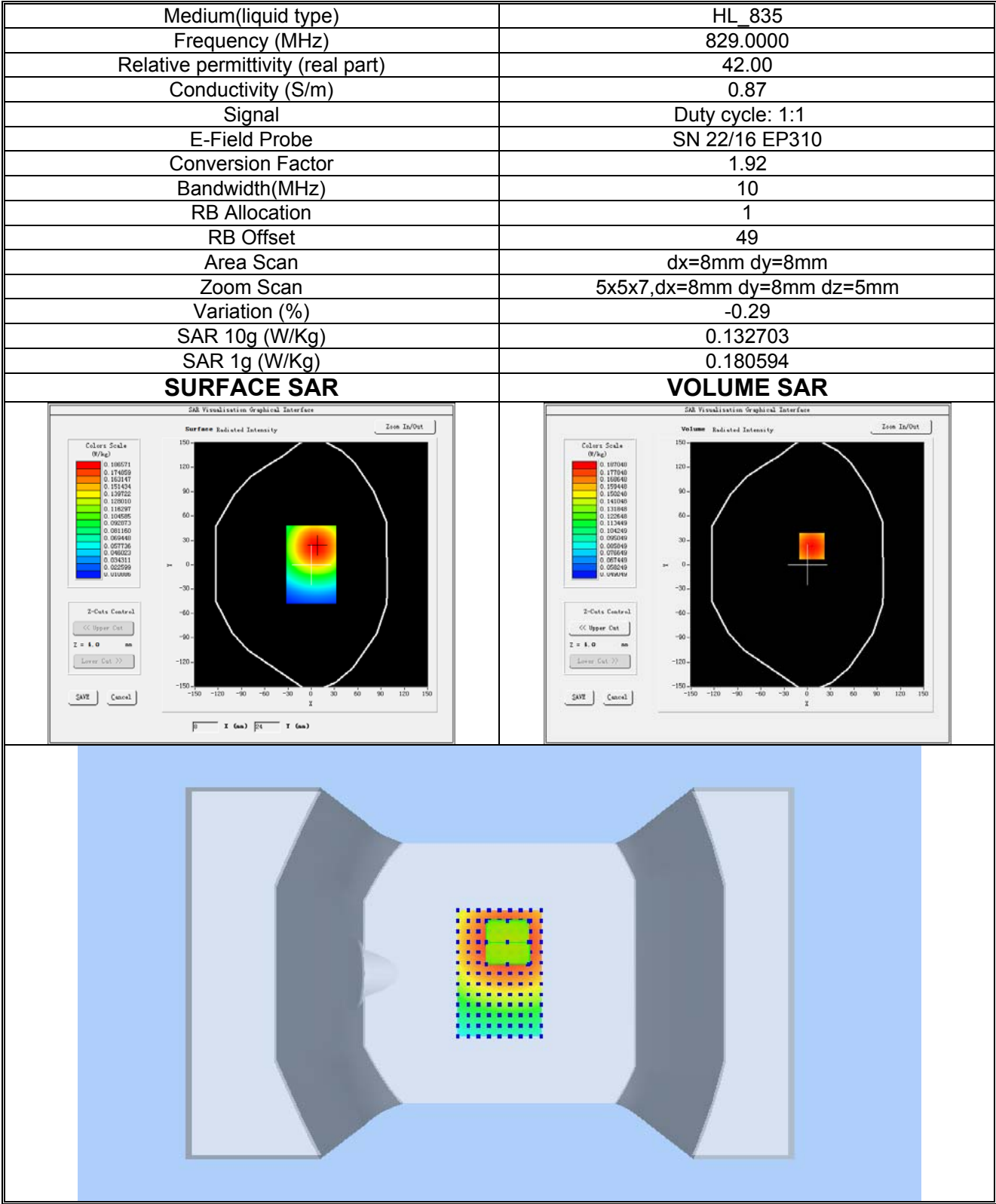
Plot 16: LTE BAND 5, Low channel (Body-worn/ Hotspot, Front Side) Product Description: Smart Phone Test Date: 2023-04-19
