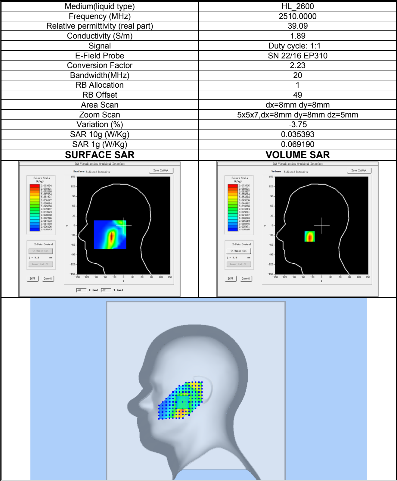
Plot 17:LTE BAND 7, Low channel (RightHead Cheek) Product Description: Smart Phone Test Date: 2023-04-16
