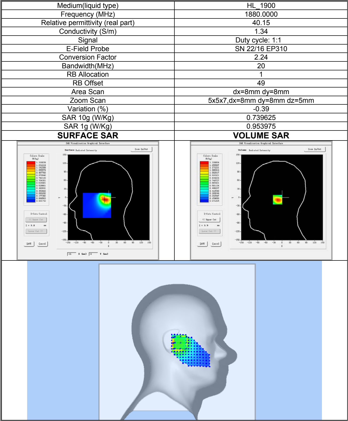
Plot 11:LTE BAND 2, Middle channel (Left Head Cheek) Product Description:Smart Phone Test Date: 2023-04-13
