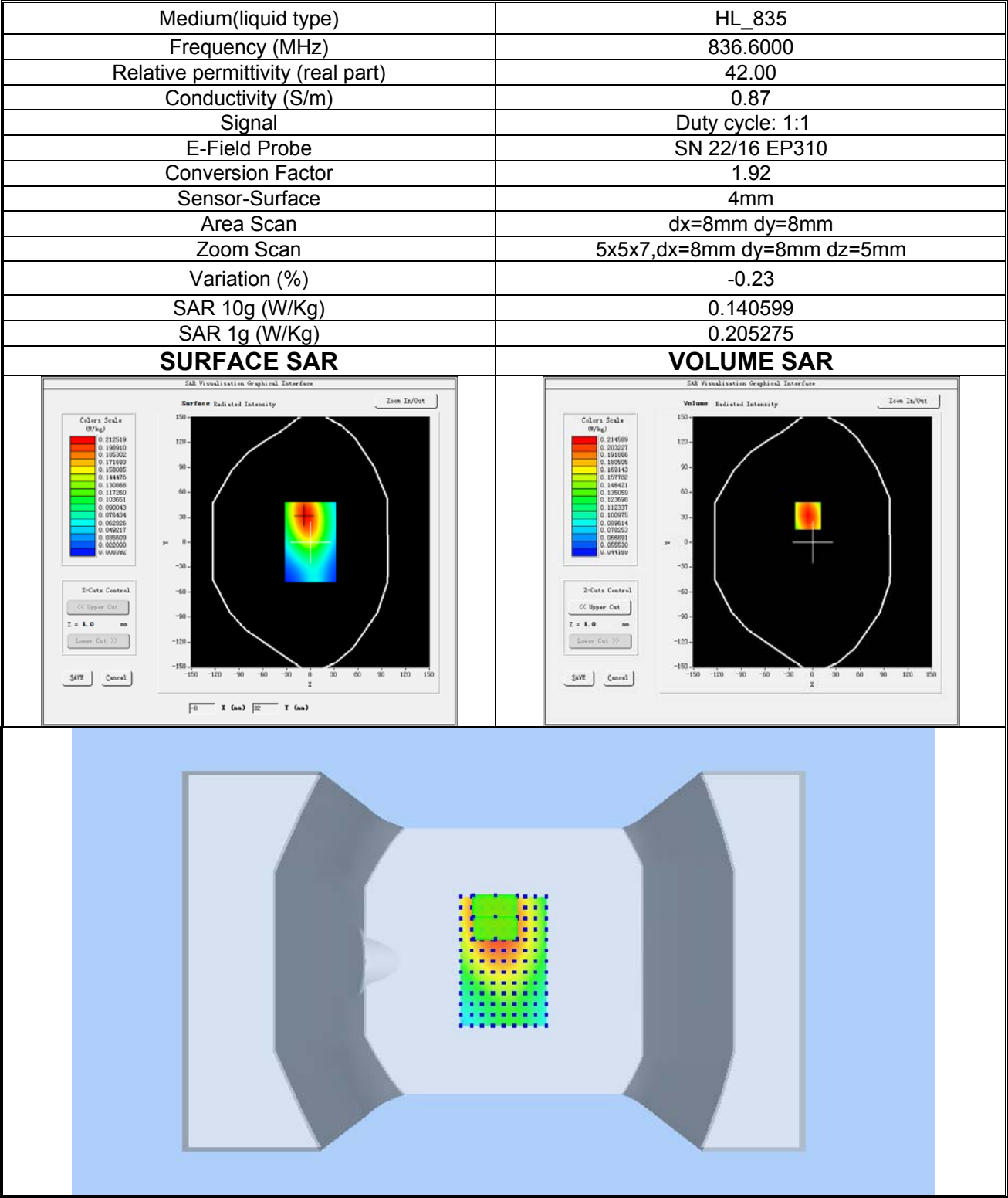
Plot 10: WCDMA BAND V, Middle channel (Body-worn/Hotspot, Right Edge) Product Description: Smart Phone Test Date: 2023-04-18
