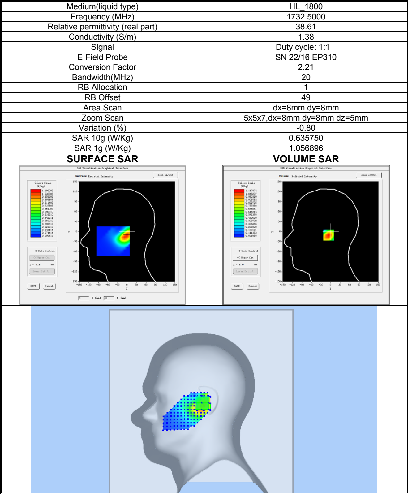
Plot 13:LTE BAND 4, Middle channel (Right Head Cheek) Product Description: Smart Phone Test Date: 2023-04-17
