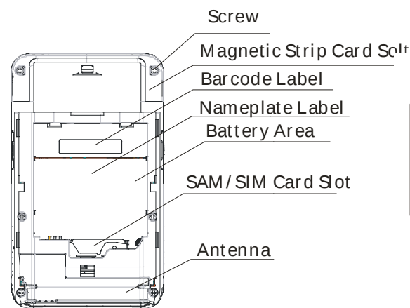
Back Layout
