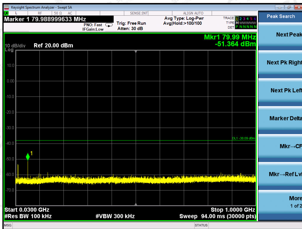
TEST PLOT OF OUT OF BAND EMISSIONS OF 802.11n40 FOR MODULATION IN LOW CHANNEL
