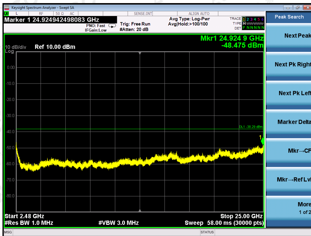
TEST PLOT OF OUT OF BAND EMISSIONS OF 802.11n40 FOR MODULATION IN HIGH CHANNEL
