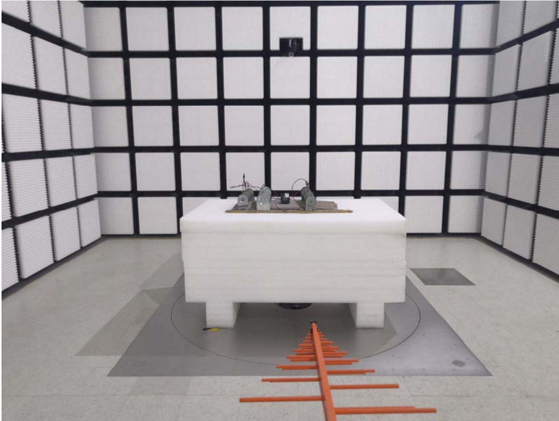
Radiated Emission Below 1GHz View- Model: M5-2C-120
