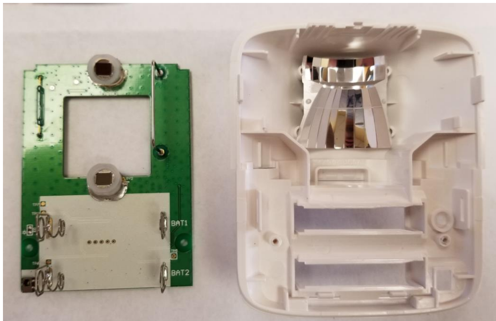
PCBA (side B)
