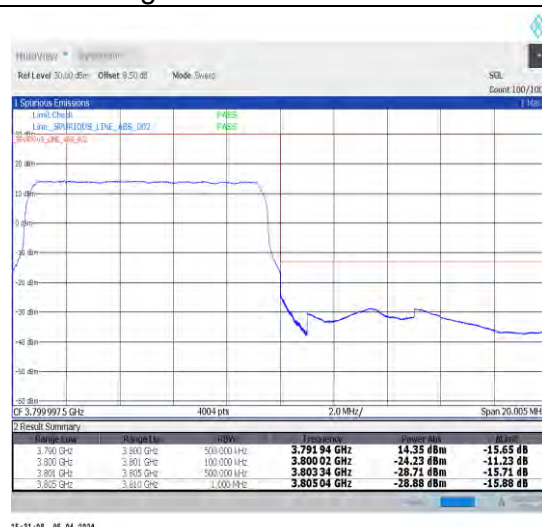
1-N78-3700-3800-N78-3700-380030-10-H-3-DFT-PI2BPSK-Outer_Full-24@0-Ant1-1--PASS-see graph
