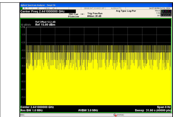
Number of Pulses in 31.6 seconds \pi/4 DQPSK 2-DH1
