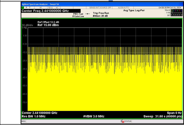
Number of Pulses in 31.6 seconds \pi/4 DQPSK 2-DH3
