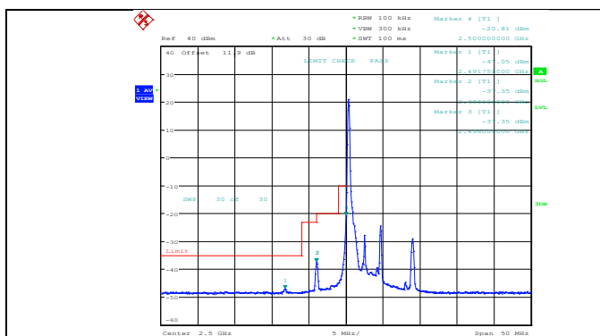
Band7-5MHz-QPSK-20775-1RB#0
