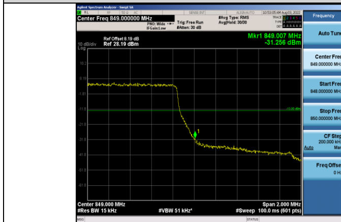
Band5-1.4MHz-64QAM-20643-6RB#0
