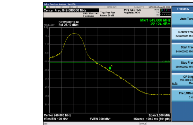
Band5-10MHz-64QAM-20600-1RB#49
