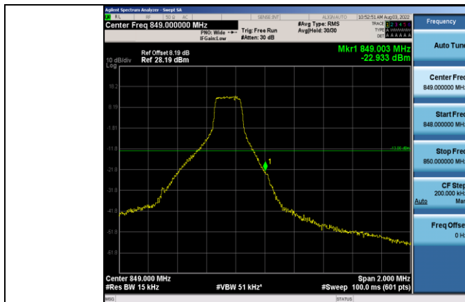
Band5-1.4MHz-64QAM-20643-1RB#5
