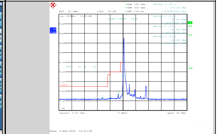
Band38-5MHz-64QAM-37775-1RB#0
