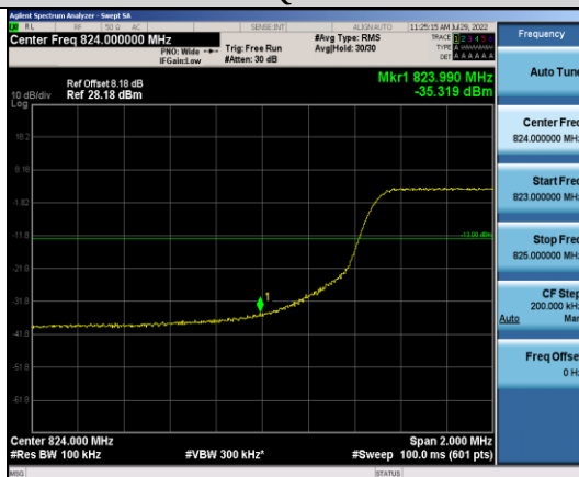
Band5-10MHz-16QAM-20450-50RB#0
