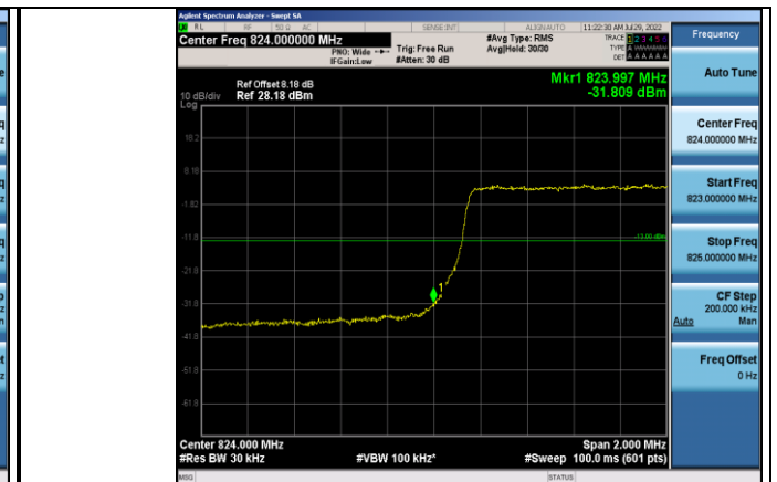
Band5-3MHz-QPSK-20415-15RB#0
