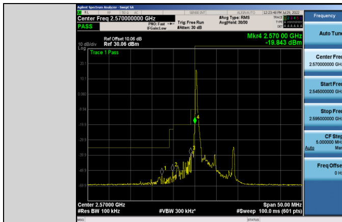
Band38-5MHz-16QAM-37775-1RB#0
