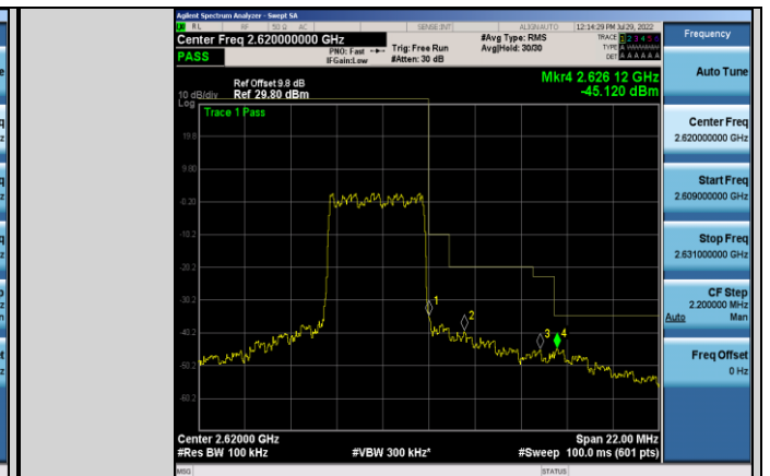
Band38-5MHz-16QAM-38225-25RB#0
