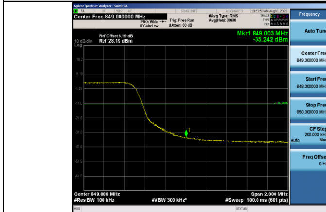
Band5-10MHz-64QAM-20600-50RB#0
