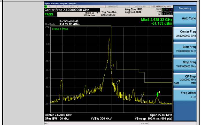
Band38-5MHz-QPSK-38225-1RB#24
