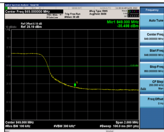
Band5-10MHz-16QAM-20600-50RB#0
