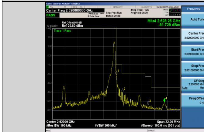
Band38-5MHz-16QAM-38225-1RB#24
