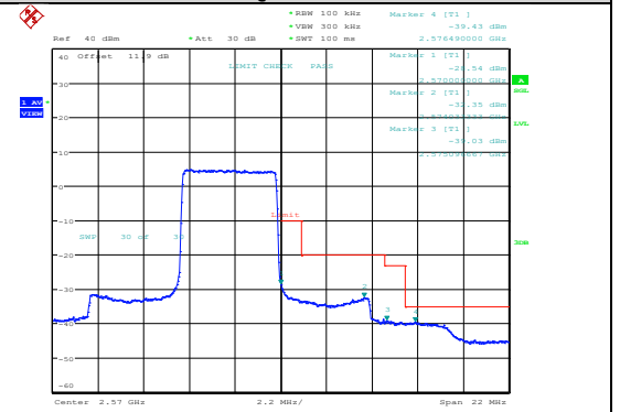
Band7-5MHz-QPSK-21425-1RB#24
