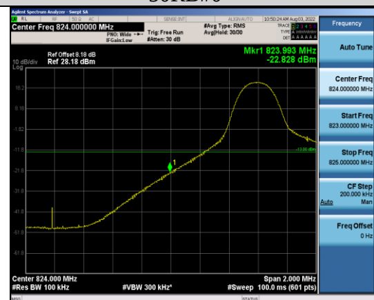
Band5-10MHz-64QAM-20450-1RB#0
