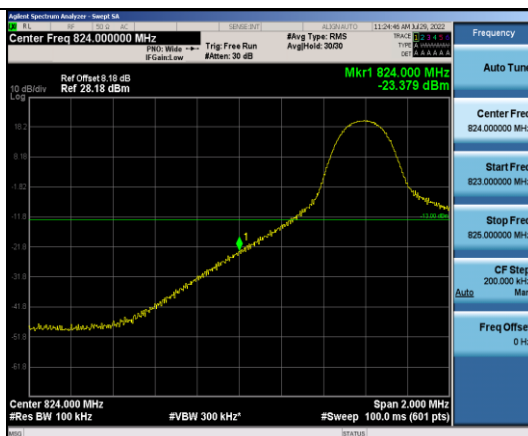
Band5-10MHz-16QAM-20450-1RB#0
