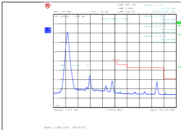
Band7-20MHz-64QAM-21350-1RB#0
