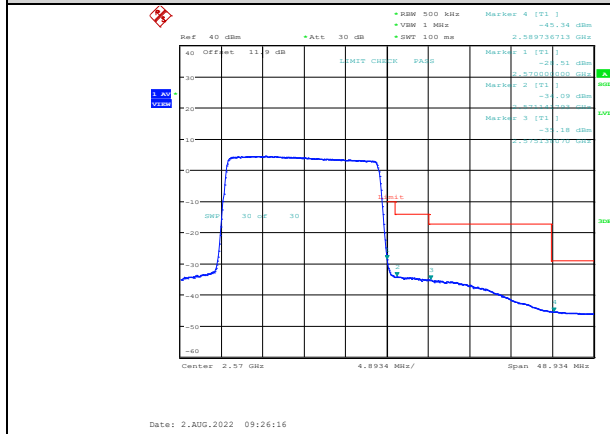
Band7-20MHz-64QAM-21350-100RB#0
