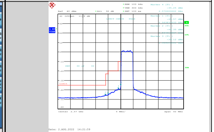
Band38-5MHz-64QAM-37775-25RB#0
