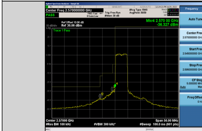
Band38-5MHz-16QAM-37775-25RB#0
