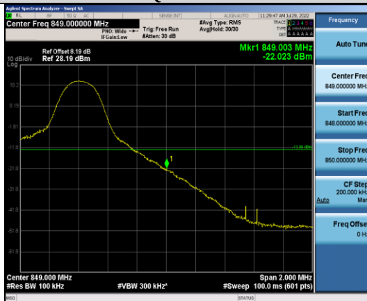
Band5-10MHz-16QAM-20600-1RB#49
