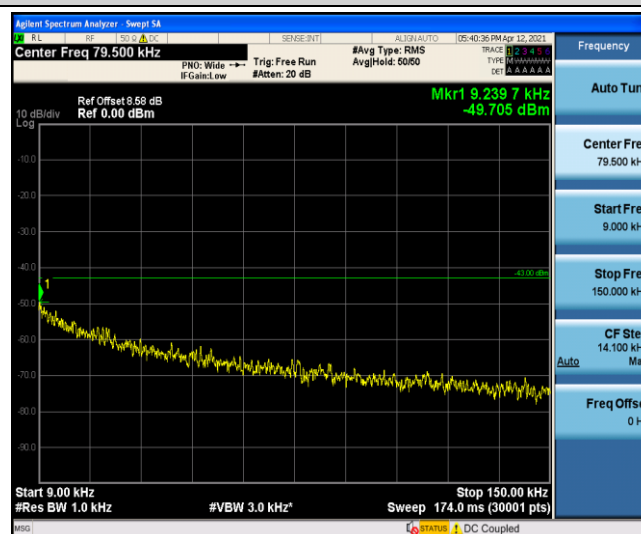
Band5-5MHz-QPSK-20625-1-0-High-0.009-0.15--49.71-PASS
