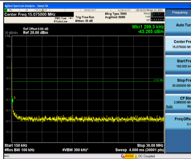
Band5-5MHz-QPSK-20425-1-0-Low-0.15-30--43.27-PASS
