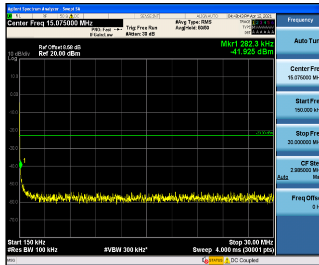
Band5-3MHz-16QAM-20415-1-0-Low-0.15-30--41.93-PASS
