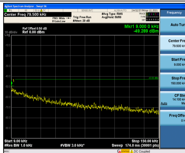
Band5-3MHz-16QAM-20525-1-0-Low-0.009-0.15--49.29-PASS
