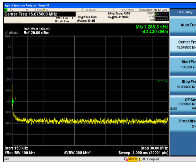
Band5-3MHz-16QAM-20635-1-0-High-0.15-30--42.43-PASS
