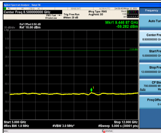
Band5-3MHz-16QAM-20635-1-0-High-5000-12000--59.28-PASS
