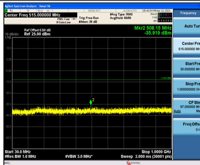
Band5-5MHz-QPSK-20625-1-0-High-30-1000--35.92-PASS
