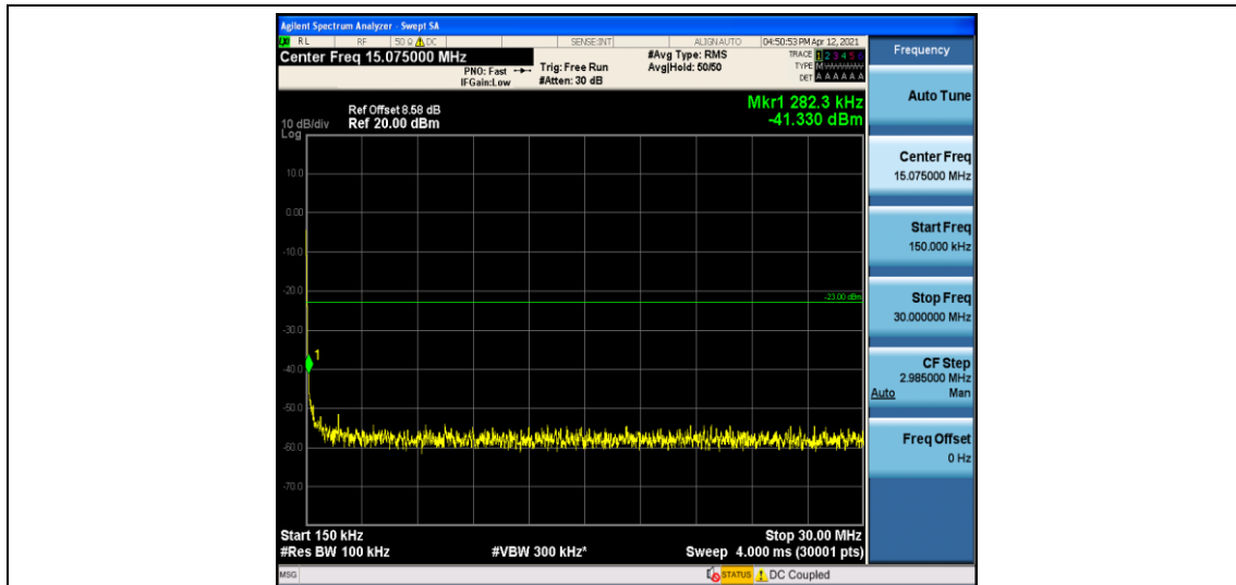
Band5-3MHz-QPSK-20525-1-0-Low-0.15-30--41.33-PASS
