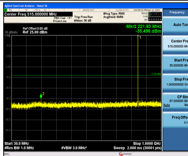
Band5-3MHz-16QAM-20635-1-0-High-30-1000--35.5-PASS
