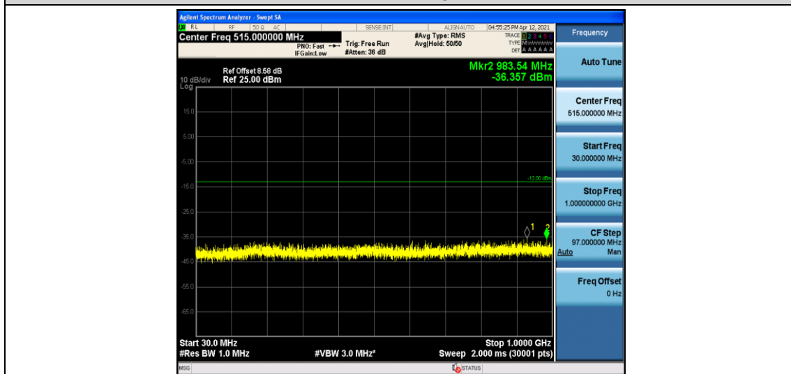
Band5-3MHz-QPSK-20635-1-0-High-30-1000--36.36-PASS
