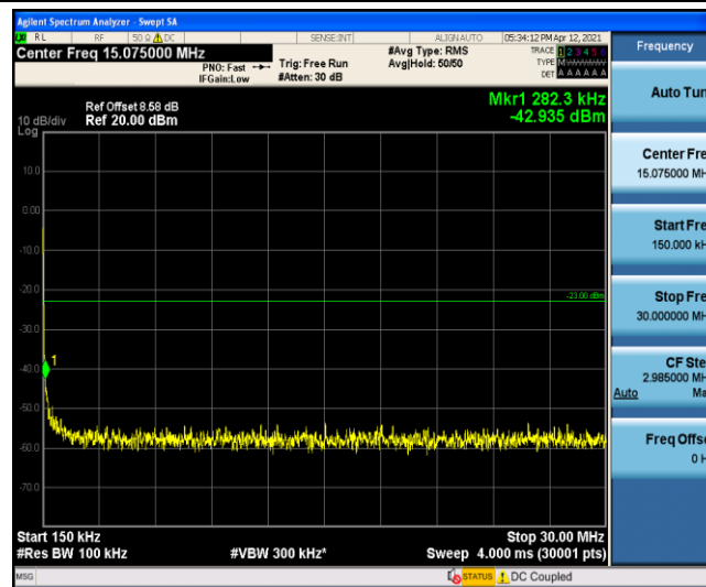
Band5-5MHz-16QAM-20425-1-0-Low-0.15-30--42.94-PASS
