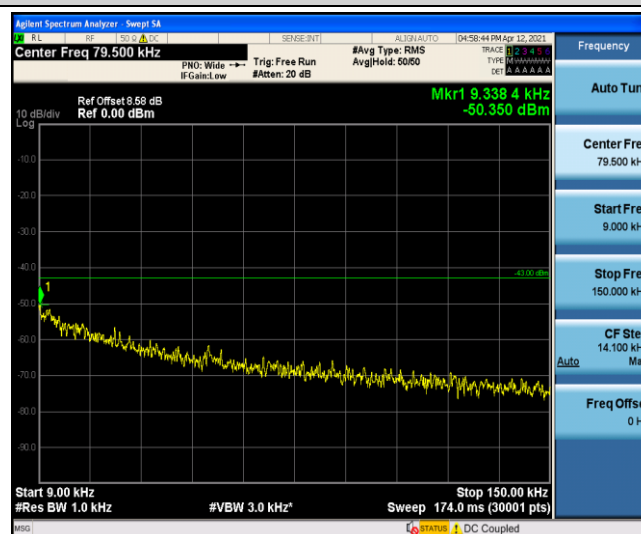
Band5-3MHz-16QAM-20635-1-0-High-0.009-0.15--50.35-PASS
