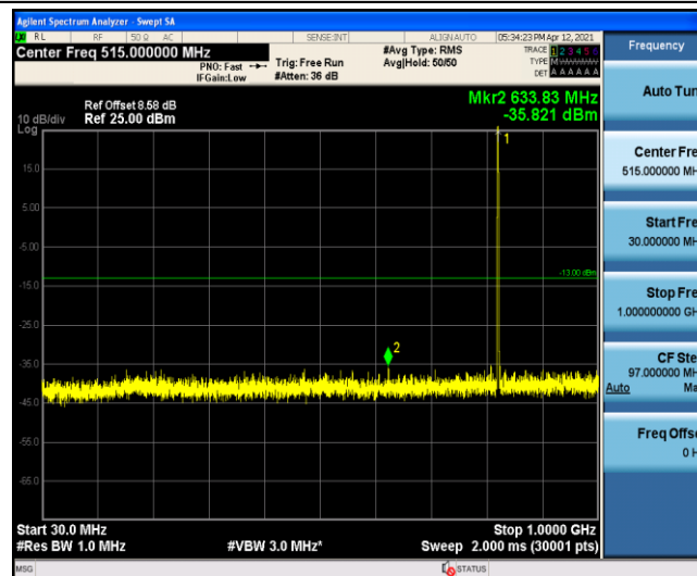
Band5-5MHz-16QAM-20425-1-0-Low-30-1000--35.82-PASS
