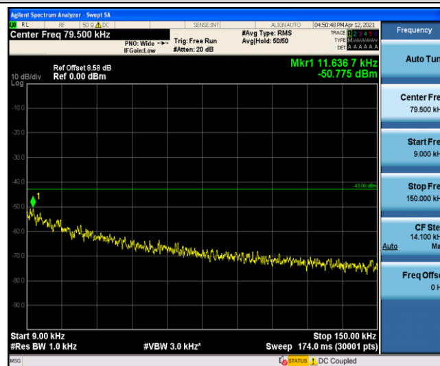
Band5-3MHz-QPSK-20525-1-0-Low-0.009-0.15--50.78-PASS
