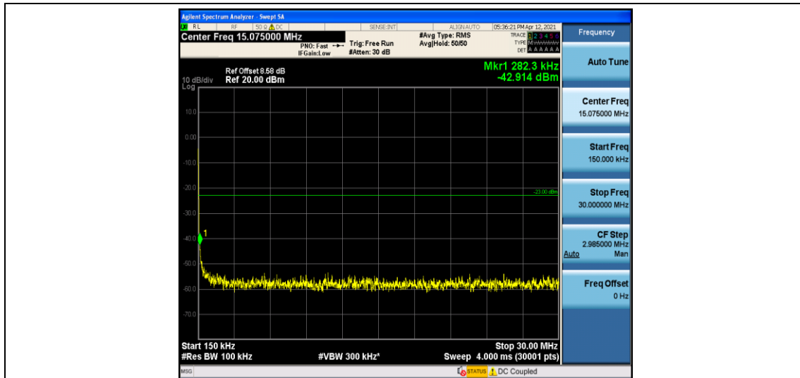
Band5-5MHz-QPSK-20525-1-0-Low-0.15-30--42.91-PASS
