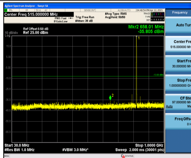
Band5-3MHz-16QAM-20415-1-0-Low-30-1000--35.81-PASS
