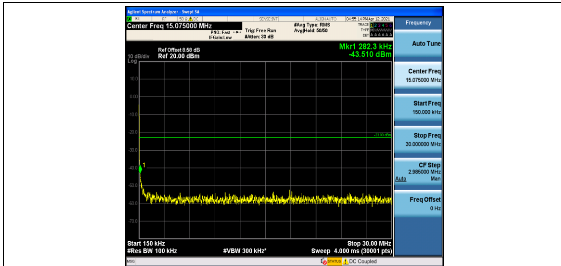
Band5-3MHz-QPSK-20635-1-0-High-0.15-30--43.51-PASS
