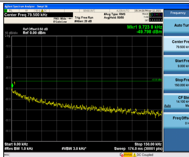
Band5-5MHz-16QAM-20425-1-0-Low-0.009-0.15--49.8-PASS
