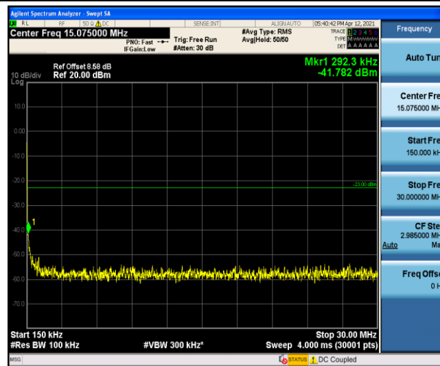
Band5-5MHz-QPSK-20625-1-0-High-0.15-30--41.78-PASS
