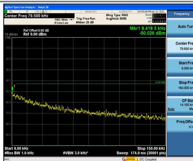
Band5-3MHz-QPSK-20635-1-0-High-0.009-0.15--50.03-PASS
