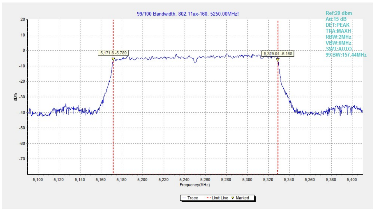
Fig.93 99% Occupied bandwidth (802.11ax-HE160, 5250MHz)
