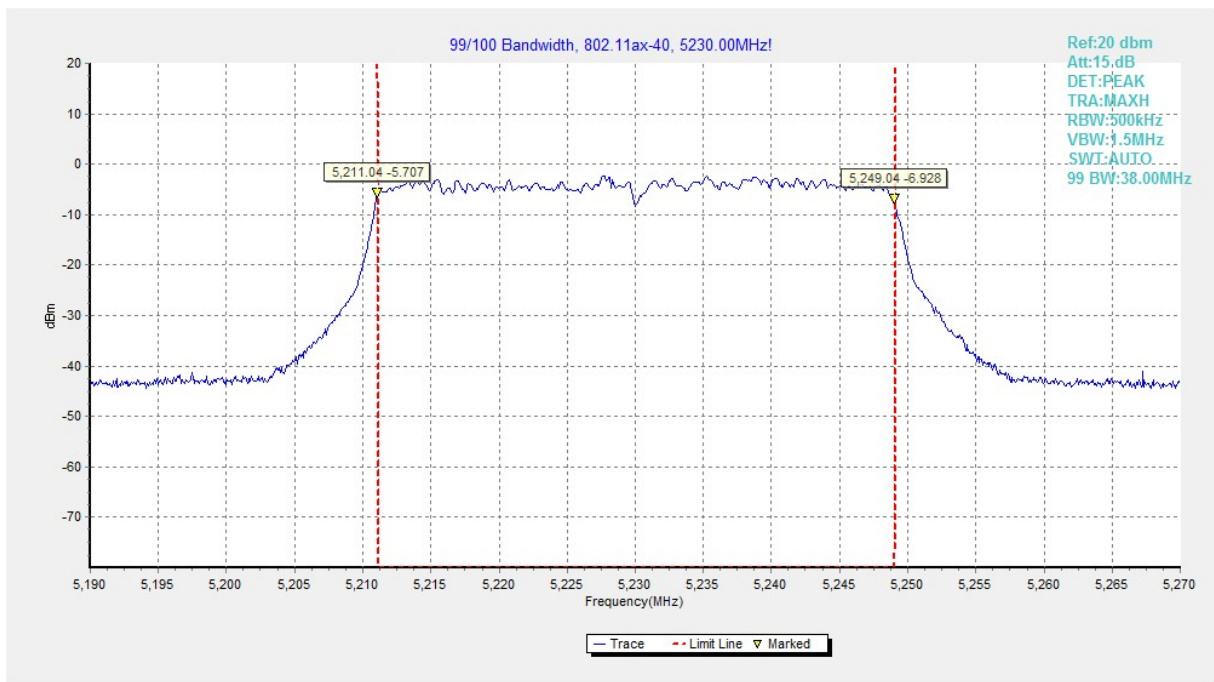
Fig.91 99% Occupied bandwidth (802.11ax-HE40, 5230MHz)
