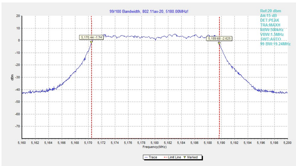
Fig.87 99% Occupied bandwidth (802.11ax-HE20, 5180MHz)
