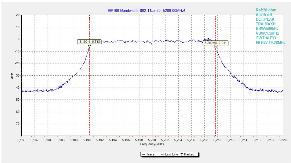
Fig.88 99% Occupied bandwidth (802.11ax-HE20, 5200MHz)
