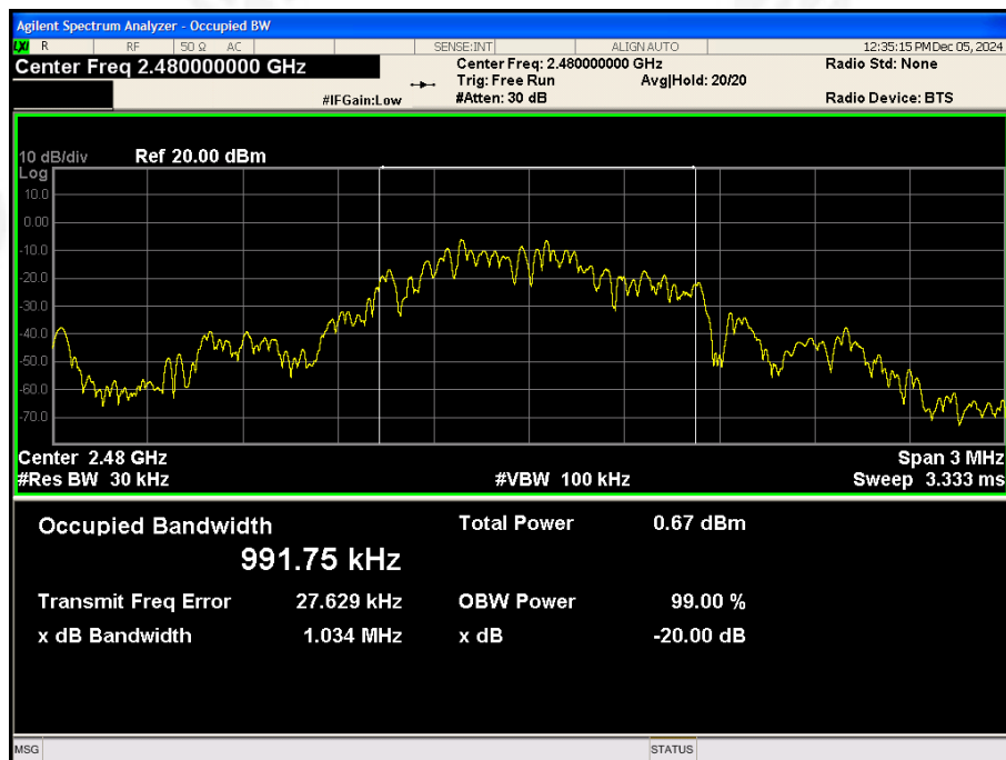
CH39: 2480MHz
