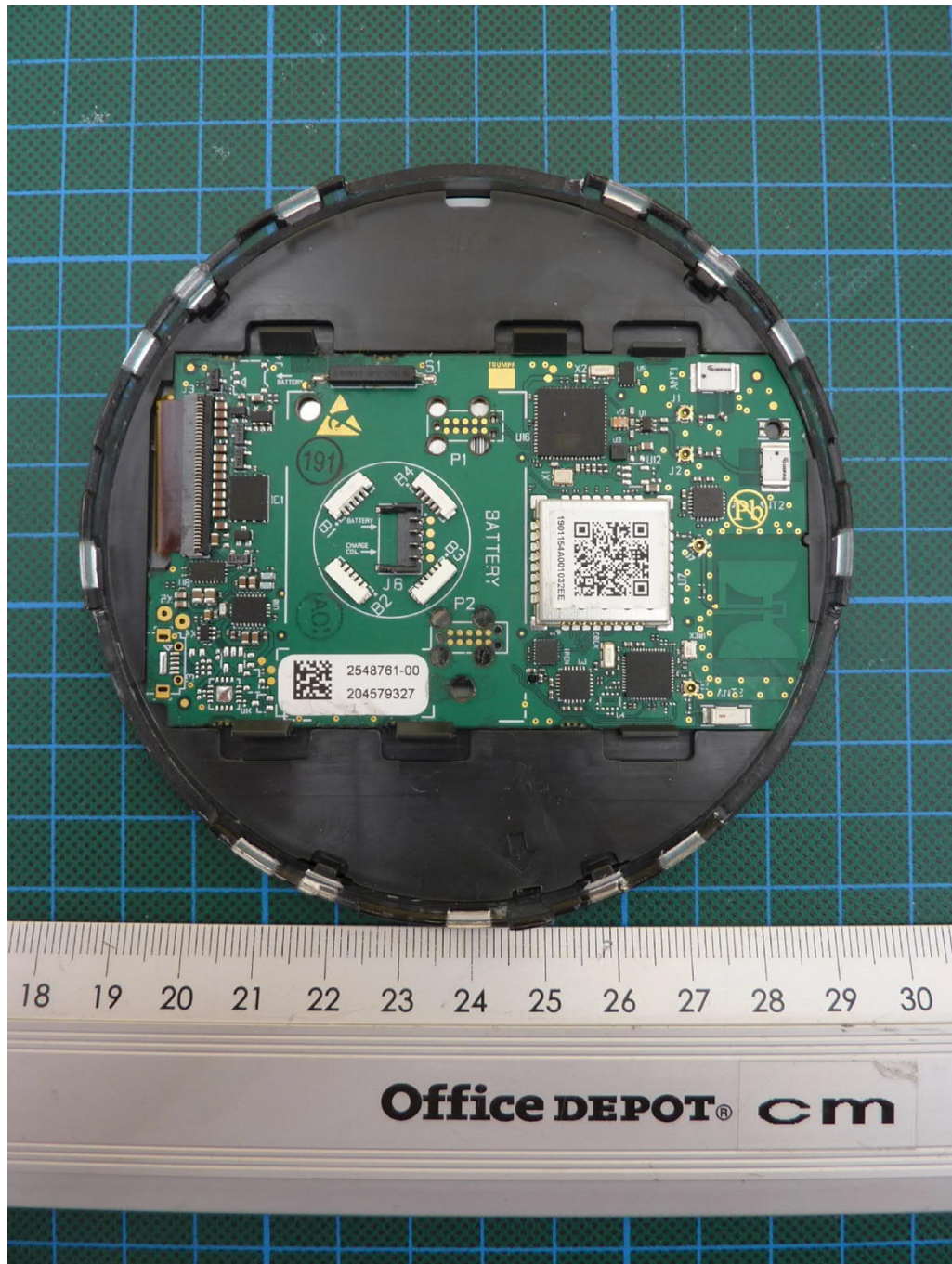
Hhousing, top part with PCB
