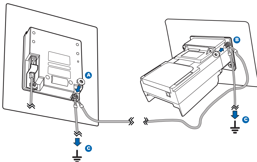
Figure 11 Grounding the UX300 and PIN Pad Units
