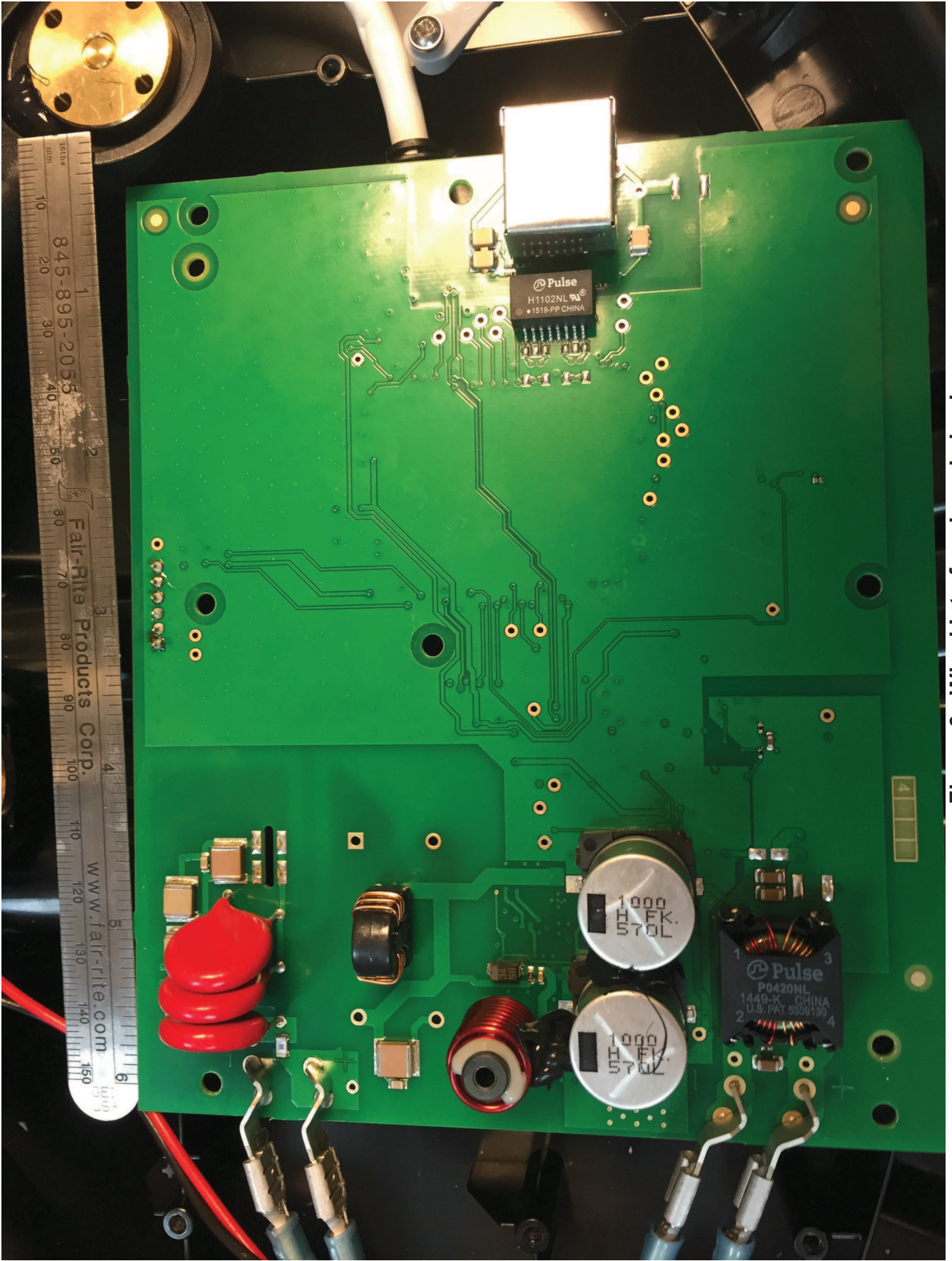
Figure 6 - Wired Interface board - back
