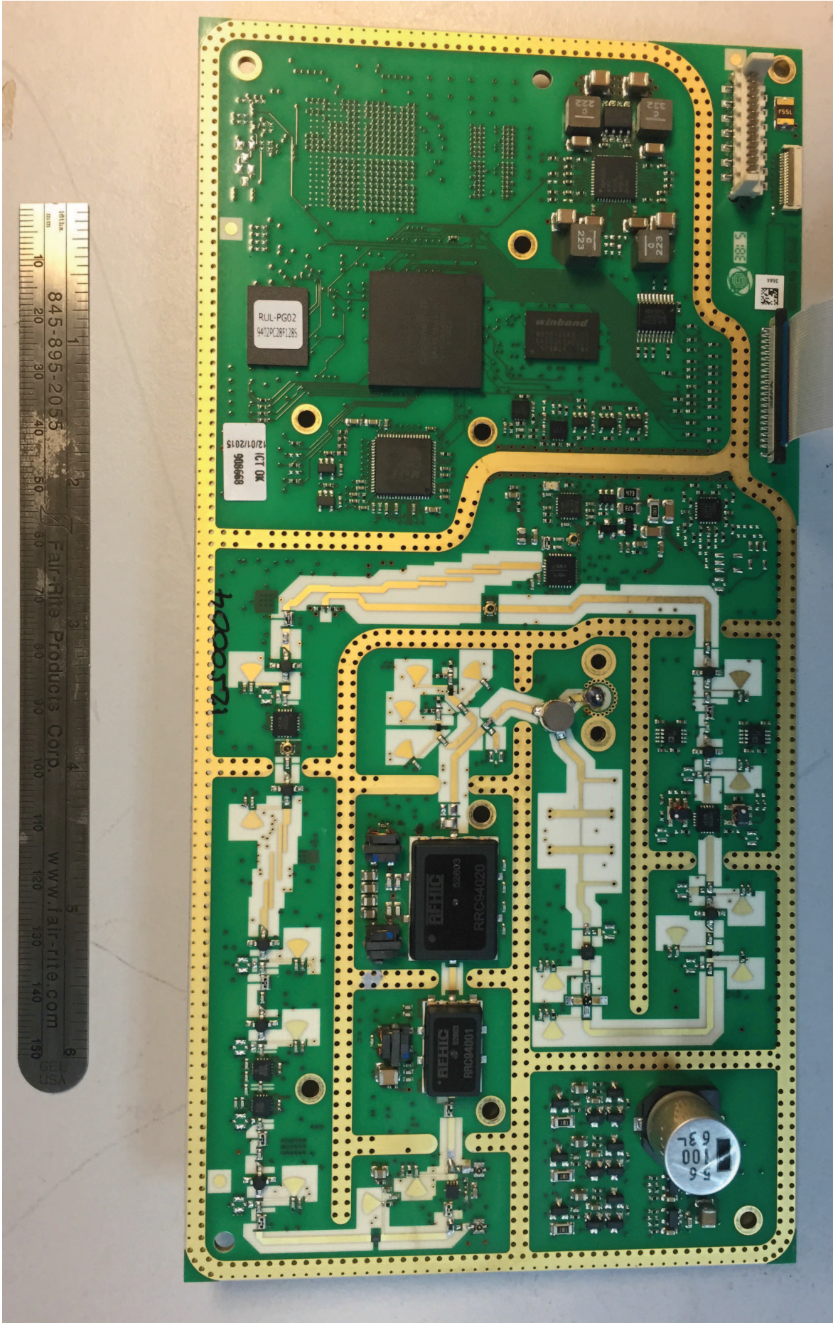
Figure 7 – RF board – Top
