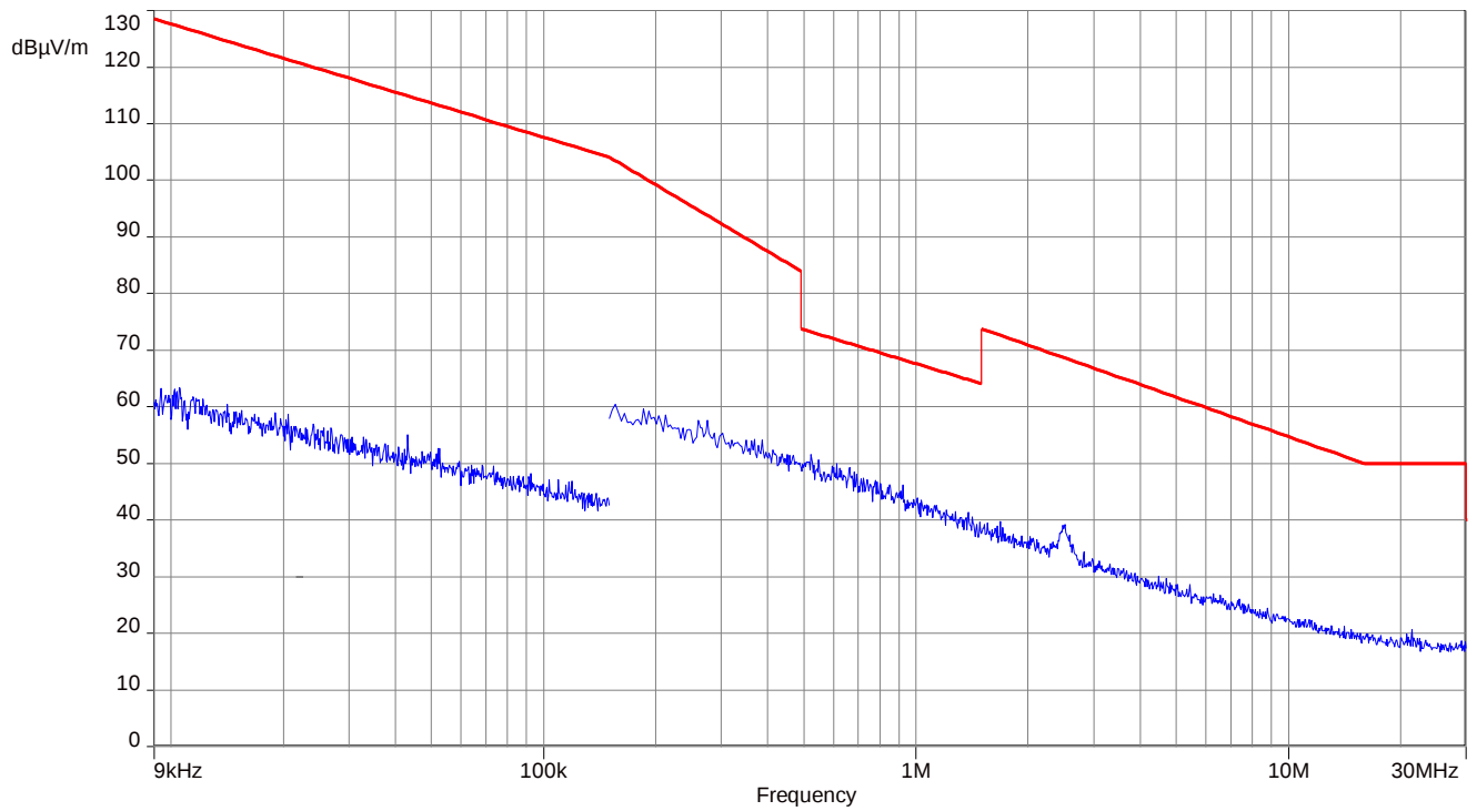
Plot 4: 9 kHz to 30 MHz, UWB test mode
