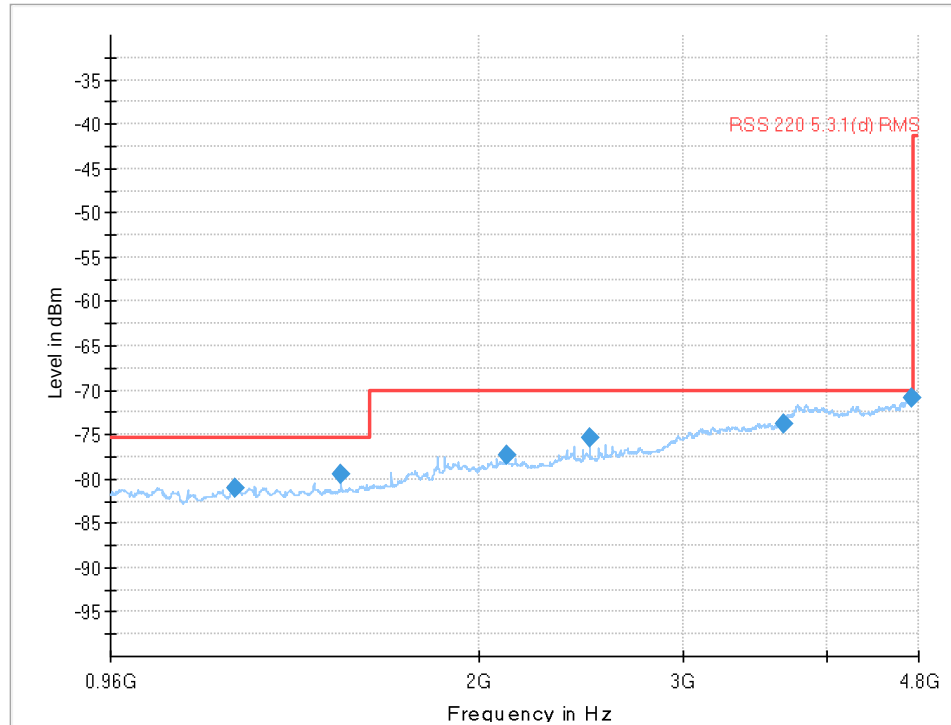
Plot 7: 960 MHz to 4.8 GHz (Limit acc. to RSS-220 5.3.1(d)), UWB test mode
