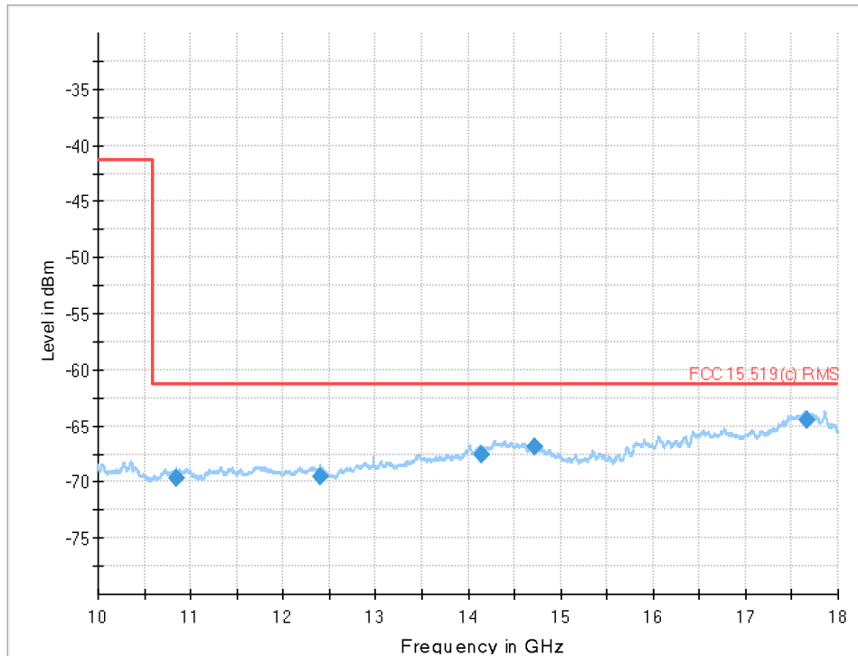
Plot 9: 10 GHz to 18 GHz, UWB test mode
