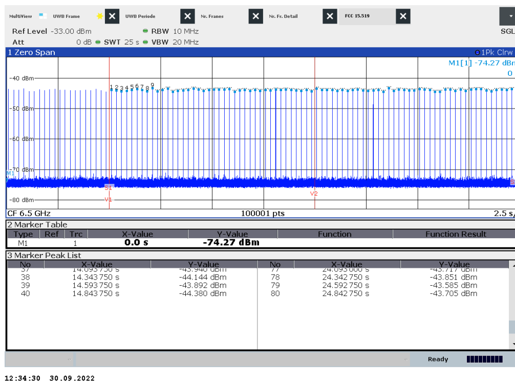
Plot 16: Emissions of the EUT (normal mode, placed on inductive charger), switching off the associated UWB receiver
