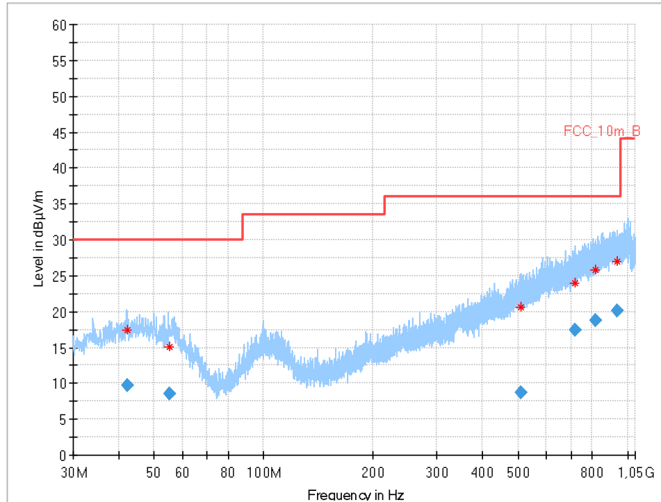
Plot 5: 30 MHz to 1 GHz, UWB test mode
