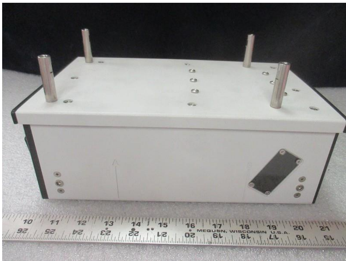
EUT_ Left Side View& Dimension
