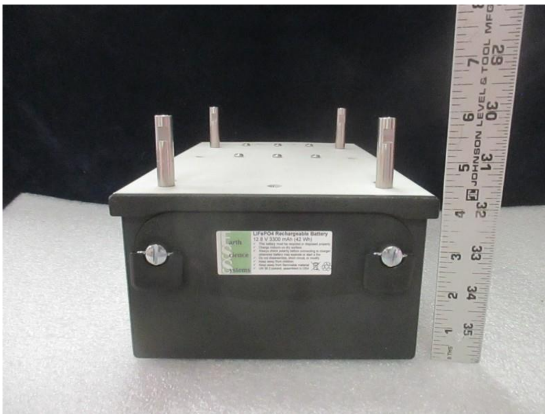
EUT_ Rear View & Dimension
