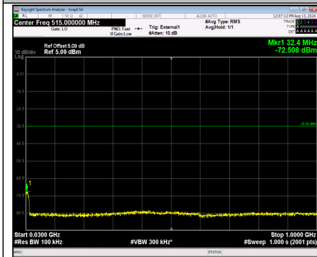
41-41-20MHz-20MHz-16QAM-16QAM-40641-40839-100 RB#0-100RB#0-30~1000MHz-PASS
