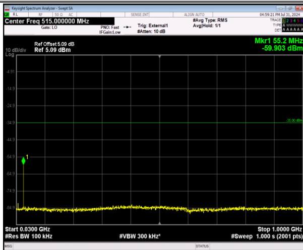
41-41-20MHz-20MHz-64QAM-64QAM-40942-41140-1R B#0-ORB#0-30~1000MHz-PASS
