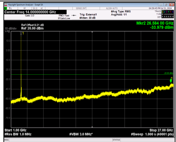
41-41-20MHz-20MHz-64QAM-64QAM-40942-41140-1RB #0-ORB#0-1000~27000MHz-PASS
