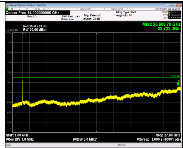
41-41-20MHz-20MHz-16QAM-16QAM-40641-40839-1RB #99-ORB#0-1000~27000MHz-PASS
