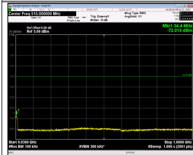
41-41-20MHz-20MHz-64QAM-64QAM-40641-40839-100 RB#0-100RB#0-30~1000MHz-PASS
