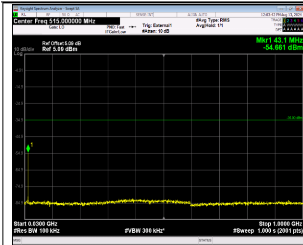
41-41-20MHz-20MHz-16QAM-16QAM-40641-40839-1R B#99-ORB#0-30~1000MHz-PASS
