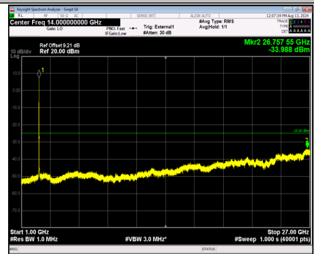
41-41-20MHz-20MHz-16QAM-16QAM-40641-40839-100 RB#0-100RB#0-1000~27000MHz-PASS
