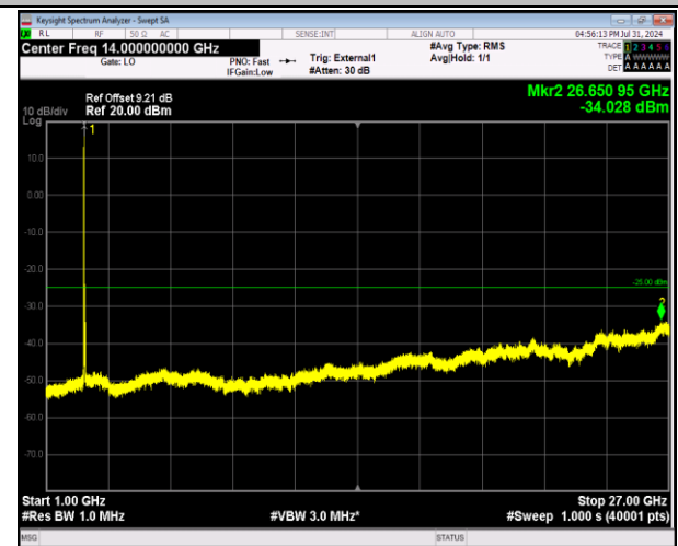
41-41-20MHz-20MHz-64QAM-64QAM-40641-40839-1RB #0-ORB#0-1000~27000MHz-PASS
