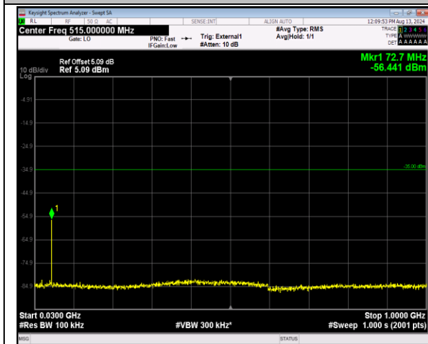
41-41-20MHz-20MHz-QPSK-QPSK-40942-41140-1RB#9 9-0RB#0-30~1000MHz-PASS
