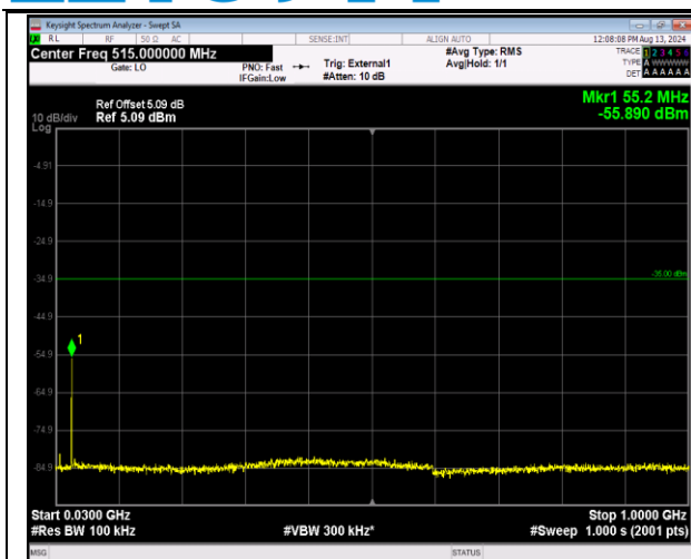
41-41-20MHz-20MHz-QPSK-QPSK-40942-41140-1RB#0 -0RB#0-30~1000MHz-PASS
