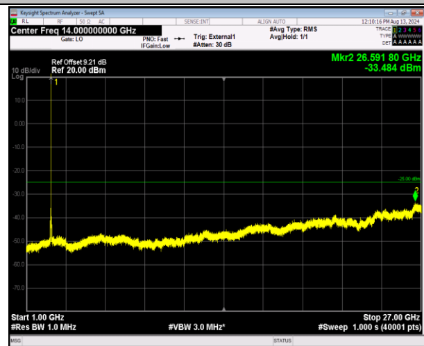
41-41-20MHz-20MHz-QPSK-QPSK-40942-41140-1RB#9 9-0RB#0-1000~27000MHz-PASS
