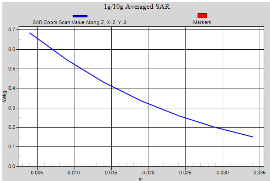
Figure 13 Left Hand Touch Cheek GSM 850 Channel 190
