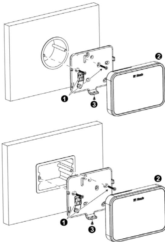
Figure 4b – Wall Mounting with External Electrical Connector
