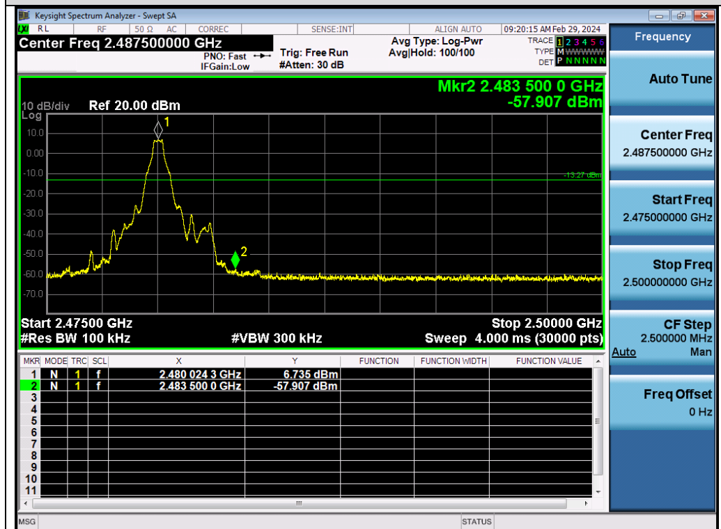
Test Graph BR ANT1 2480 1Mbps Higher Band Edge Emissions
